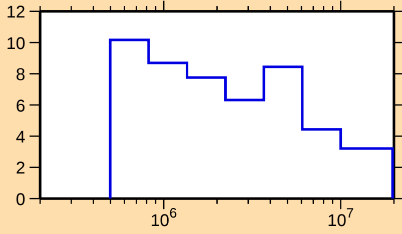
\Delta\sigma/\sigma vs. E for ^{144}\text{Gd}(n,\text{tot.})
