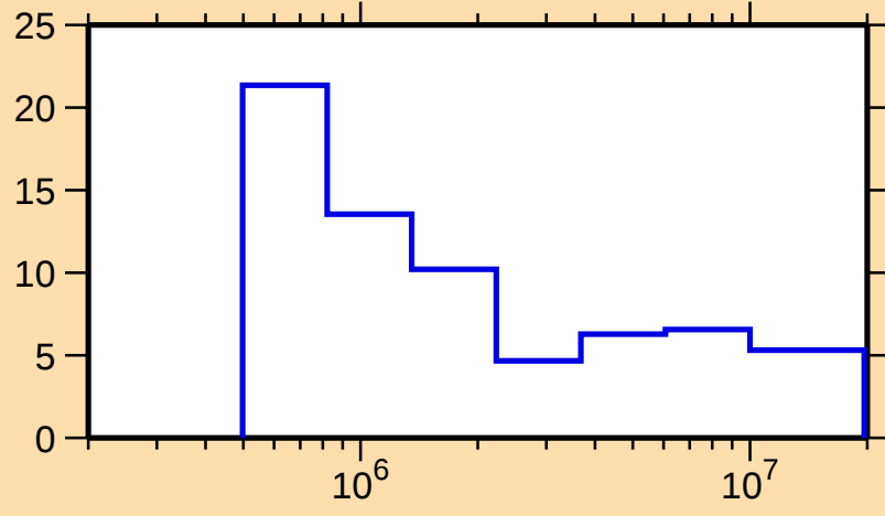
\Delta\sigma/\sigma vs. E for ^{144}\text{Gd}(n,\text{nonel.})
