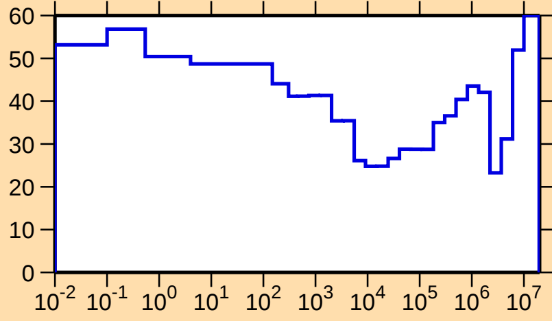
\Delta\sigma/\sigma vs. E for ^{144}\text{Gd}(n,p)
