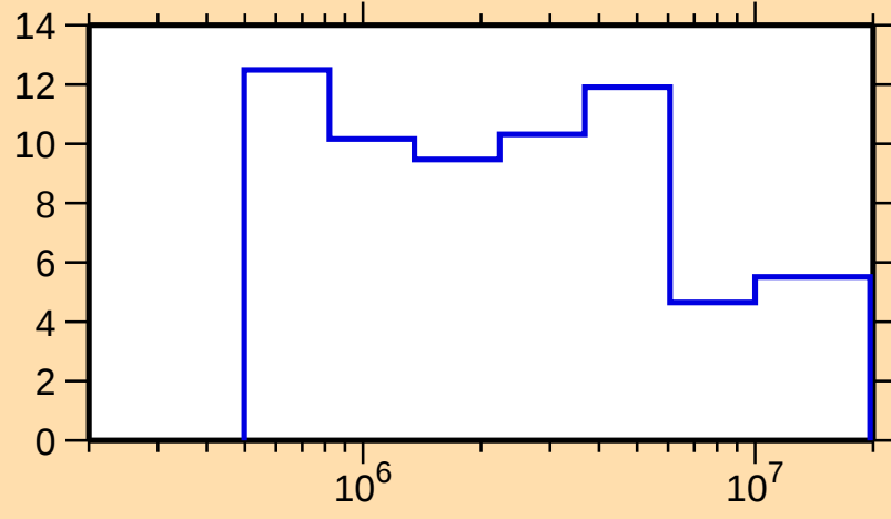
\Delta\sigma/\sigma vs. E for ^{144}\text{Gd}(n,\text{el.})
