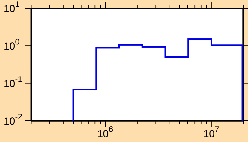
\sigma vs. E for ^{144}\text{Gd}(n,\text{inel.})
