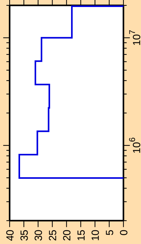
\Delta\sigma/\sigma vs. E for ^{144}\text{Gd}(n,n_1)
