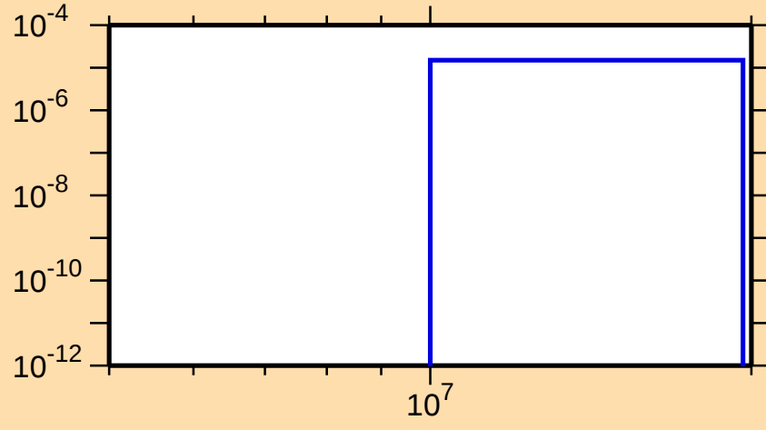
\sigma vs. E for ^{144}\text{Gd}(n,t)
