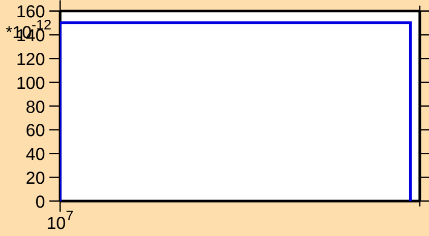
\sigma vs. E for ^{144}\text{Gd}(n,\text{nd})
