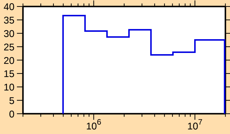
\Delta\sigma/\sigma vs. E for ^{144}\text{Gd}(n,\text{inel.})
