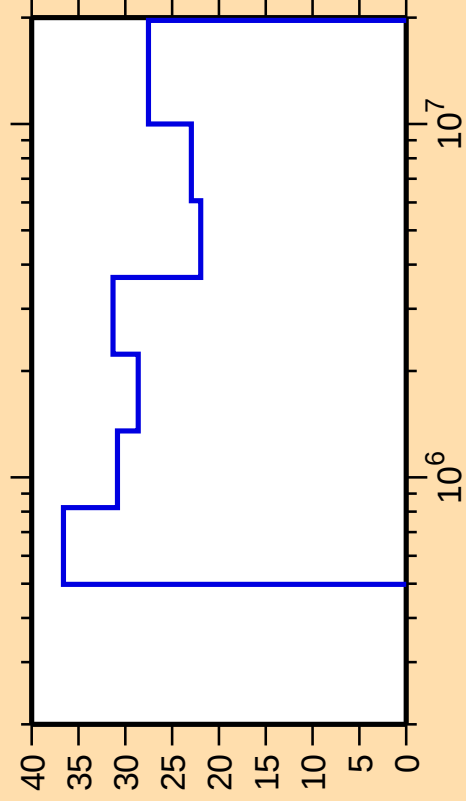
\Delta\sigma/\sigma vs. E for ^{144}\text{Gd}(n,\text{inel.})
