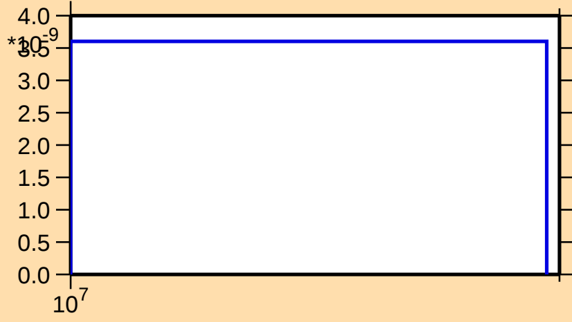
\sigma vs. E for ^{144}\text{Gd}(n,2np)
