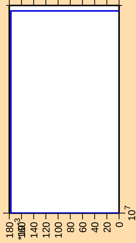
\Delta\sigma/\sigma vs. E for ^{144}\text{Gd}(\text{mt } 34)
