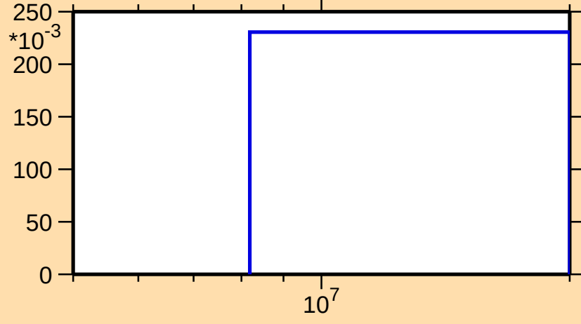
\sigma vs. E for ^{144}\text{Gd}(n,2n)
