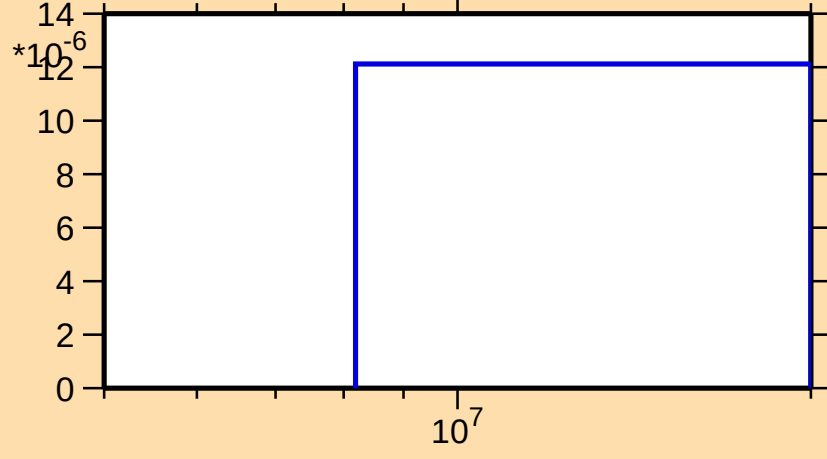
\sigma vs. E for ^{144}\text{Gd}(n,t)
