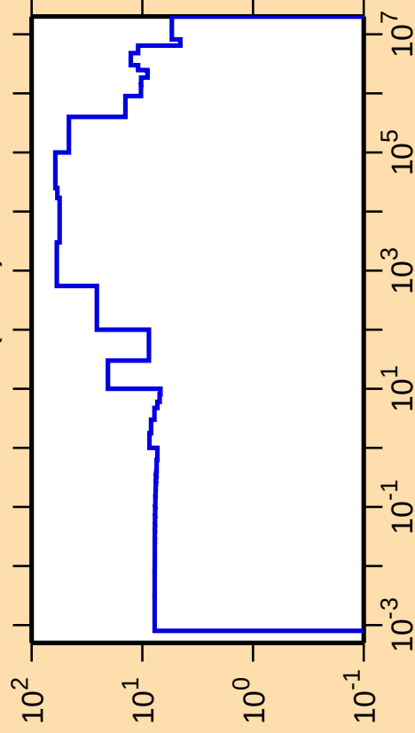
\Delta\sigma/\sigma vs. E for ^{144}\text{Gd}(n,\text{el.})
