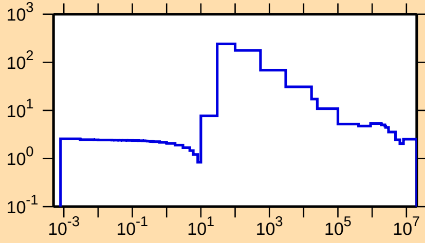
\sigma vs. E for ^{144}\text{Gd}(n,\text{el.})
