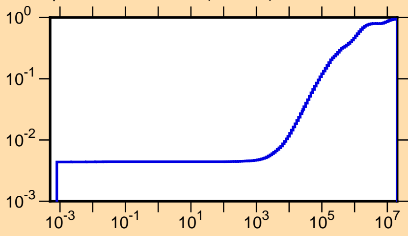
\mu vs. E for ^{154}\text{Gd}(\text{mt251})
