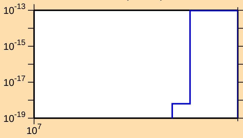
\sigma vs. E for ^{154}\text{Gd}(n,3n\alpha)
