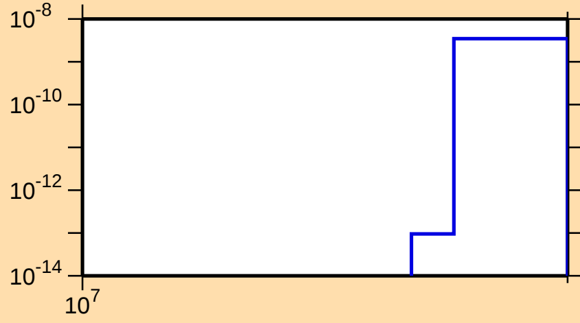
\sigma vs. E for ^{154}\text{Gd}(n,\text{nt})
