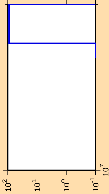
\Delta\sigma/\sigma vs. E for ^{154}\text{Gd}(n,\text{nt})
