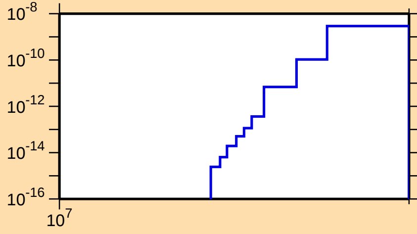
\sigma vs. E for ^{154}\text{Gd}(n,\text{He3})
