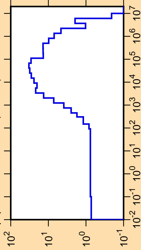
\Delta\mu/\mu vs. E for ^{154}\text{Gd}(\text{mt251})
