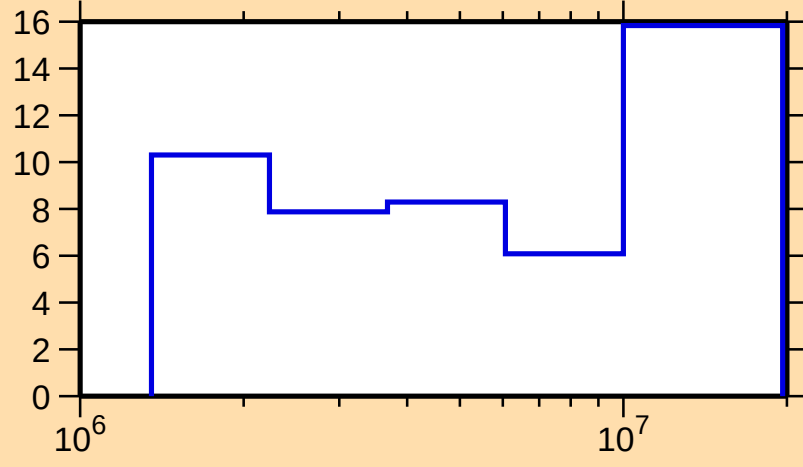
\Delta\sigma/\sigma vs. E for ^{154}\text{Gd}(n,n\text{cont.})
