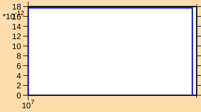
\sigma vs. E for ^{154}\text{Gd}(n,2np)
