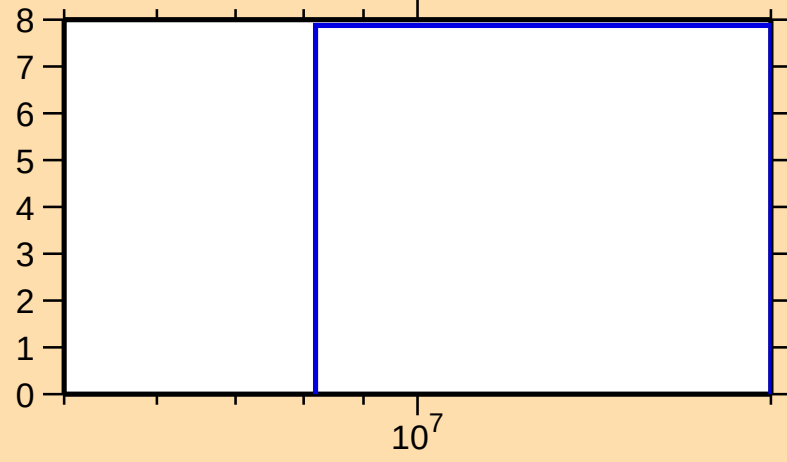
\Delta\sigma/\sigma vs. E for ^{154}\text{Gd}(n,2n)
