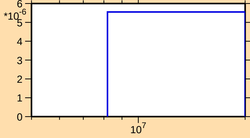
\sigma vs. E for ^{154}\text{Gd}(n,t)
