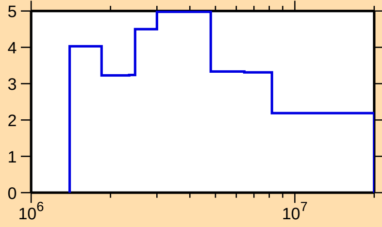
\Delta\sigma/\sigma vs. E for ^{154}\text{Gd}(n,n\text{onel.})
