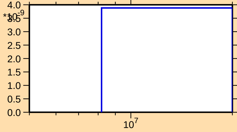
\sigma vs. E for ^{154}\text{Gd}(n,2n\alpha)
