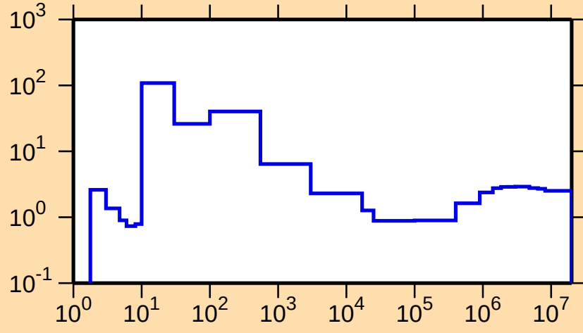
\sigma vs. E for ^{154}\text{Gd}(n,\text{nonel.})
