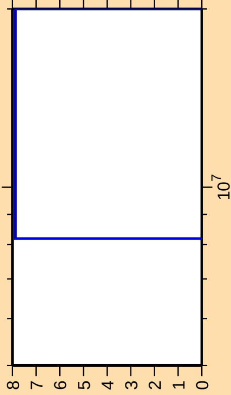
\Delta\sigma/\sigma vs. E for ^{154}\text{Gd}(n,2n)
