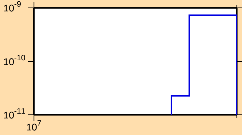
\sigma vs. E for ^{157}\text{Gd}(n,\text{He3})
