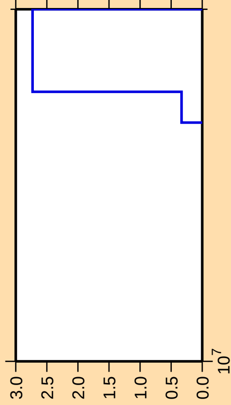
\Delta\sigma/\sigma vs. E for ^{157}\text{Gd}(n,p\alpha)
