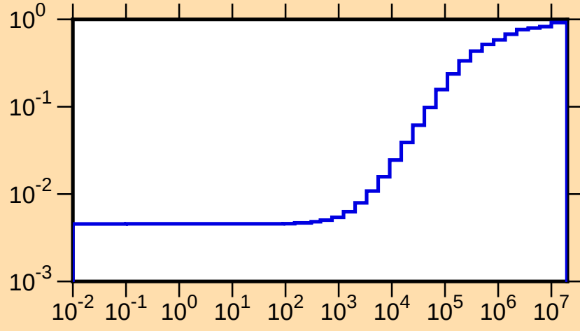
\mu vs. E for ^{157}\text{Gd}(\text{mt251})
