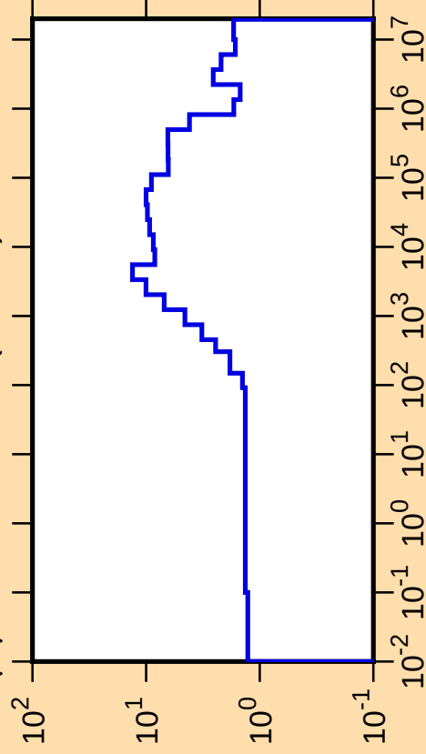
\Delta\mu/\mu vs. E for ^{157}\text{Gd}(\text{mt251})
