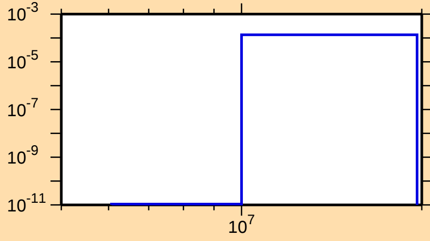
\sigma vs. E for ^{157}\text{Gd}(n,d)
