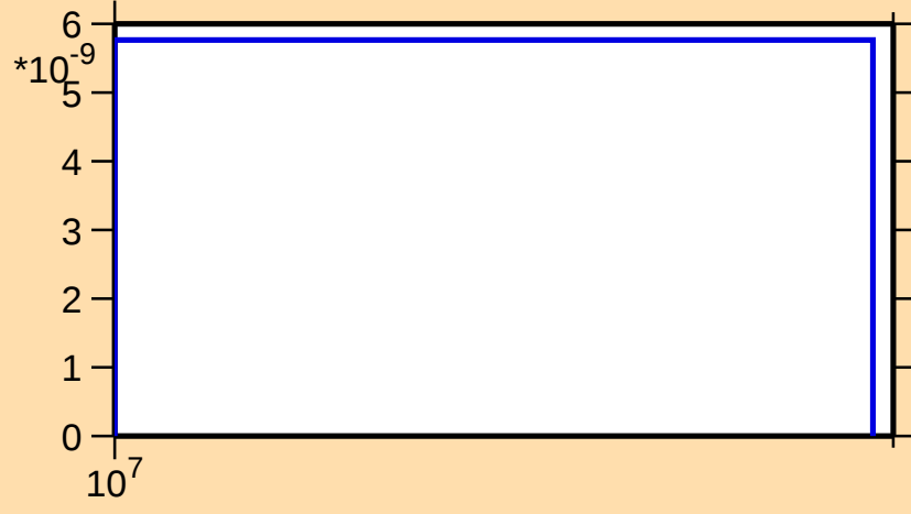
\sigma vs. E for ^{157}\text{Gd}(n,\text{nd})
