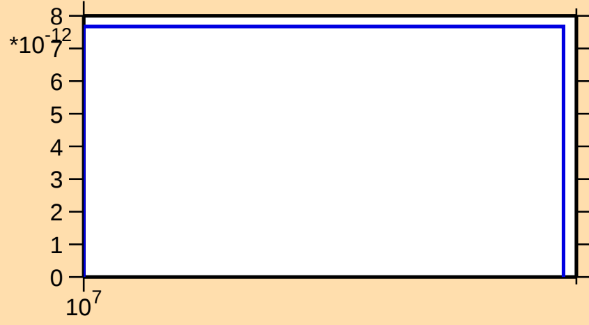
\sigma vs. E for ^{157}\text{Gd}(n,\text{He3})
