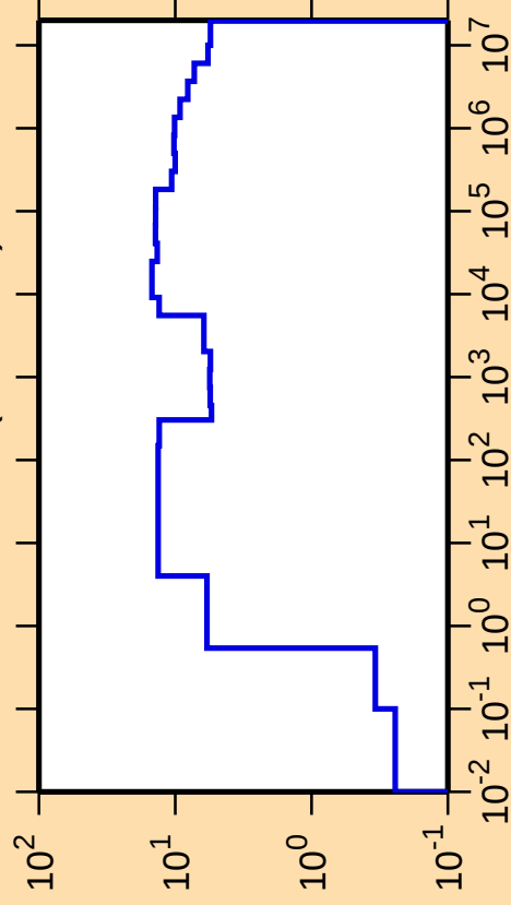
\Delta\sigma/\sigma vs. E for ^{157}\text{Gd}(n,\text{nonel.})
