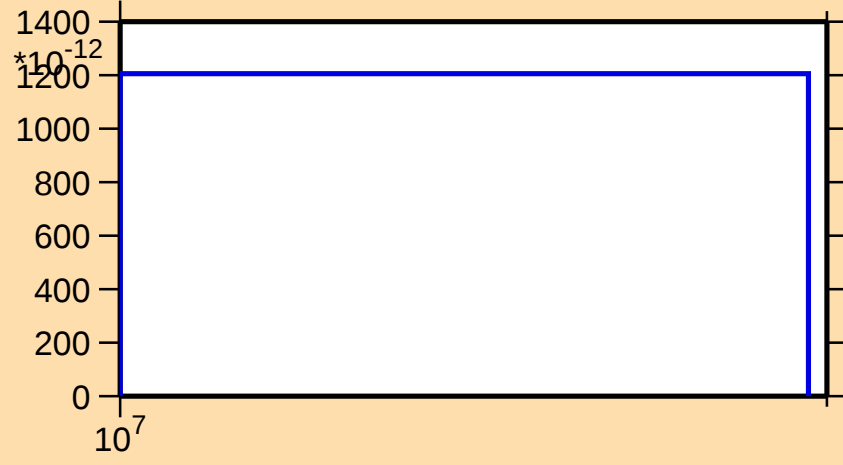
\sigma vs. E for ^{157}\text{Gd}(n,2np)
