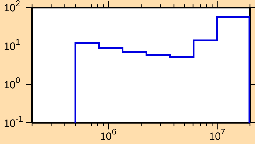
\Delta\sigma/\sigma vs. E for ^{157}\text{Gd}(n,n\text{cont.})
