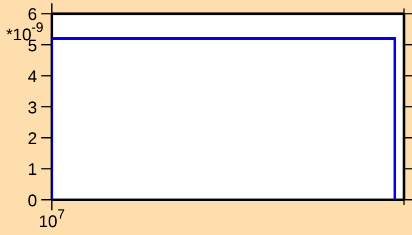
\sigma vs. E for ^{157}\text{Gd}(n,2n\alpha)
