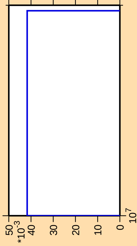
\Delta\sigma/\sigma vs. E for ^{157}\text{Gd}(n,p\alpha)
