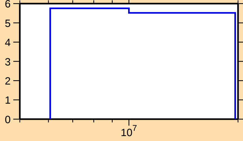
\Delta\sigma/\sigma vs. E for ^{157}\text{Gd}(n,\text{nonel.})
