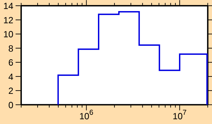
\Delta\sigma/\sigma vs. E for ^{157}\text{Gd}(n,\text{el.})
