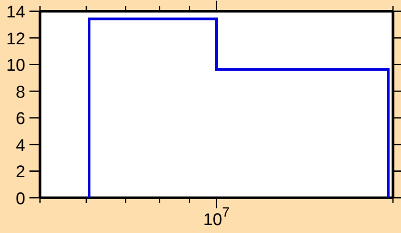
\Delta\sigma/\sigma vs. E for ^{157}\text{Gd}(n,2n)
