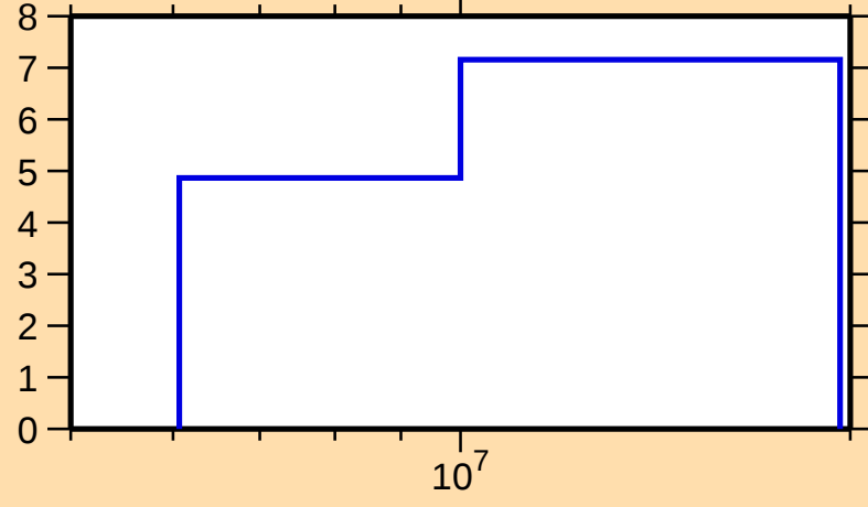
\Delta\sigma/\sigma vs. E for ^{157}\text{Gd}(n,\text{el.})
