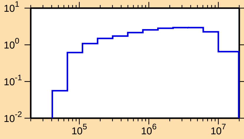
\sigma vs. E for ^{157}\text{Gd}(n,\text{inel.})
