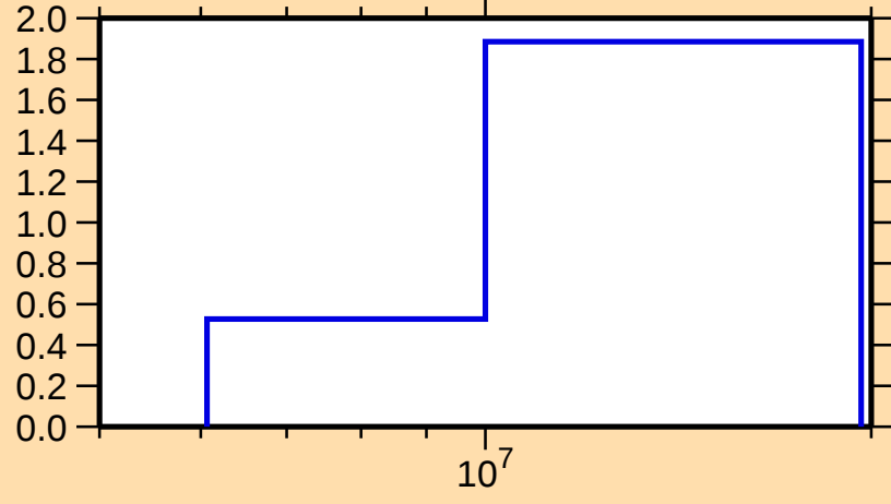
\sigma vs. E for ^{157}\text{Gd}(n,2n)
