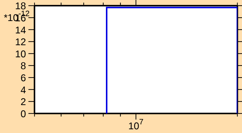
\sigma vs. E for ^{157}\text{Gd}(n,\text{nt})
