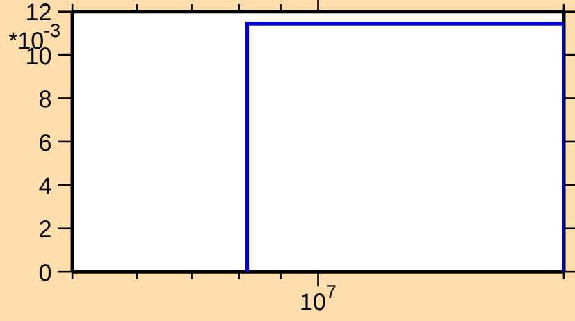
\sigma vs. E for ^{157}\text{Gd}(n,3n)
