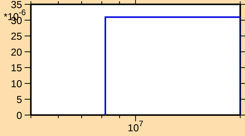
\sigma vs. E for ^{157}\text{Gd}(n,t)
