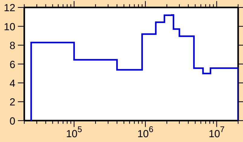
\Delta\sigma/\sigma vs. E for ^{157}\text{Gd}(n,\text{tot.})
