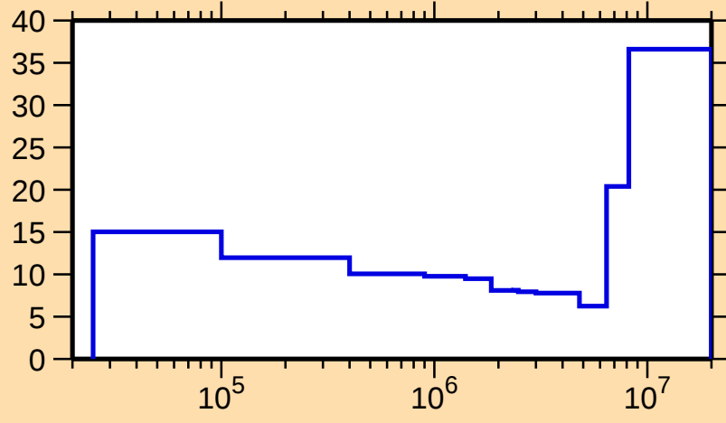
\Delta\sigma/\sigma vs. E for ^{157}\text{Gd}(n,\text{inel.})
