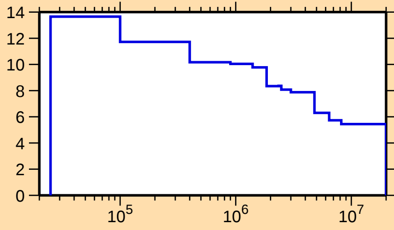
\Delta\sigma/\sigma vs. E for ^{157}\text{Gd}(n,\text{nonel.})
