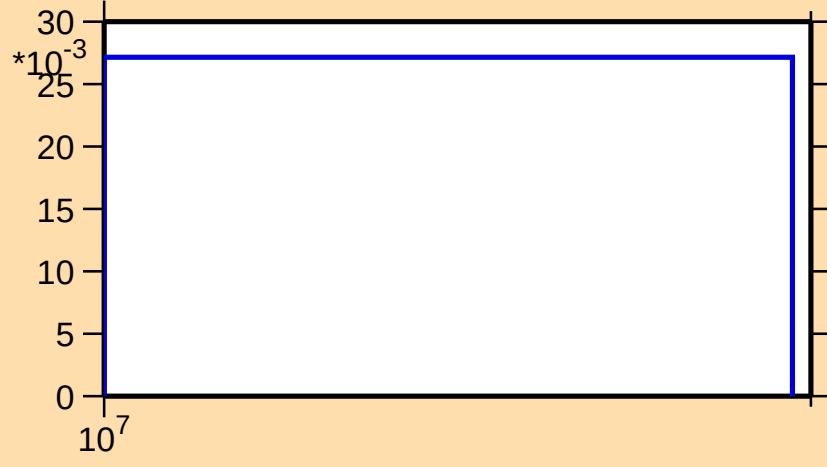
\sigma vs. E for ^{158}\text{Gd}(n,3n)
