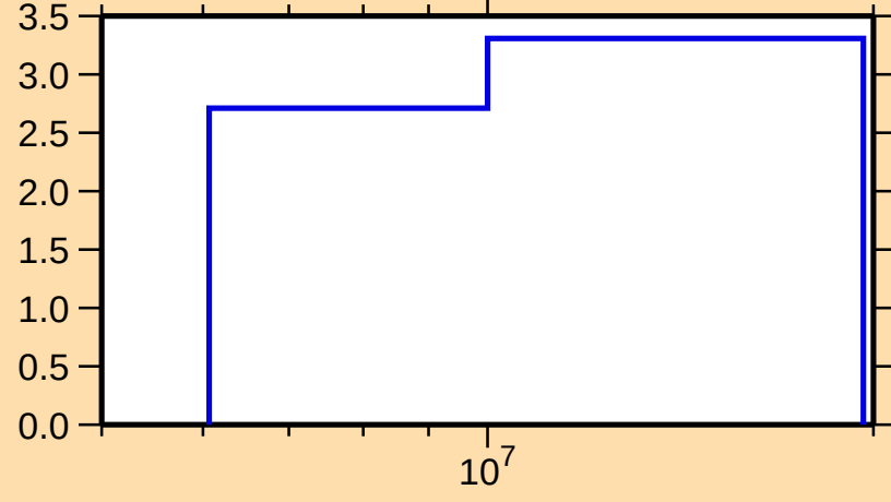
\Delta\sigma/\sigma vs. E for ^{158}\text{Gd}(n,\text{nonel.})
