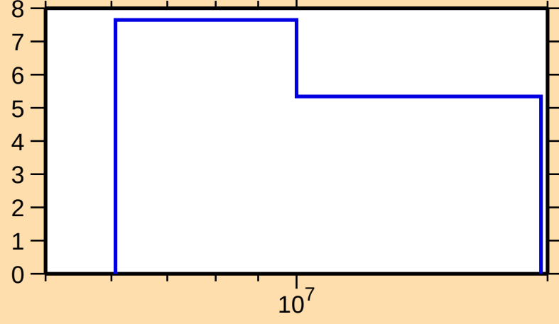
\Delta\sigma/\sigma vs. E for ^{158}\text{Gd}(n,\text{el.})
