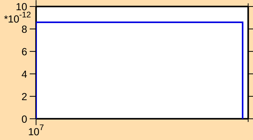
\sigma vs. E for ^{158}\text{Gd}(n,2np)
