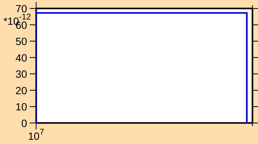
\sigma vs. E for ^{158}\text{Gd}(n,2n\alpha)
