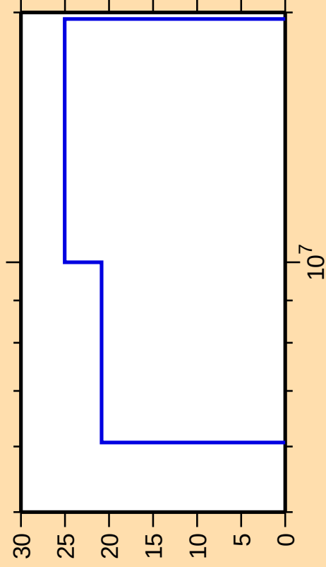
\Delta\sigma/\sigma vs. E for ^{158}\text{Gd}(n,n_1)
