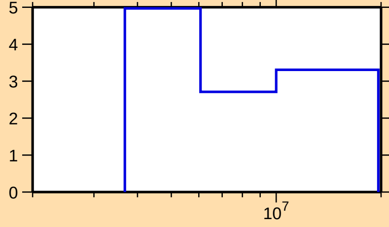
\Delta\sigma/\sigma vs. E for ^{158}\text{Gd}(n,\text{nonel.})
