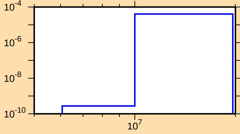
\sigma vs. E for ^{158}\text{Gd}(n,n\alpha)
