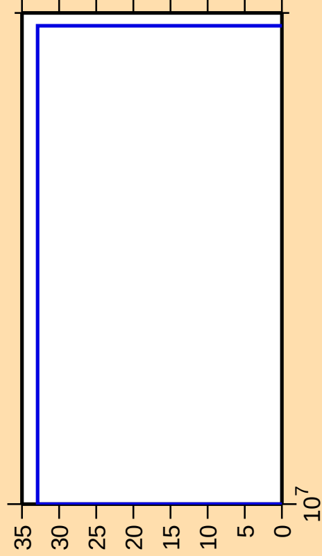
\Delta\sigma/\sigma vs. E for ^{158}\text{Gd}(n,3n)
