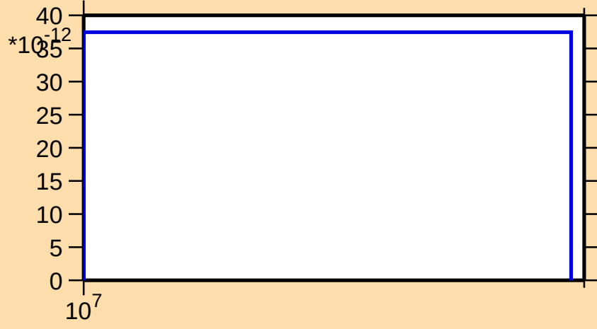
\sigma vs. E for ^{158}\text{Gd}(n,nt)
