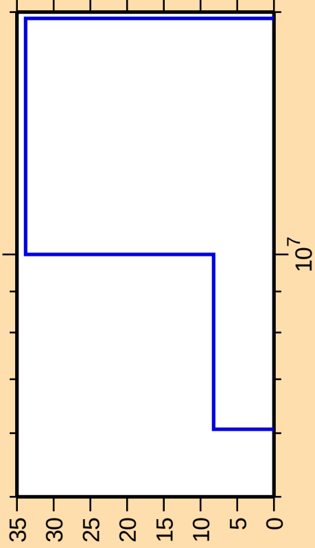
\Delta\sigma/\sigma vs. E for ^{158}\text{Gd}(n,n_{\text{cont}})
