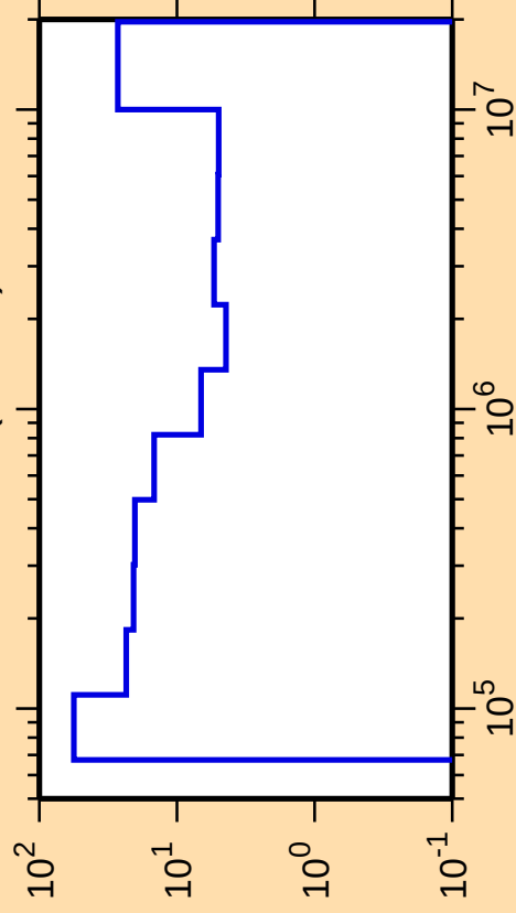
\Delta\sigma/\sigma vs. E for ^{158}\text{Gd}(n,\text{inel.})
