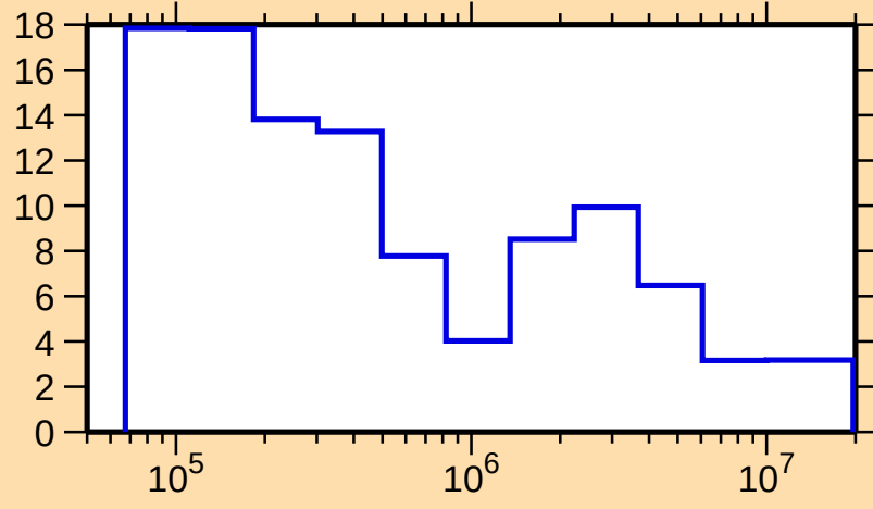
\Delta\sigma/\sigma vs. E for ^{158}\text{Gd}(n,\text{tot.})
