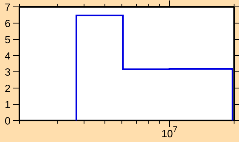
\Delta\sigma/\sigma vs. E for ^{158}\text{Gd}(n,\text{tot.})
