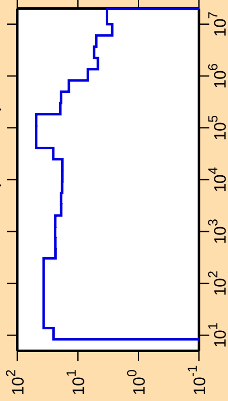
\Delta\sigma/\sigma vs. E for ^{158}\text{Gd}(n,\text{nonel.})
