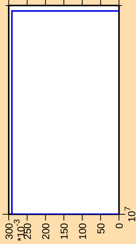
\Delta\sigma/\sigma vs. E for ^{158}\text{Gd}(n,\text{He}3)
