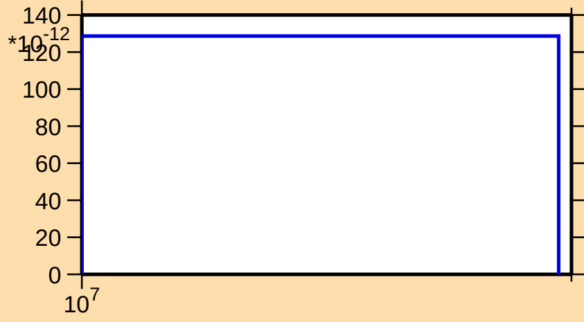
\sigma vs. E for ^{158}\text{Gd}(n,\text{nd})
