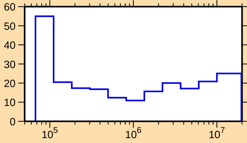
\Delta\sigma/\sigma vs. E for ^{158}\text{Gd}(n,n_1)
