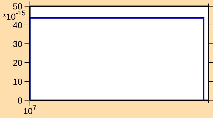
\sigma vs. E for ^{158}\text{Gd}(n,\text{He}3)
