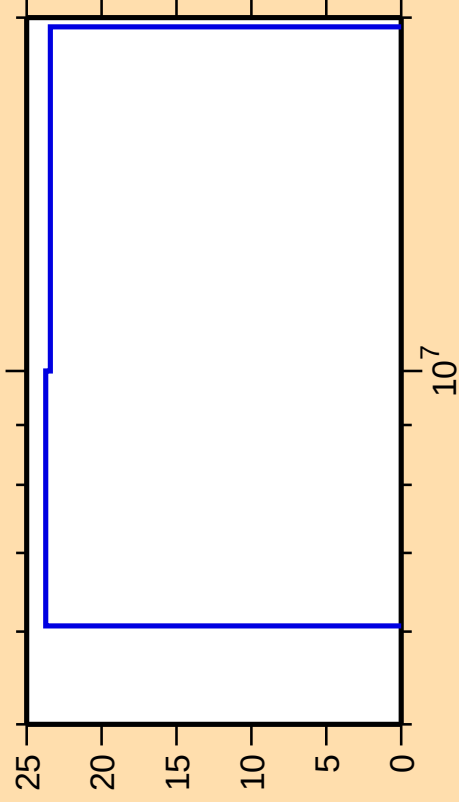
\Delta\sigma/\sigma vs. E for ^{158}\text{Gd}(n,p)
