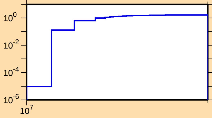
\sigma vs. E for ^{166}\text{Gd}(n,3n)
