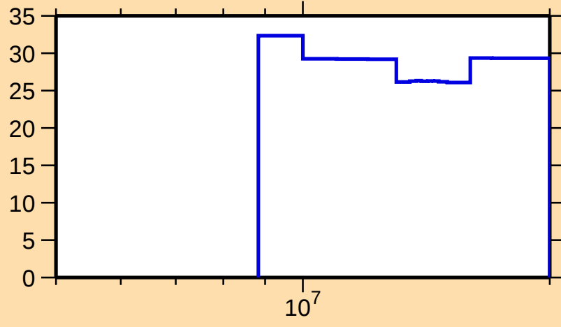
\Delta\sigma/\sigma vs. E for ^{166}\text{Gd}(n,\text{el.})
