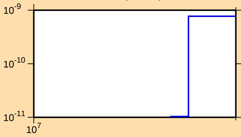
\sigma vs. E for ^{166}\text{Gd}(n,2n\alpha)
