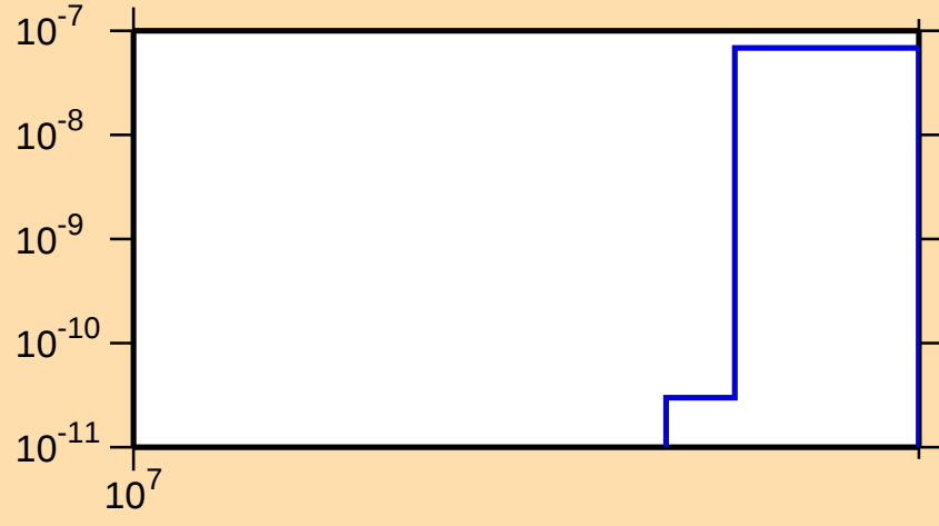
\sigma vs. E for ^{166}\text{Gd}(n,\text{nt})
