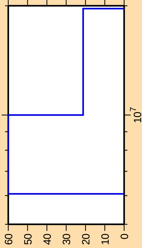
\Delta\sigma/\sigma vs. E for ^{166}\text{Gd}(n,n_{\text{cont}})
