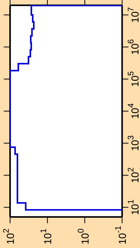
\Delta\sigma/\sigma vs. E for ^{166}\text{Gd}(n,\text{nonel.})
