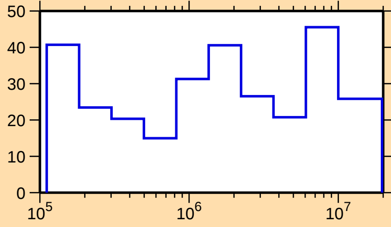
\Delta\sigma/\sigma vs. E for ^{166}\text{Gd}(n,\text{el.})
