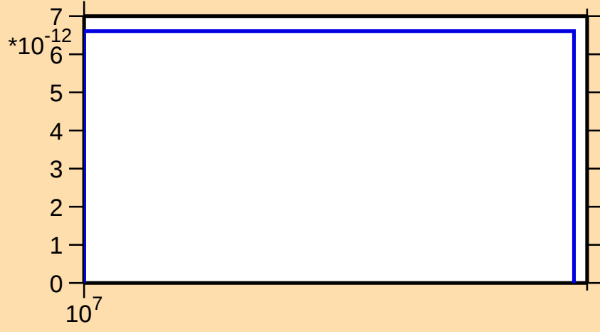
\sigma vs. E for ^{166}\text{Gd}(n,2n\alpha)
