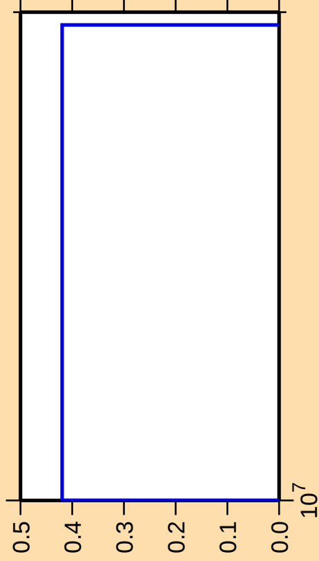
\Delta\sigma/\sigma vs. E for ^{166}\text{Gd}(n,2np)
