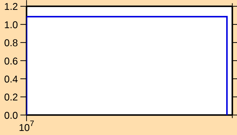
\sigma vs. E for ^{166}\text{Gd}(n,3n)
