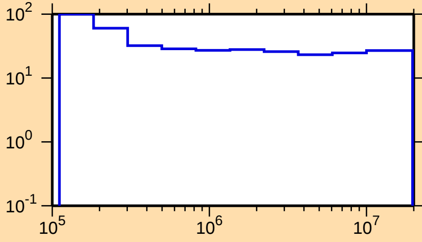
\Delta\sigma/\sigma vs. E for ^{166}\text{Gd}(n,\text{nonel.})
