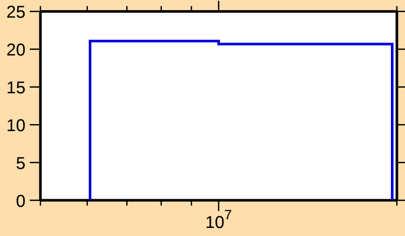
\Delta\sigma/\sigma vs. E for ^{166}\text{Gd}(n,\text{tot.})
