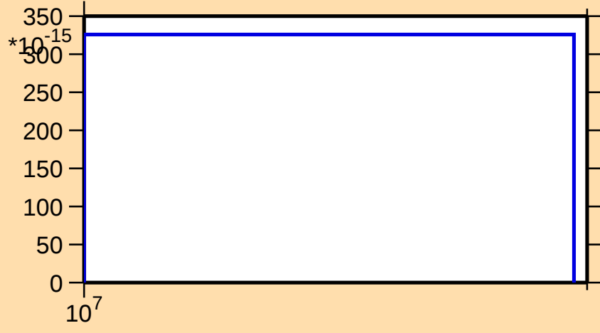
\sigma vs. E for ^{166}\text{Gd}(n,2np)
