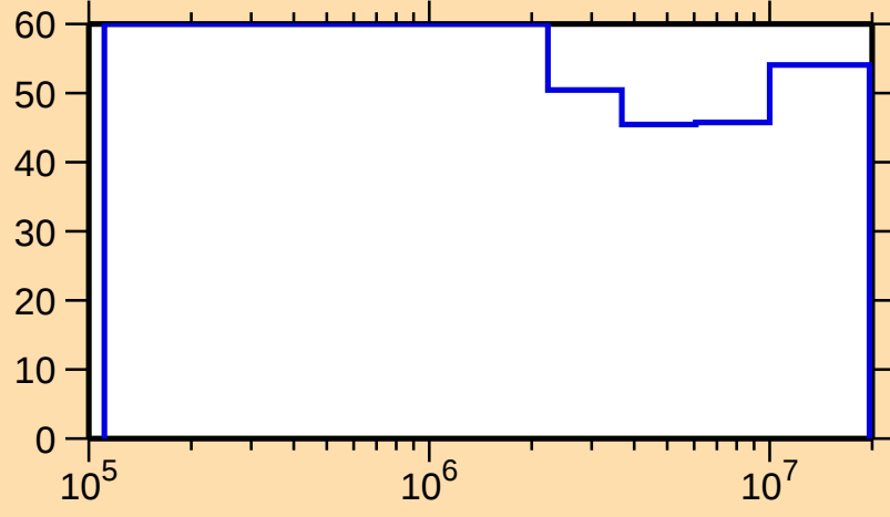
\Delta\sigma/\sigma vs. E for ^{166}\text{Gd}(n,n_1)
