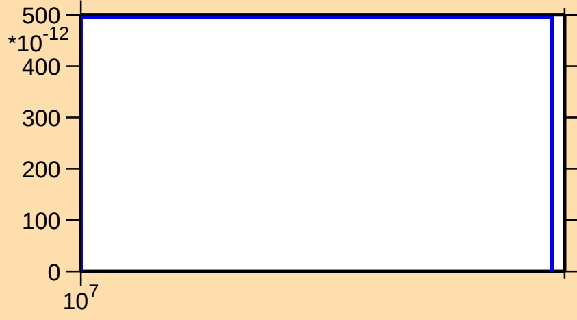
\sigma vs. E for ^{166}\text{Gd}(n,nt)
