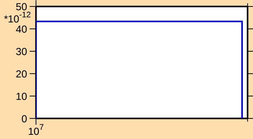
\sigma vs. E for ^{166}\text{Gd}(n,\text{nd})
