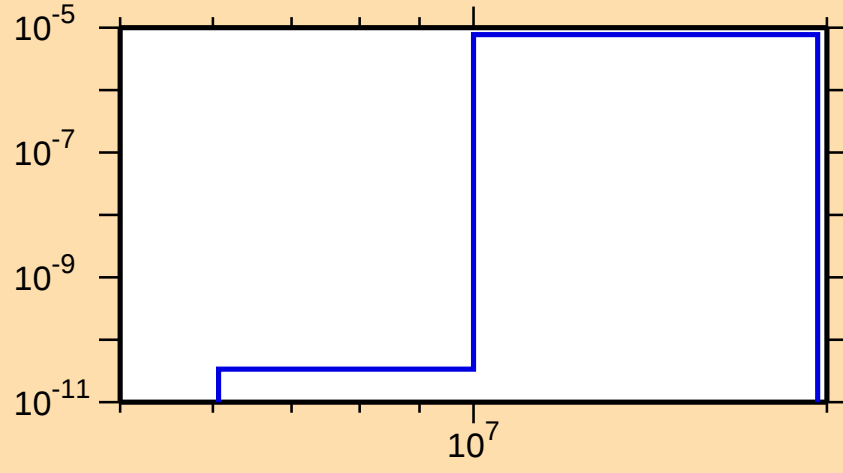
\sigma vs. E for ^{166}\text{Gd}(n,\alpha)
