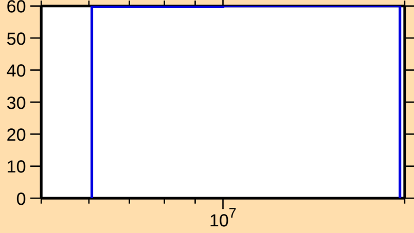
\Delta\sigma/\sigma vs. E for ^{166}\text{Gd}(n,2n)
