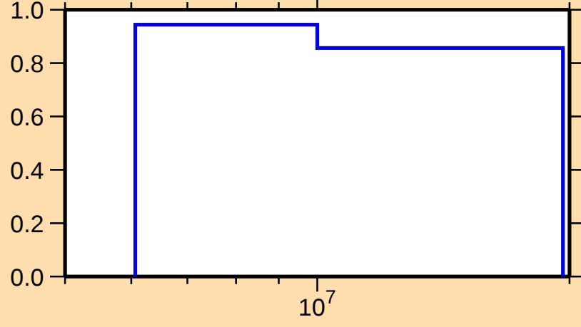
\sigma vs. E for ^{166}\text{Gd}(n,2n)
