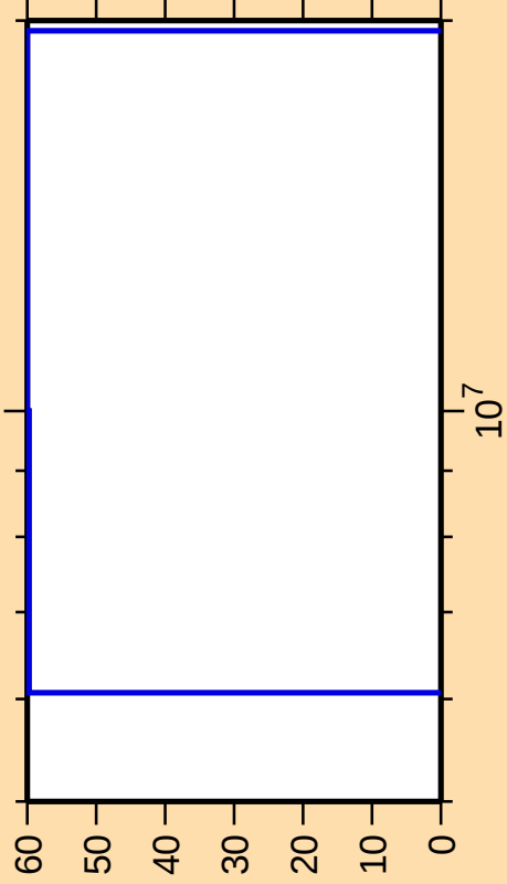
\Delta\sigma/\sigma vs. E for ^{166}\text{Gd}(n,2n)
