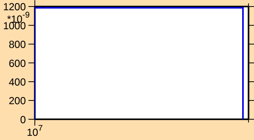
\sigma vs. E for ^{166}\text{Gd}(n,np)
