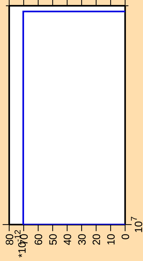
\Delta\sigma/\sigma vs. E for ^{166}\text{Gd}(\text{mt } 11)
