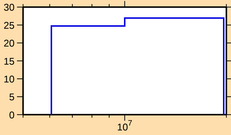
\Delta\sigma/\sigma vs. E for ^{166}\text{Gd}(n,\text{nonel.})
