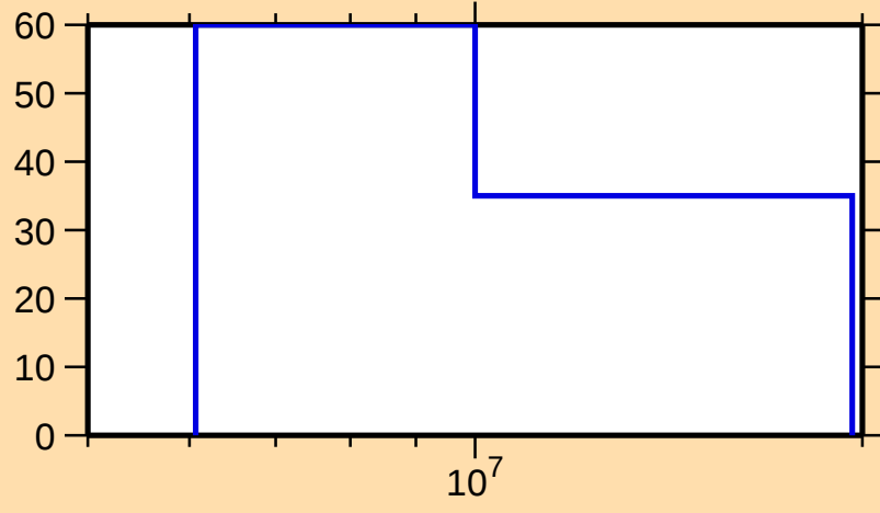
\Delta\sigma/\sigma vs. E for ^{166}\text{Gd}(n,\text{inel.})
