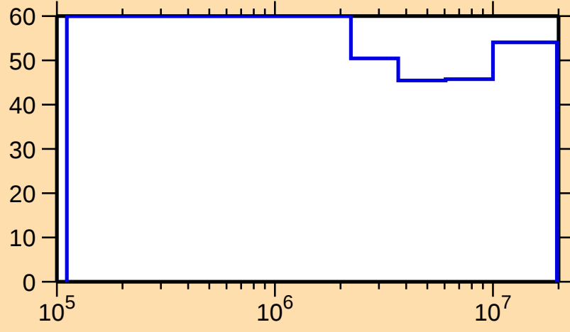
\Delta\sigma/\sigma vs. E for ^{166}\text{Gd}(n,n_1)
