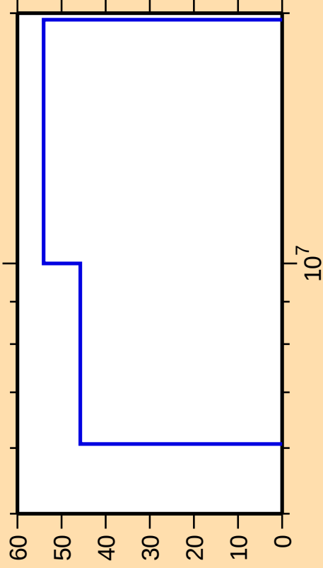
\Delta\sigma/\sigma vs. E for ^{166}\text{Gd}(n,n_1)
