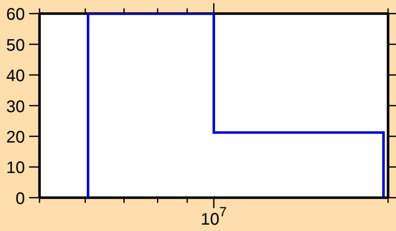
\Delta\sigma/\sigma vs. E for ^{166}\text{Gd}(n,n\text{cont.})
