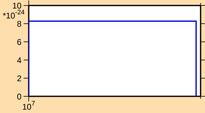
\sigma vs. E for ^{166}\text{Gd}(\text{mt } 11)
