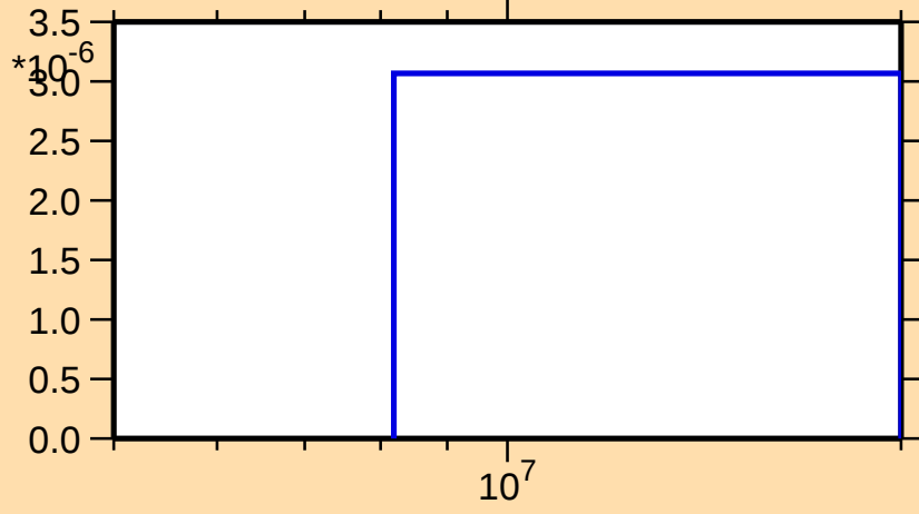
\sigma vs. E for ^{166}\text{Gd}(n,t)
