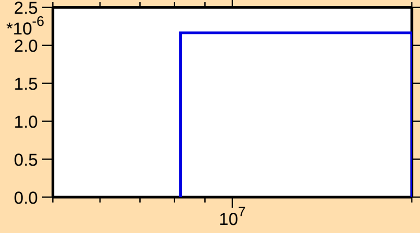
\sigma vs. E for ^{166}\text{Gd}(n,d)
