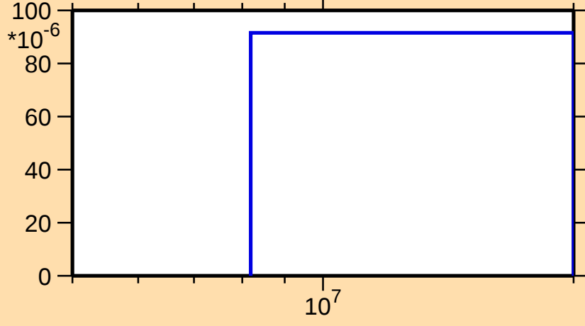
\sigma vs. E for ^{166}\text{Gd}(n,p)
