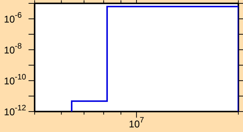
\sigma vs. E for ^{166}\text{Gd}(n,\alpha)
