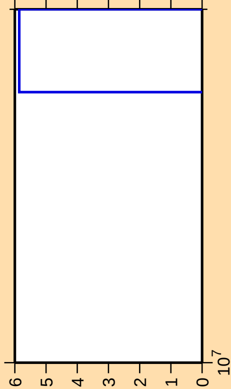
\Delta\sigma/\sigma vs. E for ^{66}\text{Ge}(n,2n\alpha)
