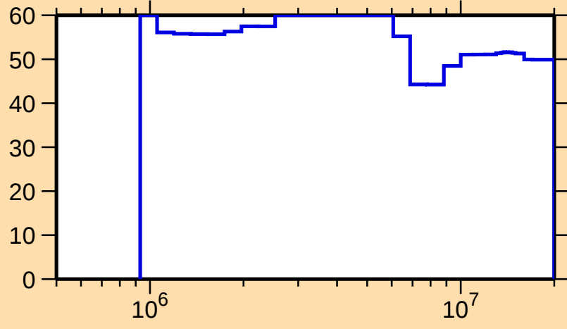
\Delta\sigma/\sigma vs. E for ^{66}\text{Ge}(n,\text{inel.})
