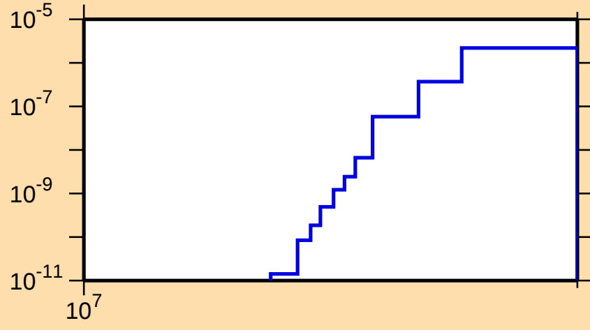
\sigma vs. E for ^{66}\text{Ge}(\text{mt117})
