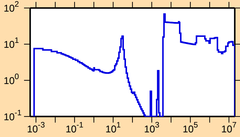
\Delta\sigma/\sigma vs. E for ^{66}\text{Ge}(n,\text{tot.})
