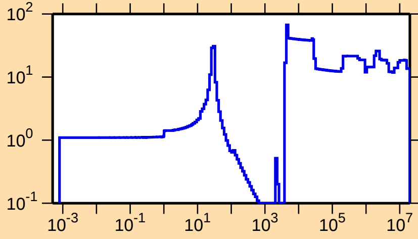
\Delta\sigma/\sigma vs. E for ^{66}\text{Ge}(n,\text{el.})
