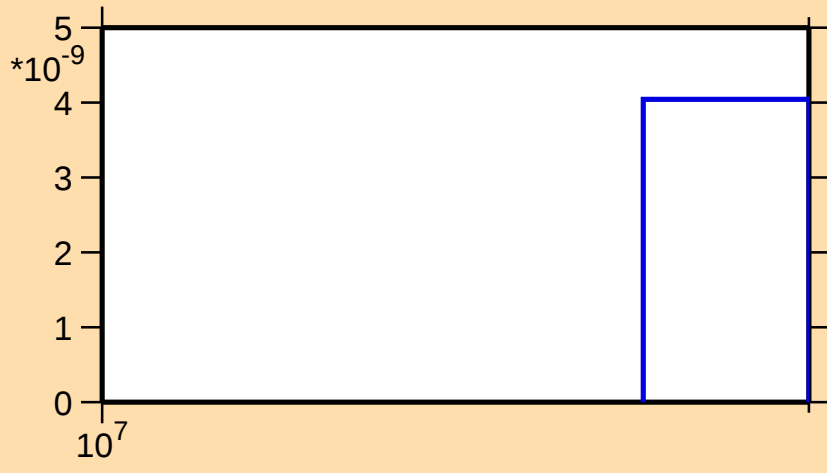
\sigma vs. E for ^{66}\text{Ge}(n,2np)
