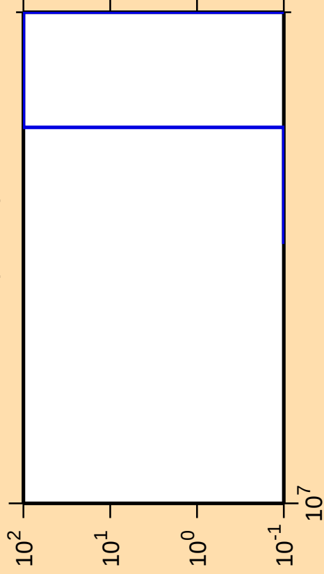
\Delta\sigma/\sigma vs. E for ^{66}\text{Ge}(\text{mt } 34)
