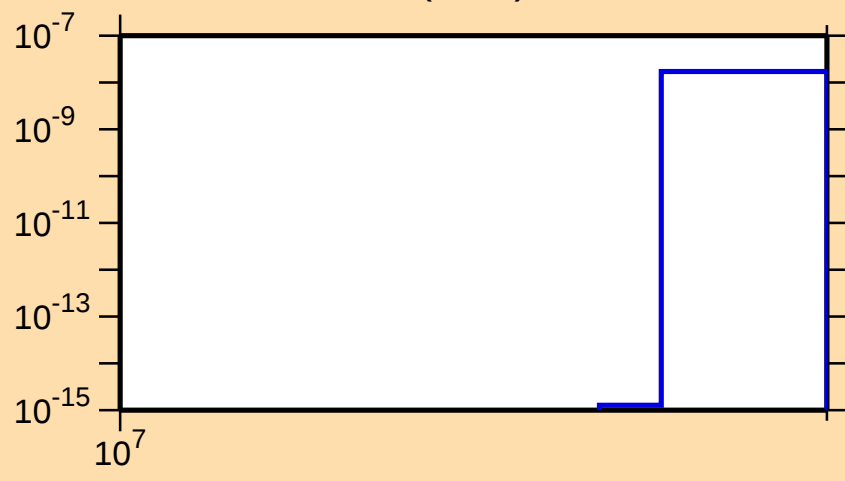
\sigma vs. E for ^{66}\text{Ge}(n,\text{nd})
