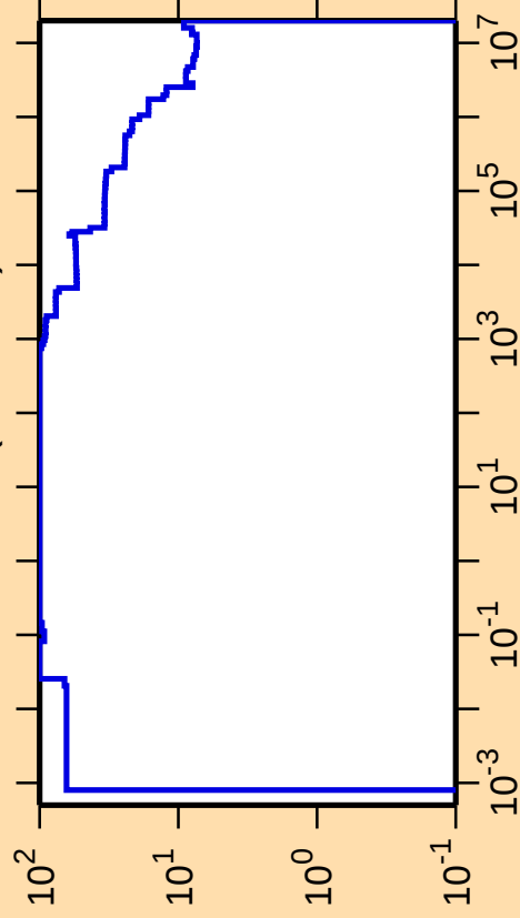
\Delta\sigma/\sigma vs. E for ^{66}\text{Ge}(n,\text{nonel.})
