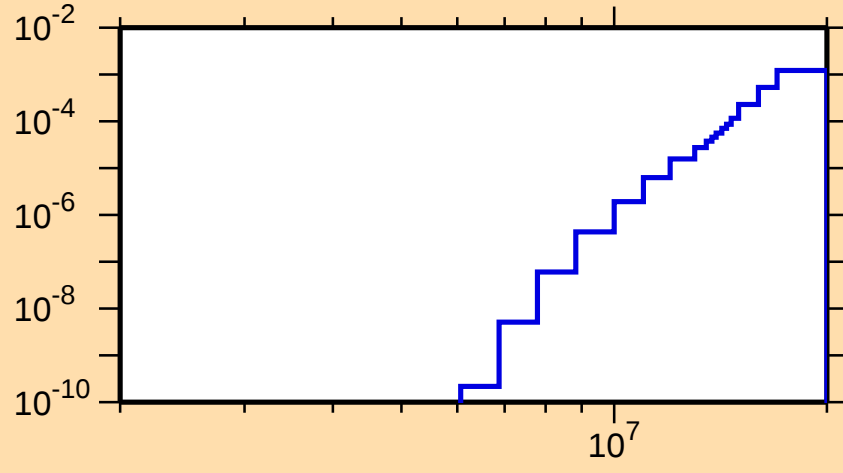
\sigma vs. E for ^{66}\text{Ge}(n,\text{He}3)
