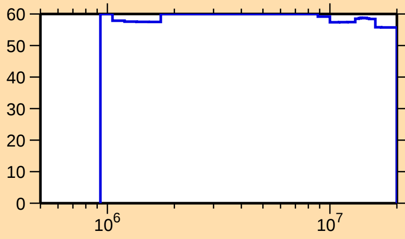
\Delta\sigma/\sigma vs. E for ^{66}\text{Ge}(n,n_1)
