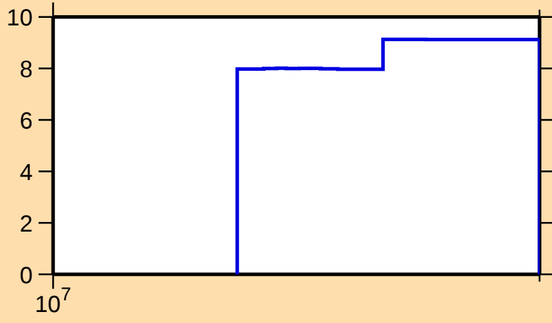
\Delta\sigma/\sigma vs. E for ^{66}\text{Ge}(n,\text{nonel.})
