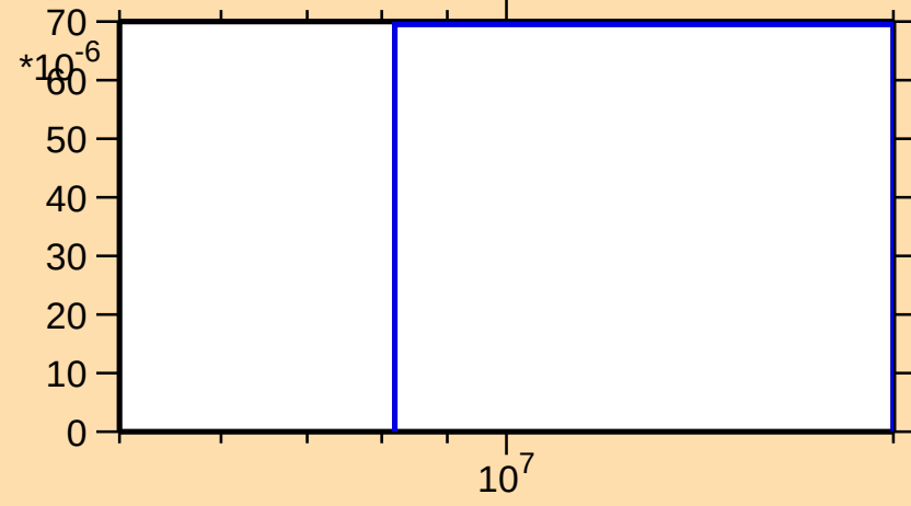
\sigma vs. E for ^{66}\text{Ge}(n,t)
