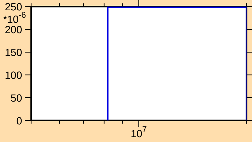
\sigma vs. E for ^{66}\text{Ge}(n,\text{pd})
