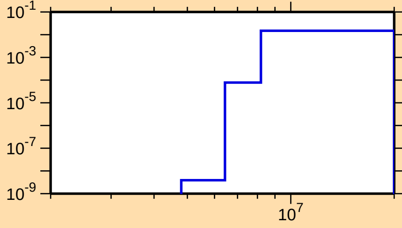
\sigma vs. E for ^{66}\text{Ge}(n,n\alpha)
