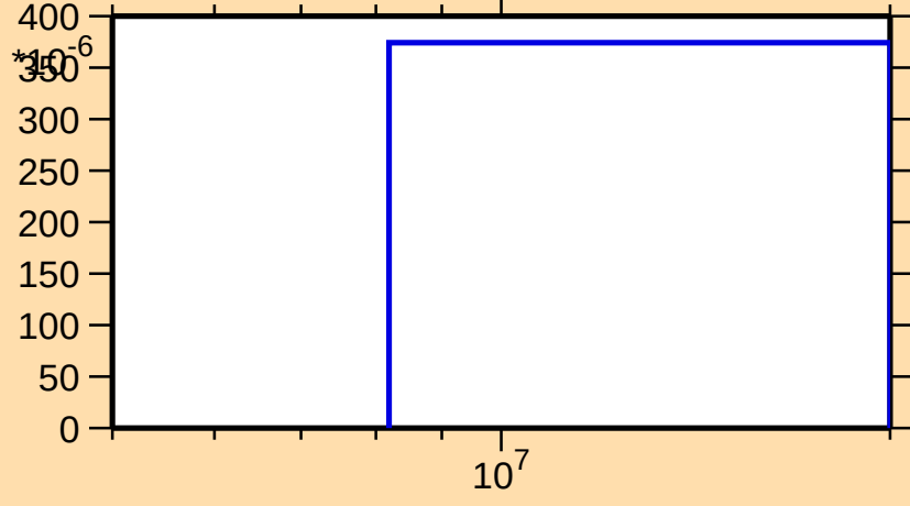
\sigma vs. E for ^{66}\text{Ge}(n,2n)
