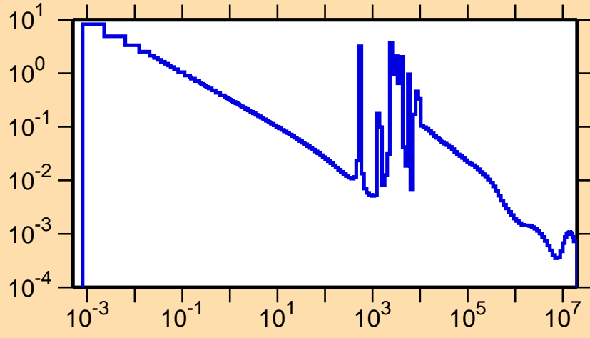
\sigma vs. E for ^{77}\text{Ge}(n,\gamma)
