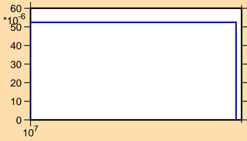
\sigma vs. E for ^{77}\text{Ge}(n,np)
