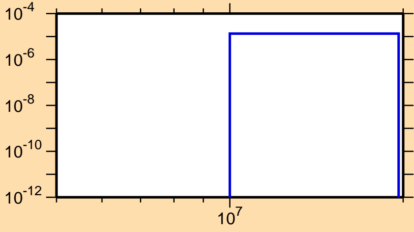
\sigma vs. E for ^{77}\text{Ge}(n,n\alpha)
