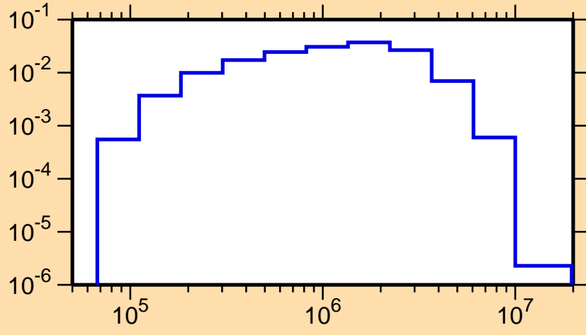
\sigma vs. E for ^{77}\text{Ge}(n,n_2)
