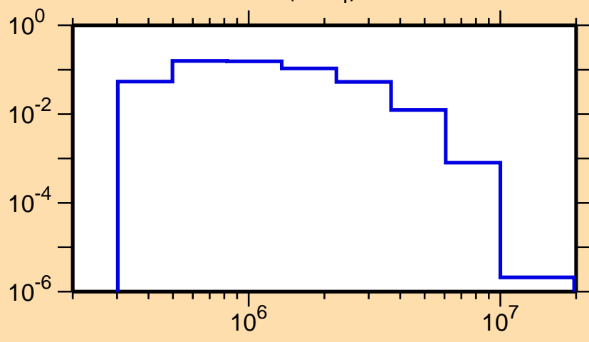
\sigma vs. E for ^{77}\text{Ge}(n,n_4)
