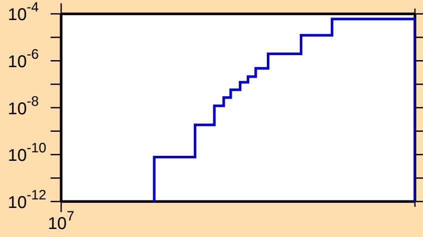
\sigma vs. E for ^{81}\text{Ge}(n,t)
