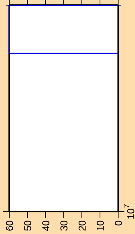
\Delta\sigma/\sigma vs. E for ^{81}\text{Ge}(n,\text{nt})
