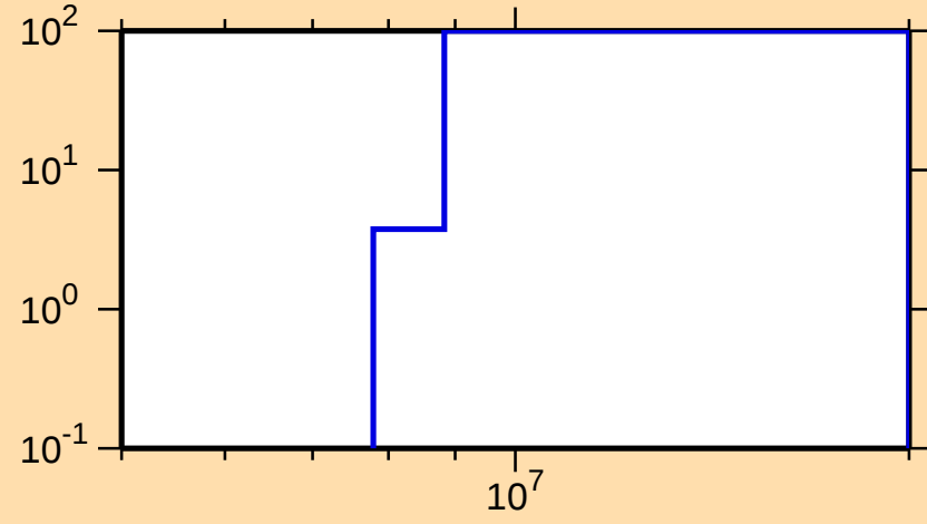
\Delta\sigma/\sigma vs. E for ^{81}\text{Ge}(n,p)
