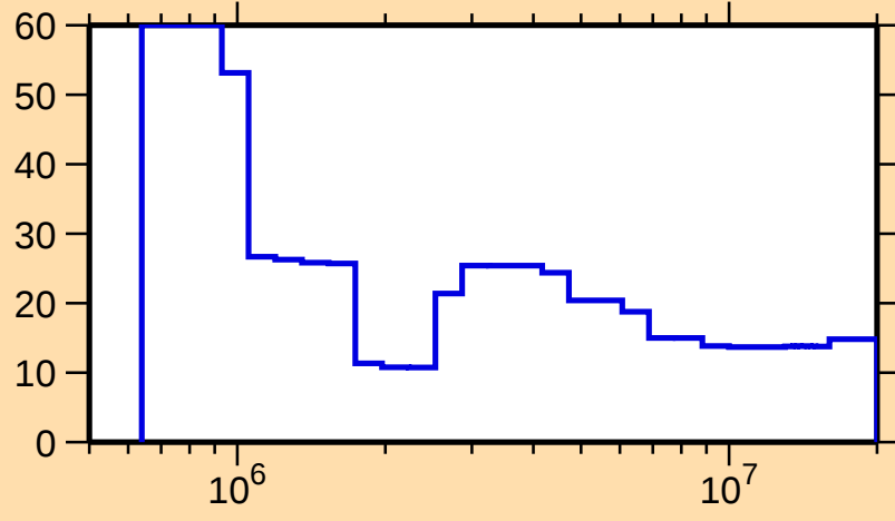
\Delta\sigma/\sigma vs. E for ^{81}\text{Ge}(n,\text{nonel.})
