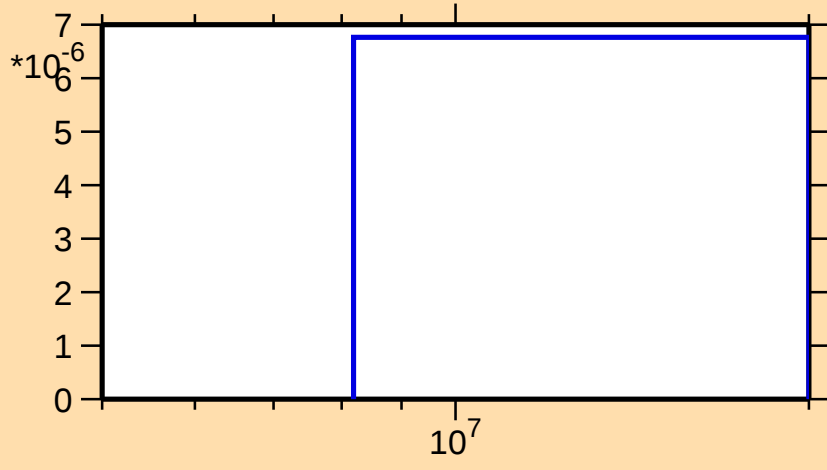
\sigma vs. E for ^{81}\text{Ge}(n,d)
