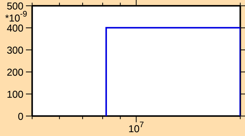
\sigma vs. E for ^{81}\text{Ge}(n,n\alpha)
