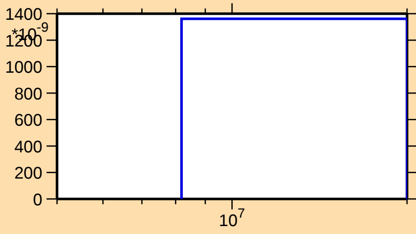
\sigma vs. E for ^{81}\text{Ge}(n,np)
