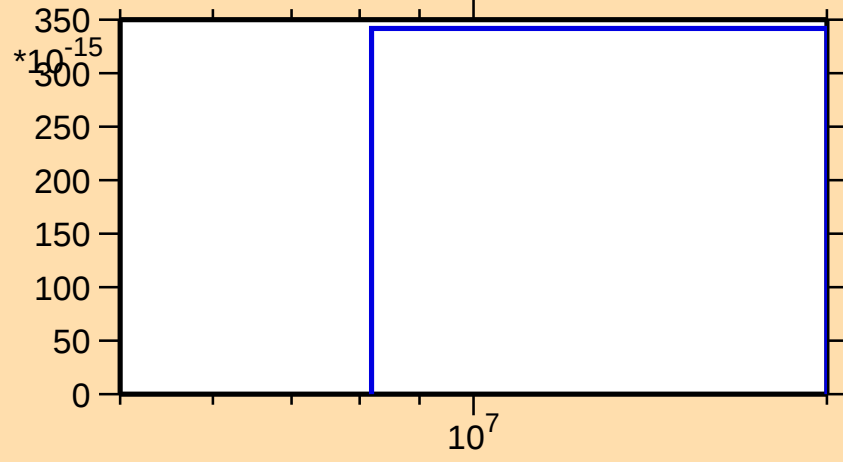
\sigma vs. E for ^{81}\text{Ge}(n,2n\alpha)
