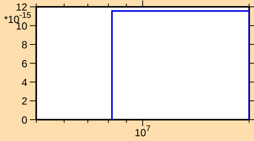
\sigma vs. E for ^{81}\text{Ge}(n,2np)
