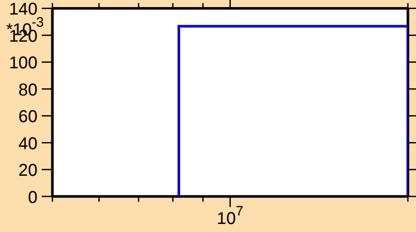
\sigma vs. E for ^{81}\text{Ge}(n,3n)
