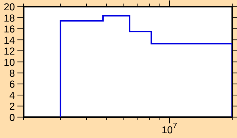
\Delta\sigma/\sigma vs. E for ^{81}\text{Ge}(n,n\text{onel.})
