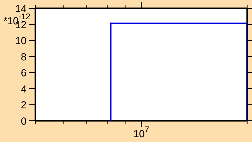
\sigma vs. E for ^{81}\text{Ge}(n,\text{nt})
