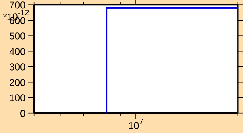
\sigma vs. E for ^{81}\text{Ge}(n,\text{nd})
