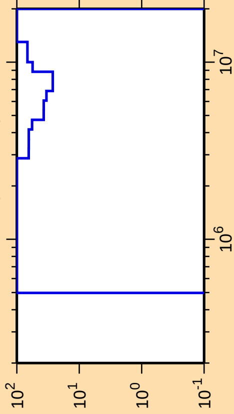
\Delta\sigma/\sigma vs. E for ^{165}\text{Hf}(n,\text{ncont.})
