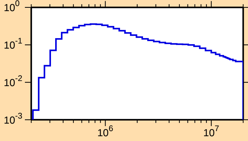
\sigma vs. E for ^{165}\text{Hf}(n,n_4)
