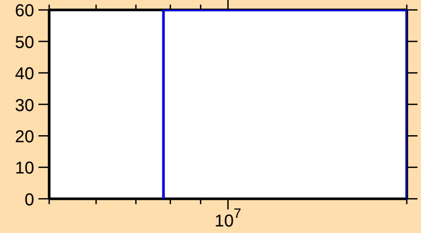
\Delta\sigma/\sigma vs. E for ^{165}\text{Hf}(n,2n)
