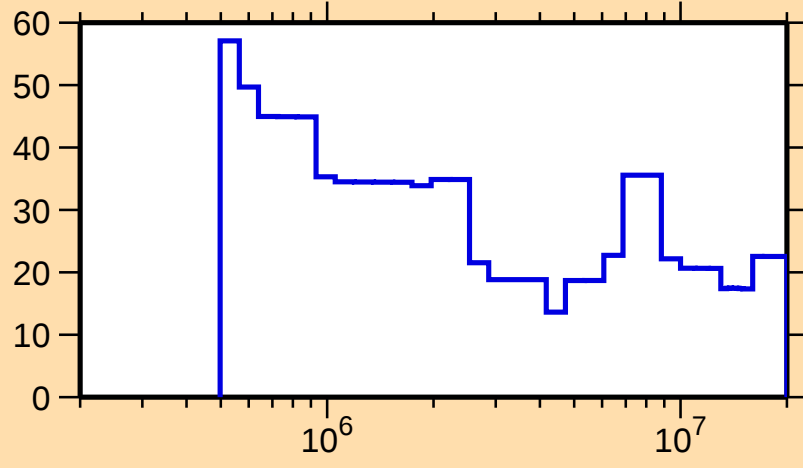
\Delta\sigma/\sigma vs. E for ^{165}\text{Hf}(n,\text{el.})
