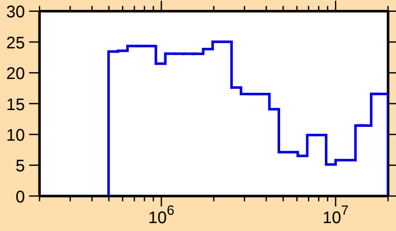
\Delta\sigma/\sigma vs. E for ^{165}\text{Hf}(n,\text{tot.})
