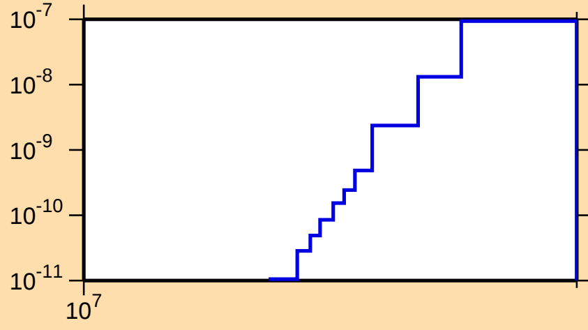
\sigma vs. E for ^{165}\text{Hf}(\text{mt 45})
