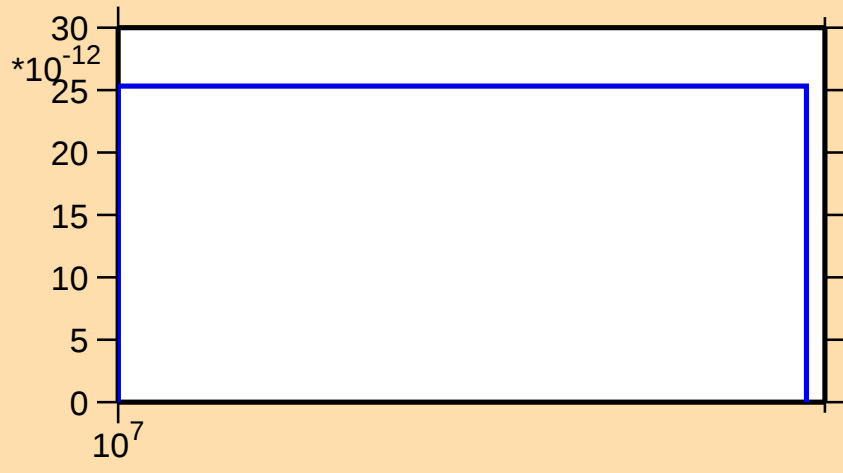
\sigma vs. E for ^{165}\text{Hf}(\text{mt117})
