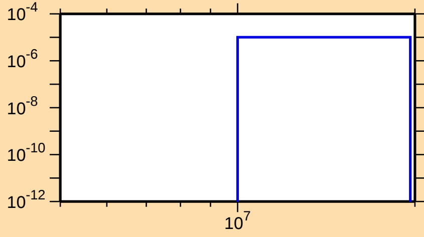
\sigma vs. E for ^{165}\text{Hf}(n,2n\alpha)
