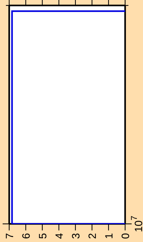
\Delta\sigma/\sigma vs. E for ^{165}\text{Hf}(n,nt)
