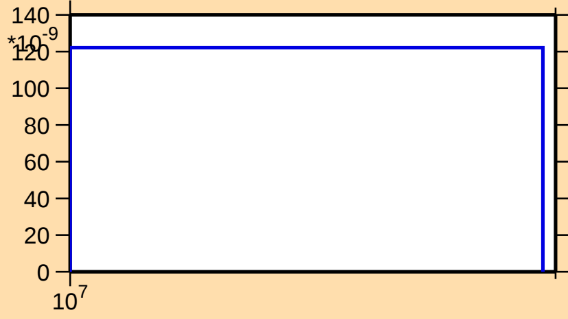
\sigma vs. E for ^{165}\text{Hf}(n,\text{nd})
