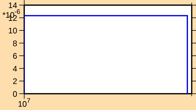
\sigma vs. E for ^{165}\text{Hf}(n,2np)
