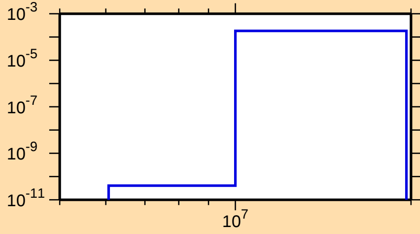
\sigma vs. E for ^{165}\text{Hf}(n,t)
