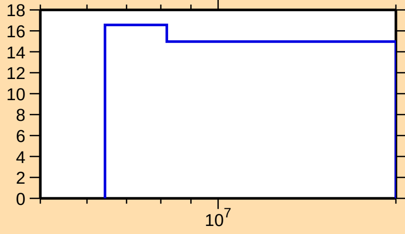
\Delta\sigma/\sigma vs. E for ^{165}\text{Hf}(n,\text{nonel.})
