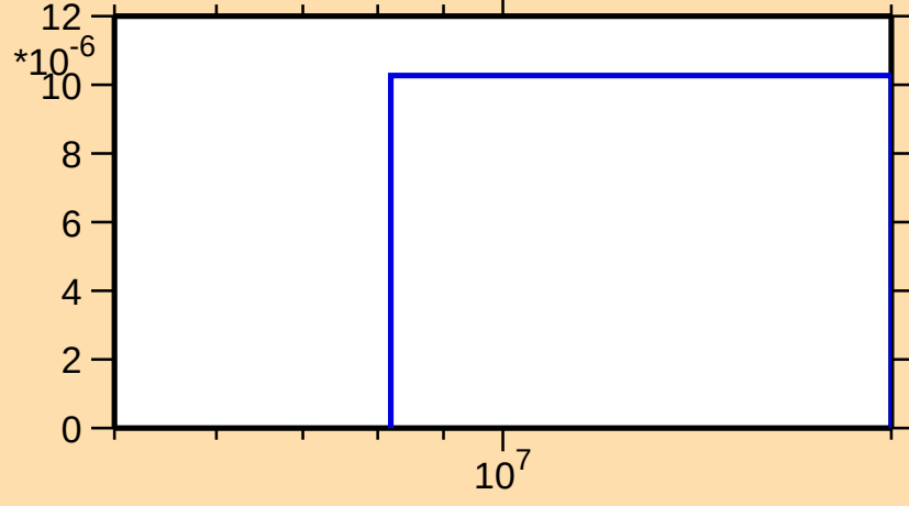
\sigma vs. E for ^{165}\text{Hf}(n,2np)
