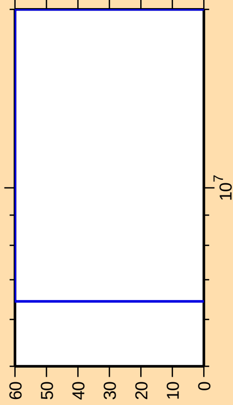
\Delta\sigma/\sigma vs. E for ^{165}\text{Hf}(n,n_1)
