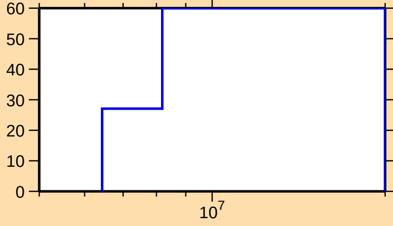
\Delta\sigma/\sigma vs. E for ^{165}\text{Hf}(n,\text{inel.})
