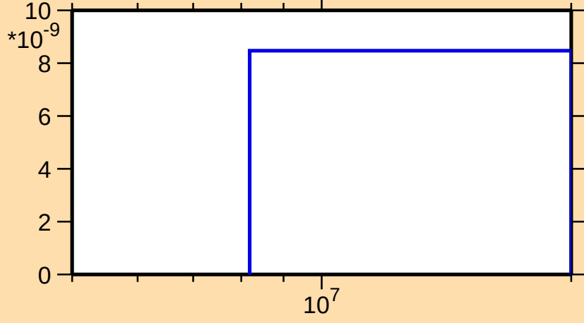
\sigma vs. E for ^{165}\text{Hf}(n,\text{pd})
