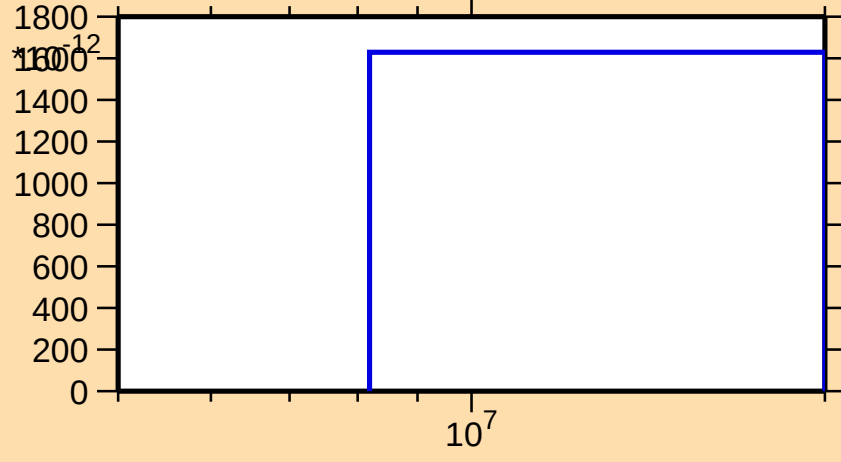
\sigma vs. E for ^{165}\text{Hf}(\text{mt } 45)
