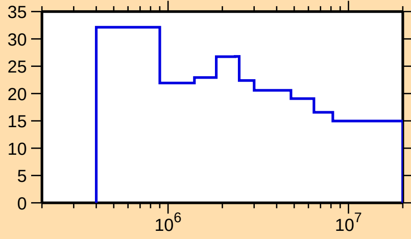
\Delta\sigma/\sigma vs. E for ^{165}\text{Hf}(n,n\text{onel.})
