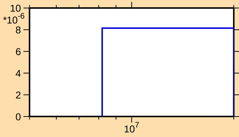
\sigma vs. E for ^{165}\text{Hf}(n,2n\alpha)
