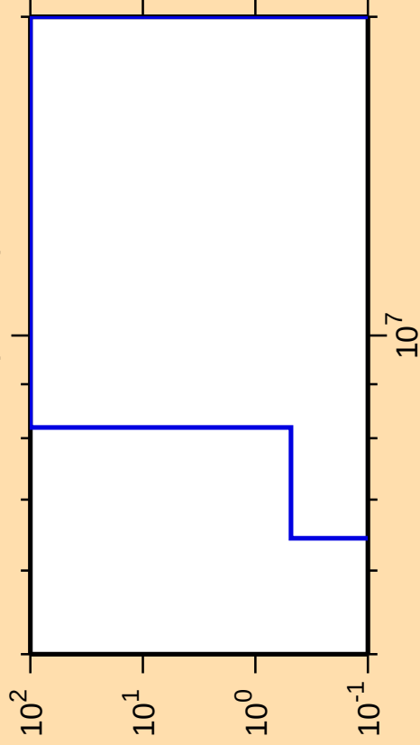
\Delta\sigma/\sigma vs. E for ^{165}\text{Hf}(n,\text{He3})
