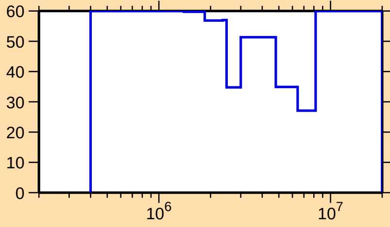
\Delta\sigma/\sigma vs. E for ^{165}\text{Hf}(n,\text{inel.})
