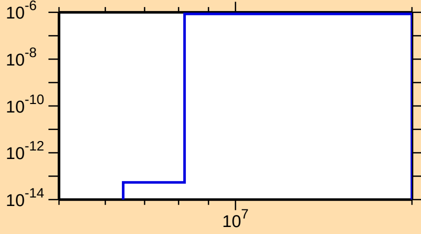
\sigma vs. E for ^{165}\text{Hf}(n,\text{He3})
