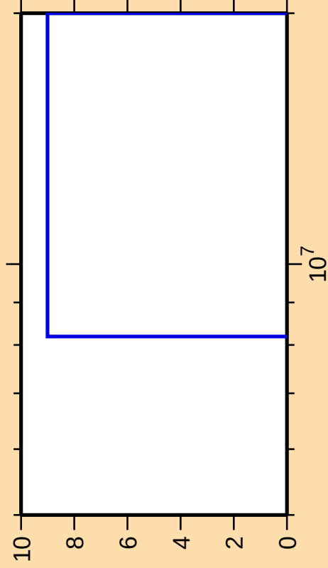
\Delta\sigma/\sigma vs. E for ^{165}\text{Hf}(n,nt)
