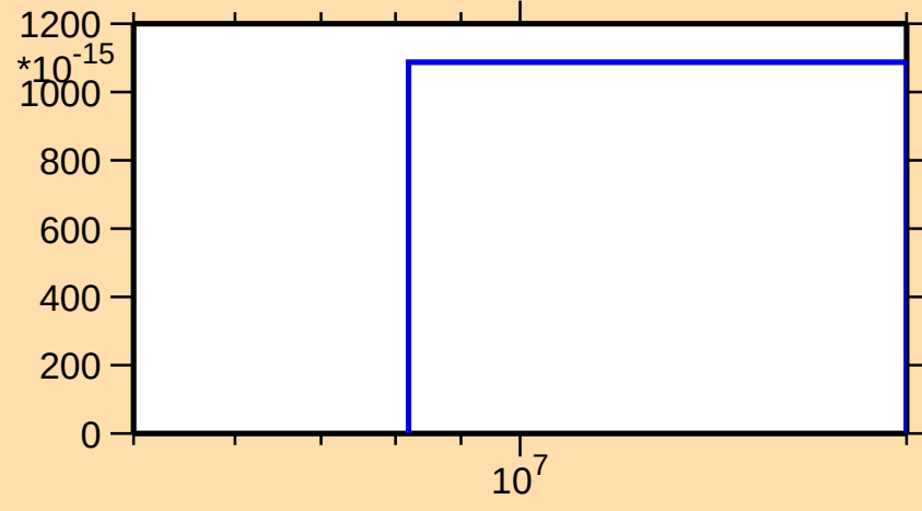
\sigma vs. E for ^{165}\text{Hf}(n,nt)
