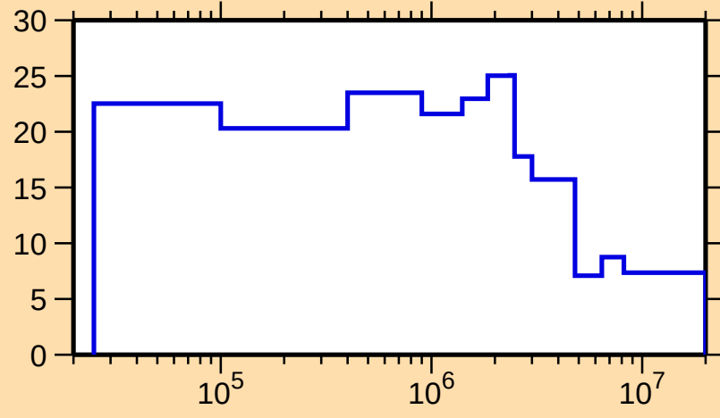
\Delta\sigma/\sigma vs. E for ^{165}\text{Hf}(n,\text{tot.})
