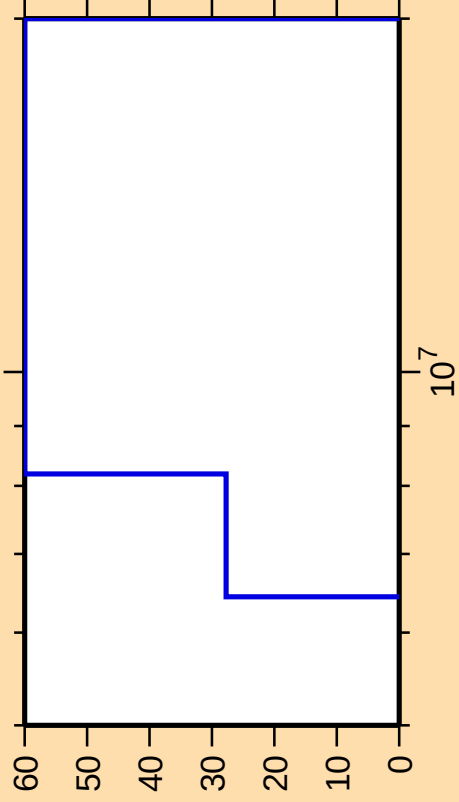
\Delta\sigma/\sigma vs. E for ^{165}\text{Hf}(n,n\text{cont.})
