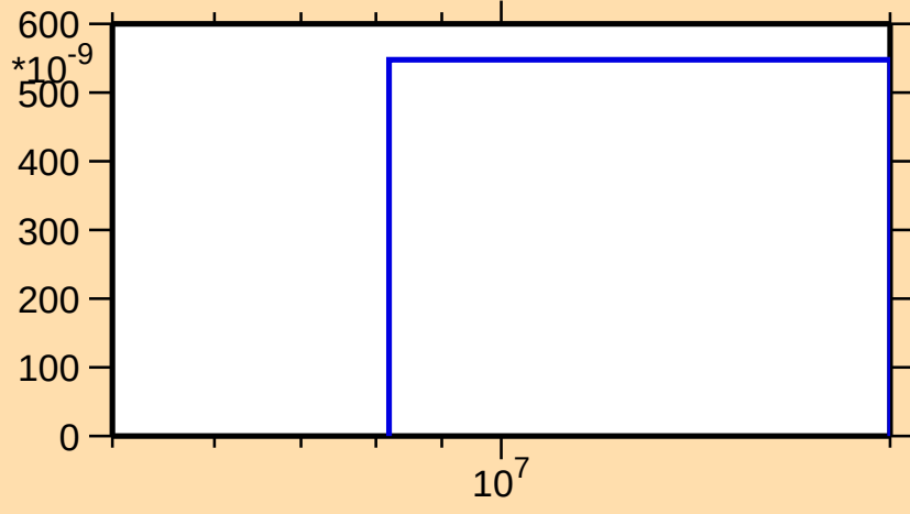
\sigma vs. E for ^{165}\text{Hf}(n,3n)
