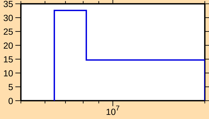
\Delta\sigma/\sigma vs. E for ^{165}\text{Hf}(n,\text{el.})
