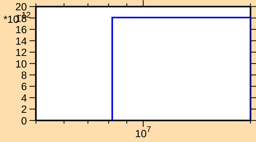
\sigma vs. E for ^{165}\text{Hf}(\text{mt } 34)
