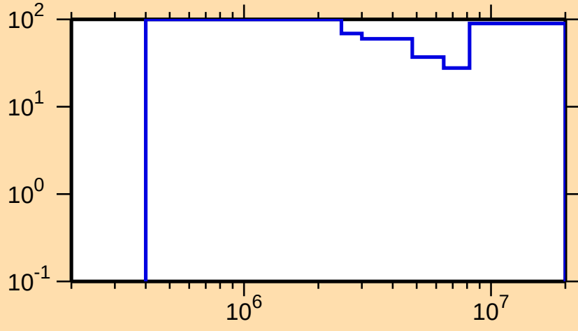
\Delta\sigma/\sigma vs. E for ^{165}\text{Hf}(n,n\text{cont.})
