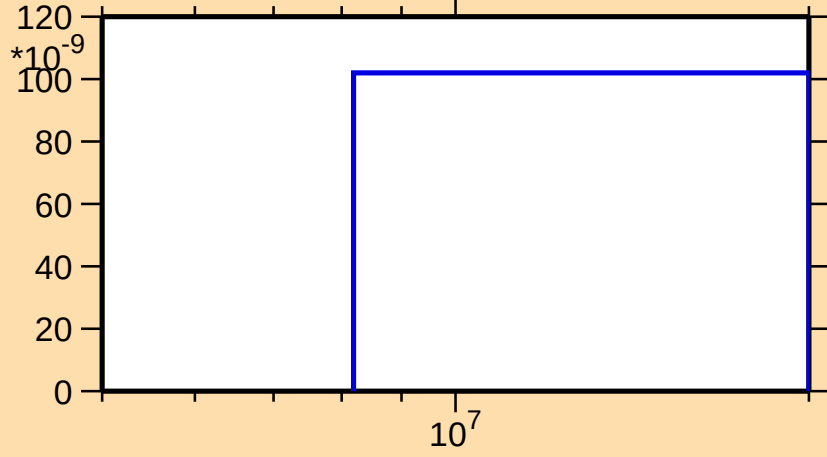
\sigma vs. E for ^{165}\text{Hf}(n,\text{nd})
