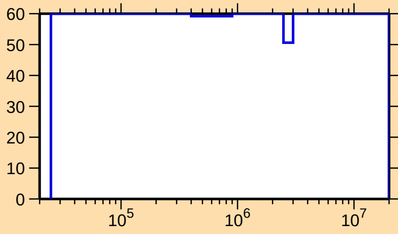
\Delta\sigma/\sigma vs. E for ^{165}\text{Hf}(n,n_1)
