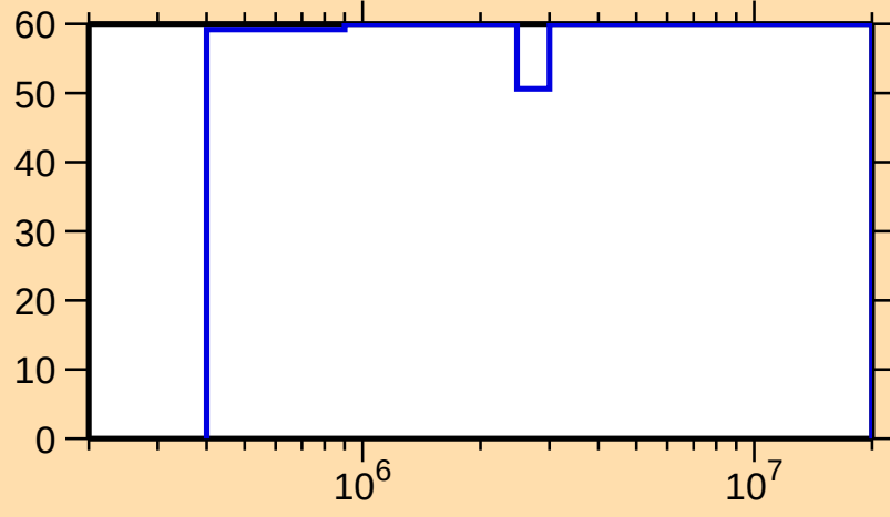
\Delta\sigma/\sigma vs. E for ^{165}\text{Hf}(n,n_1)
