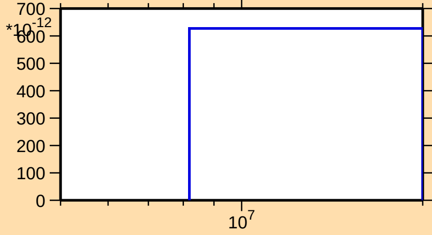
\sigma vs. E for ^{165}\text{Hf}(n,\text{pt})
