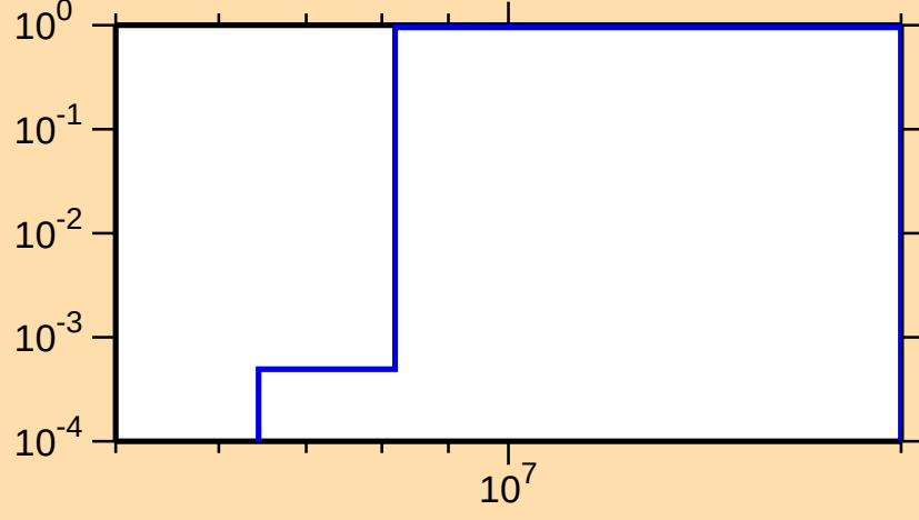
\sigma vs. E for ^{165}\text{Hf}(n,2n)
