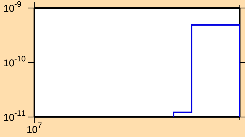
\sigma vs. E for ^{167}\text{Hf}(\text{mt } 34)
