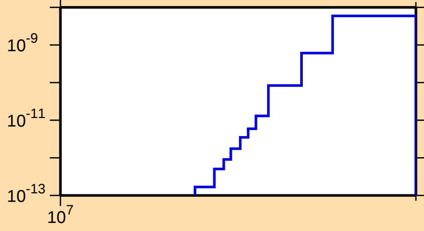
\sigma vs. E for ^{167}\text{Hf}(\text{mt 45})
