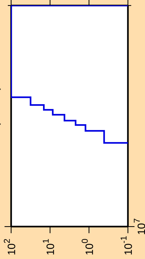
\Delta\sigma/\sigma vs. E for ^{167}\text{Hf}(\text{mt 45})
