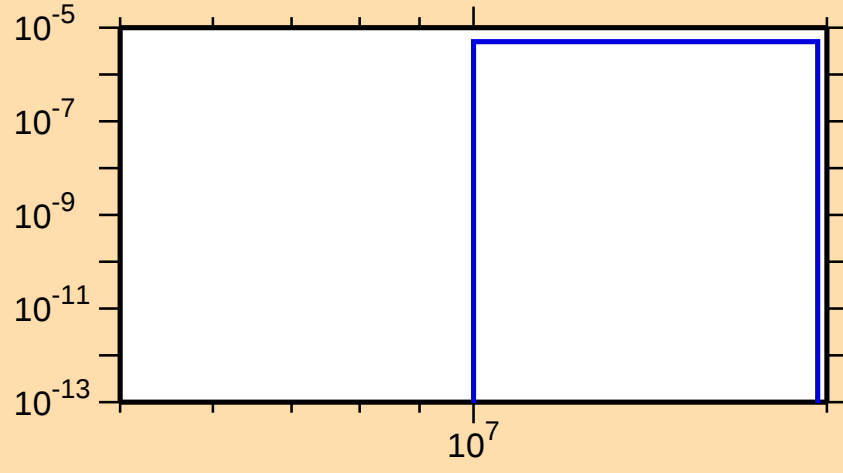
\sigma vs. E for ^{167}\text{Hf}(n,2n\alpha)
