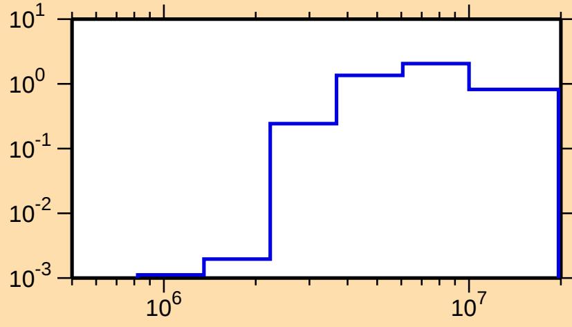
\sigma vs. E for ^{167}\text{Hf}(n,n\text{cont.})
