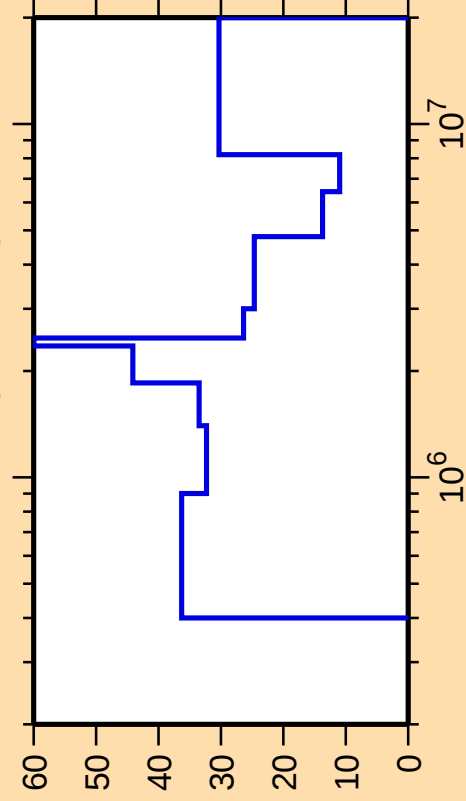
\Delta\sigma/\sigma vs. E for ^{167}\text{Hf}(n,\text{ncont.})
