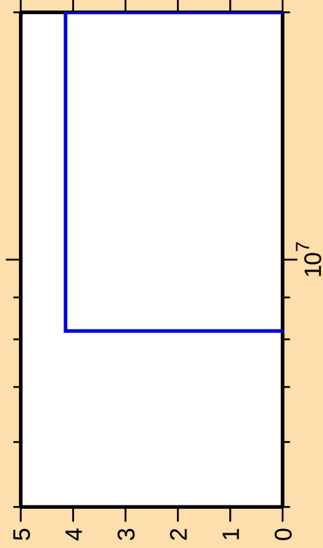
\Delta\sigma/\sigma vs. E for ^{167}\text{Hf}(n,nt)
