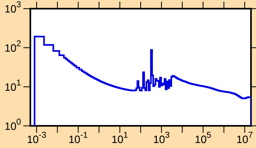
\sigma vs. E for ^{178}\text{Hf}(n,\text{tot.})
