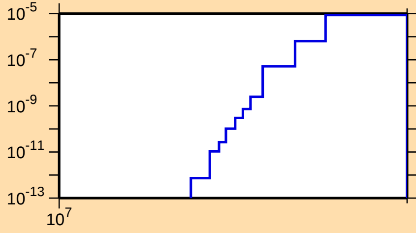
\sigma vs. E for ^{178}\text{Hf}(n,nd)
