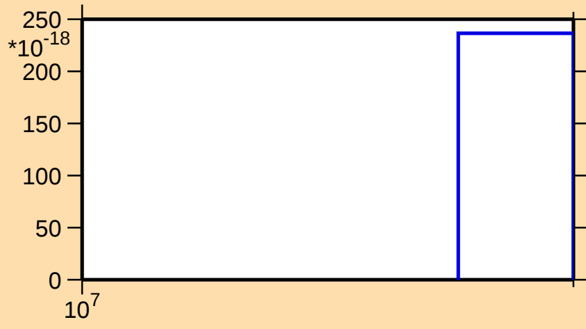
\sigma vs. E for ^{178}\text{Hf}(\text{mt } 42)
