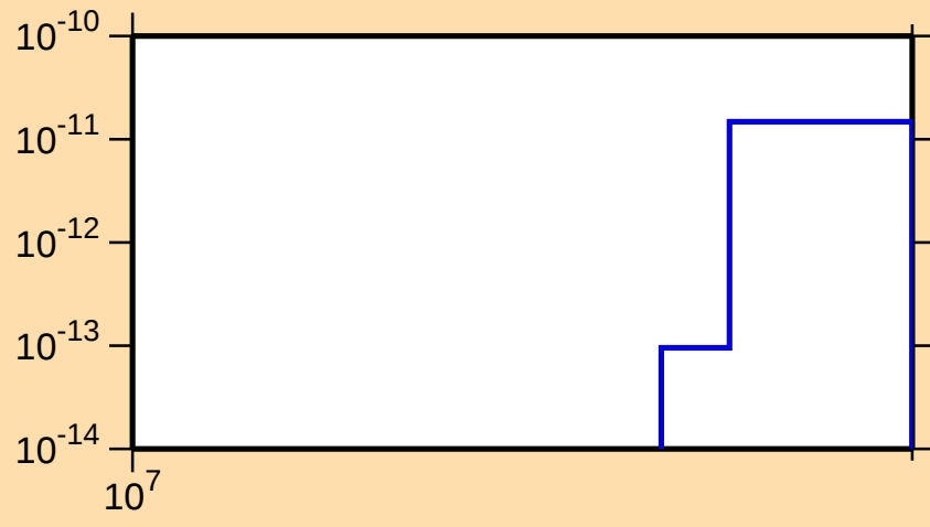
\sigma vs. E for ^{178}\text{Hf}(n,3n\alpha)
