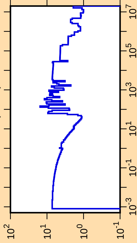
\Delta\sigma/\sigma vs. E for ^{178}\text{Hf}(n,\text{tot.})
