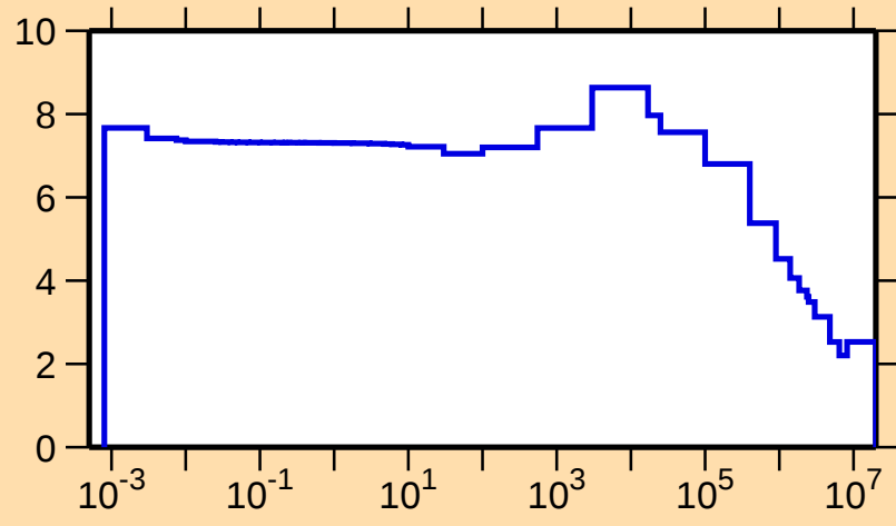
\sigma vs. E for ^{178}\text{Hf}(n,\text{el.})
