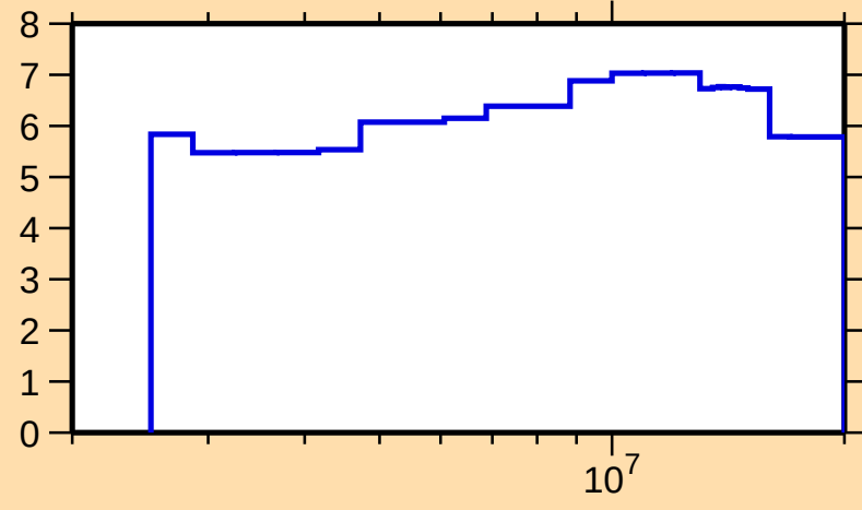
\Delta\sigma/\sigma vs. E for ^{179}\text{Hf}(n,n_1)
