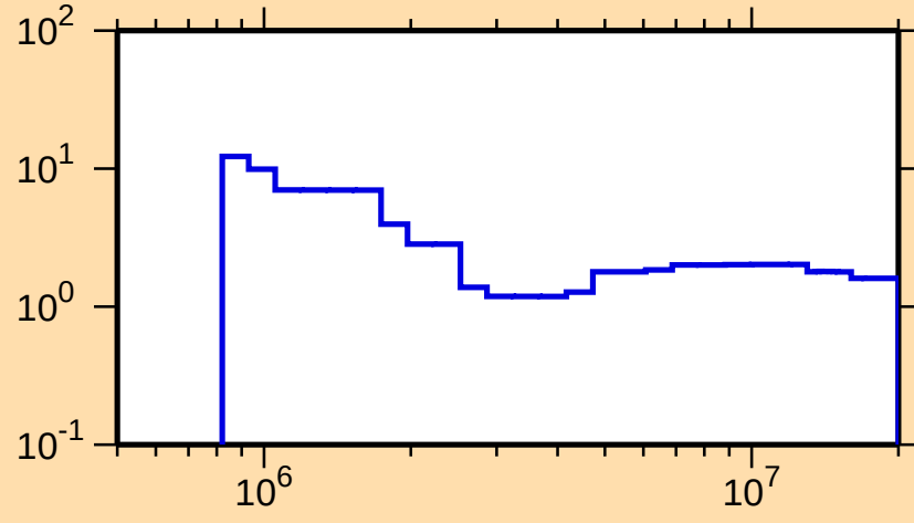
\Delta\sigma/\sigma vs. E for ^{179}\text{Hf}(n,n\text{oncl.})
