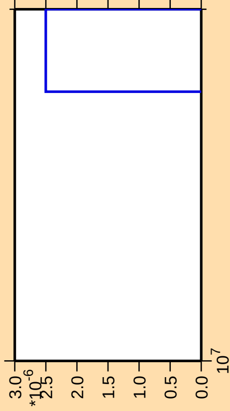
\Delta\sigma/\sigma vs. E for ^{183}\text{Hg} (mt 11)
