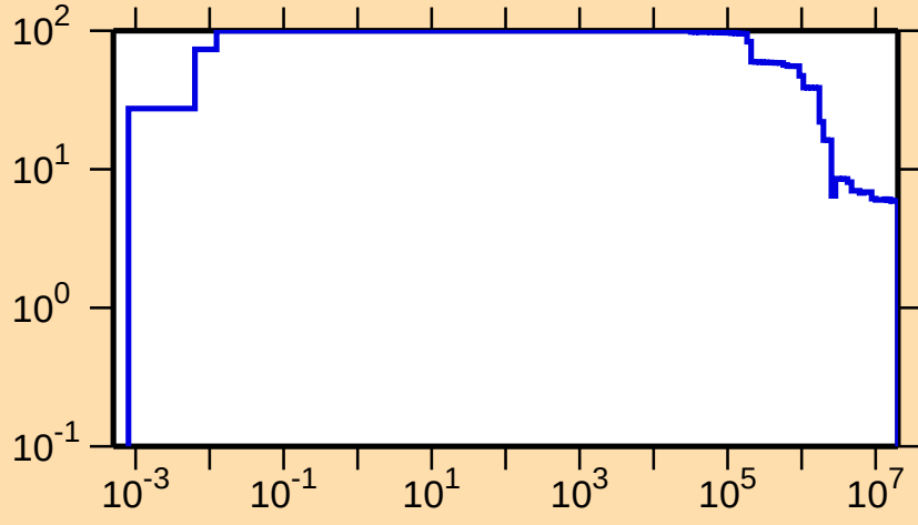
\Delta\sigma/\sigma vs. E for ^{183}\text{Hg}(n,\text{nonel.})
