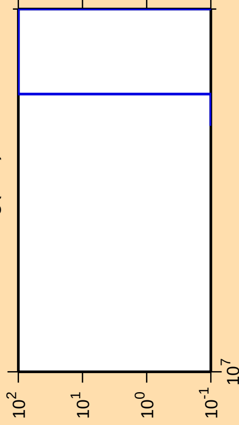
\Delta\sigma/\sigma vs. E for ^{183}\text{Hg}(n,\text{nt})
