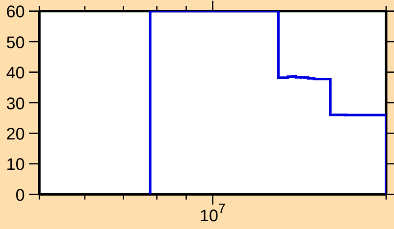
\Delta\sigma/\sigma vs. E for ^{183}\text{Hg}(n,2n)
