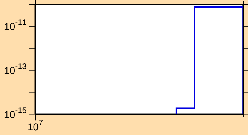
\sigma vs. E for ^{183}\text{Hg}(n,\text{nt})
