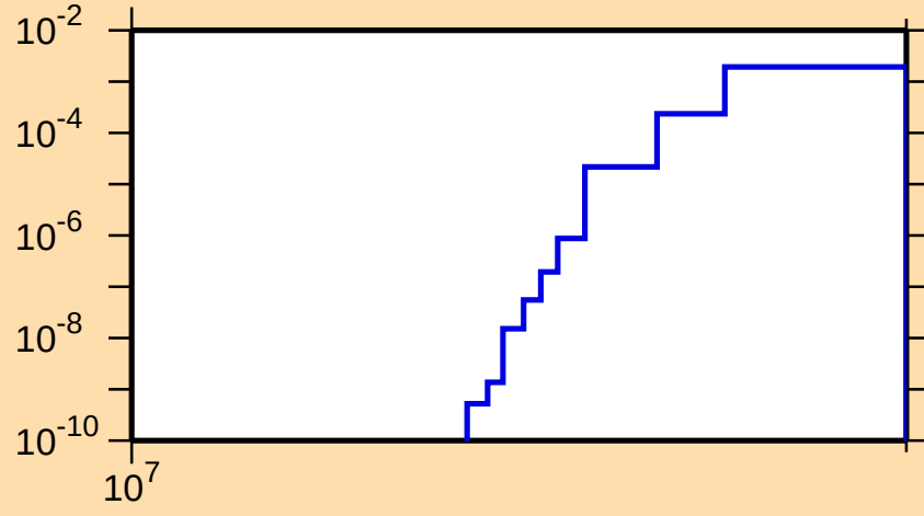
\sigma vs. E for ^{183}\text{Hg}(n,2np)
