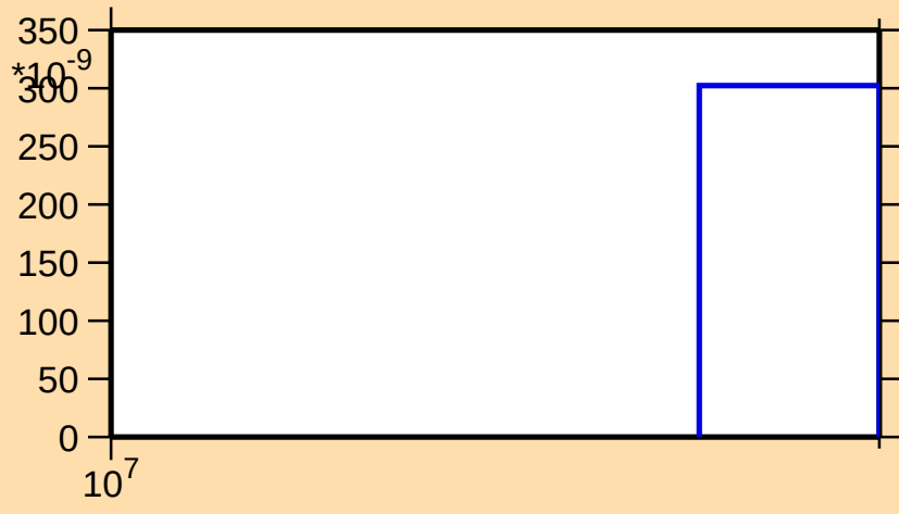
\sigma vs. E for ^{183}\text{Hg}(n,3n)
