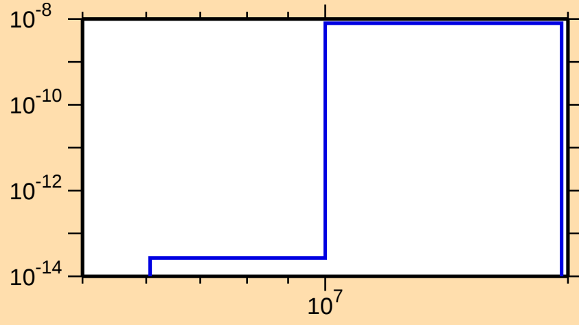
\sigma vs. E for ^{183}\text{Hg}(\text{mt117})
