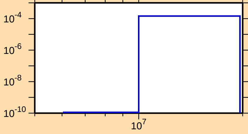
\sigma vs. E for ^{183}\text{Hg}(n,2n\alpha)
