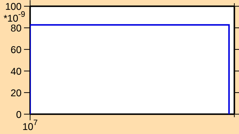
\sigma vs. E for ^{183}\text{Hg}(n,\text{nd})
