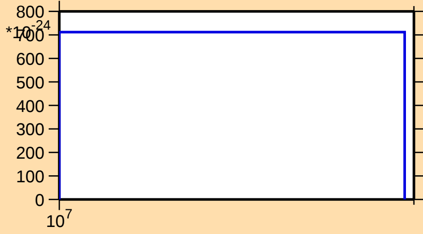
\sigma vs. E for ^{183}\text{Hg} (mt 11)
