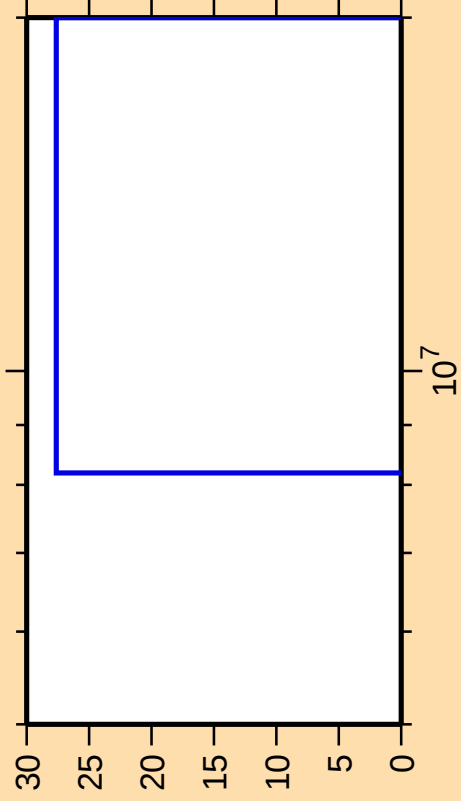
\Delta\sigma/\sigma vs. E for ^{183}\text{Hg}(n,n\text{cont.})
