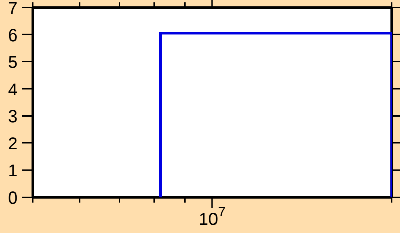
\Delta\sigma/\sigma vs. E for ^{183}\text{Hg}(n,\text{nonel.})
