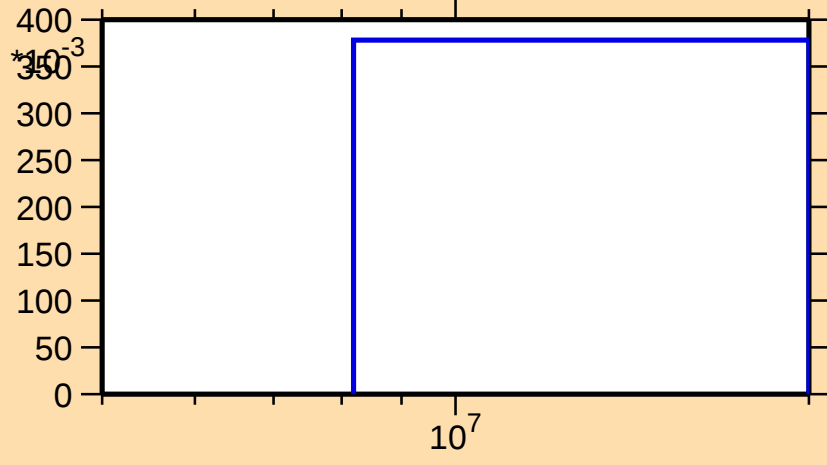
\sigma vs. E for ^{183}\text{Hg}(n,2n)
