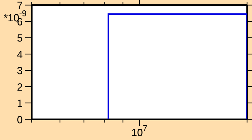
\sigma vs. E for ^{183}\text{Hg}(\text{mt117})
