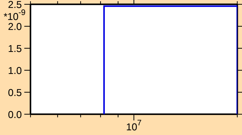
\sigma vs. E for ^{183}\text{Hg}(n,3n)
