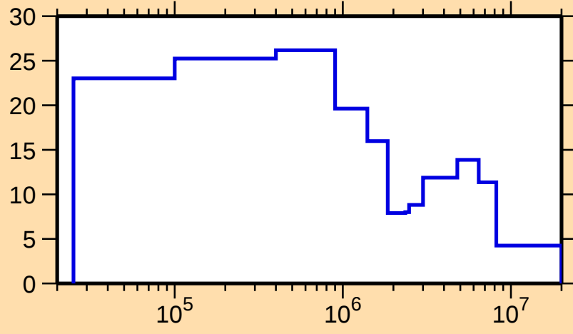
\Delta\sigma/\sigma vs. E for ^{183}\text{Hg}(n,\text{tot.})
