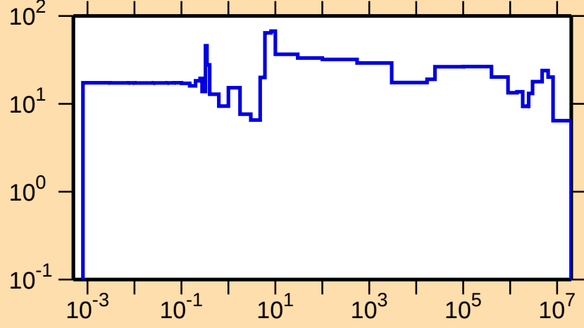
\Delta\sigma/\sigma vs. E for ^{183}\text{Hg}(n,\text{el.})
