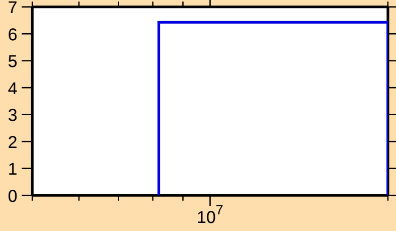
\Delta\sigma/\sigma vs. E for ^{183}\text{Hg}(n,\text{el.})
