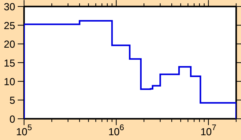
\Delta\sigma/\sigma vs. E for ^{183}\text{Hg}(n,\text{tot.})
