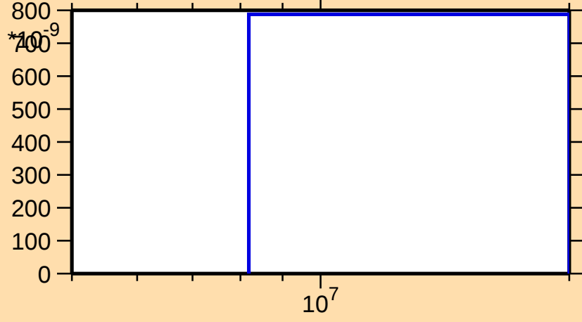
\sigma vs. E for ^{183}\text{Hg}(n,\text{pd})
