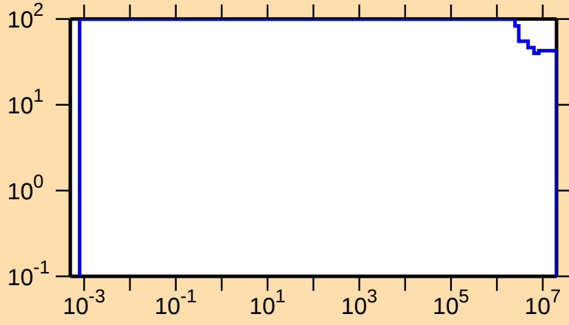
\Delta\sigma/\sigma vs. E for ^{183}\text{Hg}(n,p)
