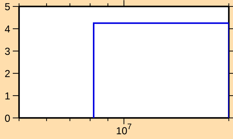
\Delta\sigma/\sigma vs. E for ^{183}\text{Hg}(n,\text{tot.})
