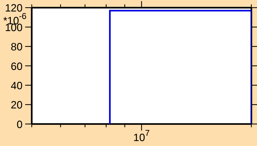
\sigma vs. E for ^{183}\text{Hg}(n,2n\alpha)
