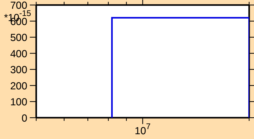
\sigma vs. E for ^{183}\text{Hg}(n,nt)
