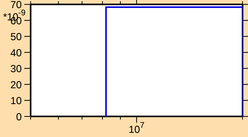
\sigma vs. E for ^{183}\text{Hg}(n,\text{nd})
