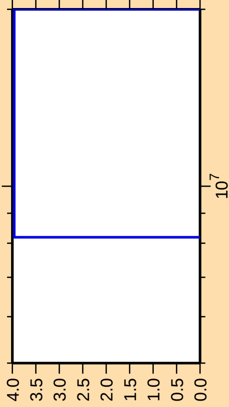
\Delta\sigma/\sigma vs. E for ^{183}\text{Hg}(n,nt)
