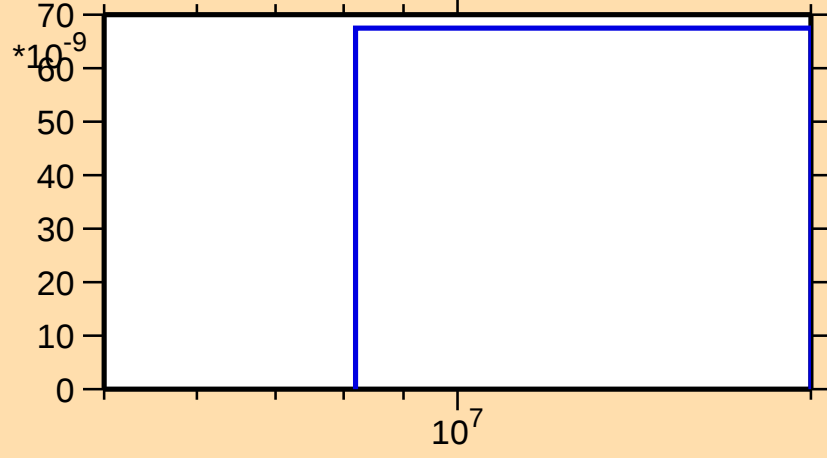
\sigma vs. E for ^{183}\text{Hg}(n,\text{pt})
