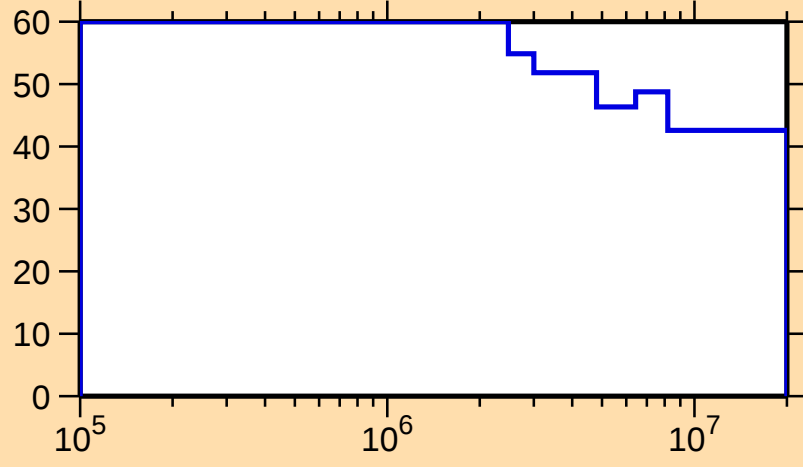
\Delta\sigma/\sigma vs. E for ^{183}\text{Hg}(n,n_1)
