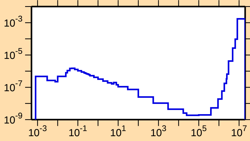
\sigma vs. E for ^{183}\text{Hg}(n,p\alpha)
