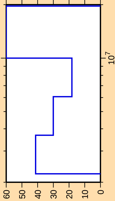
\Delta\sigma/\sigma vs. E for ^{190}\text{Hg}(n,n\text{cont.})
