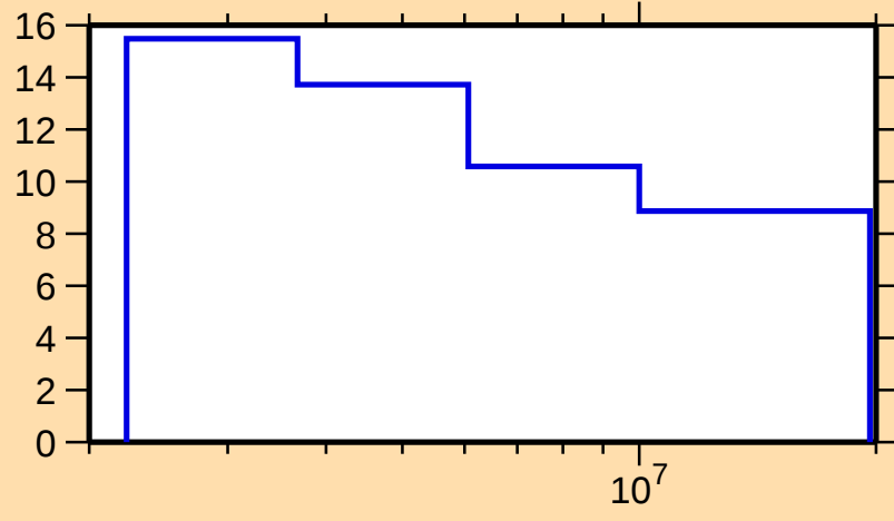
\Delta\sigma/\sigma vs. E for ^{190}\text{Hg}(n,n\text{onel.})
