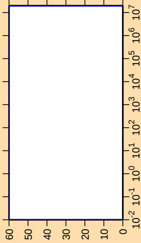
\Delta\sigma/\sigma vs. E for ^{190}\text{Hg}(n,\alpha)
