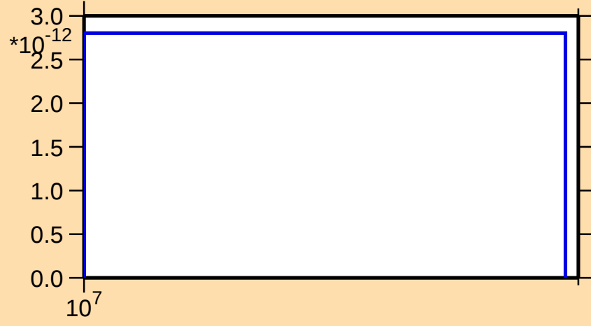
\sigma vs. E for ^{190}\text{Hg}(n,\text{pd})
