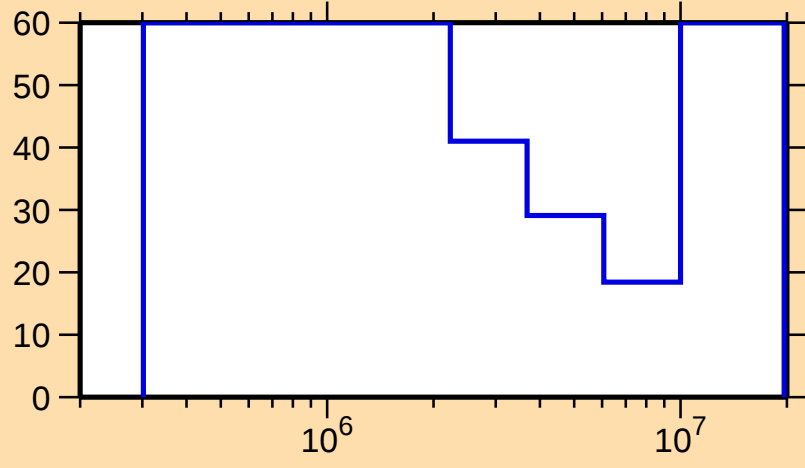
\Delta\sigma/\sigma vs. E for ^{190}\text{Hg}(n,\text{inel.})
