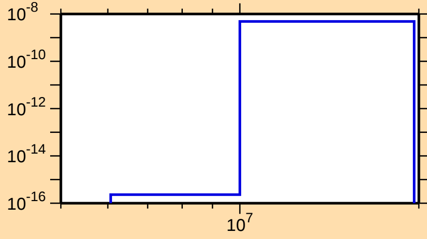
\sigma vs. E for ^{190}\text{Hg}(n,\text{He}3)
