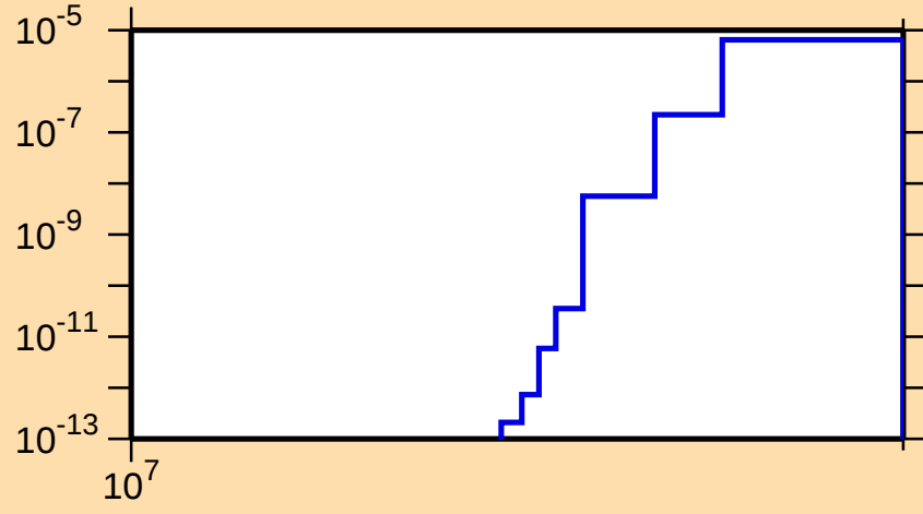
\sigma vs. E for ^{191}\text{Hg}(n,2np)
