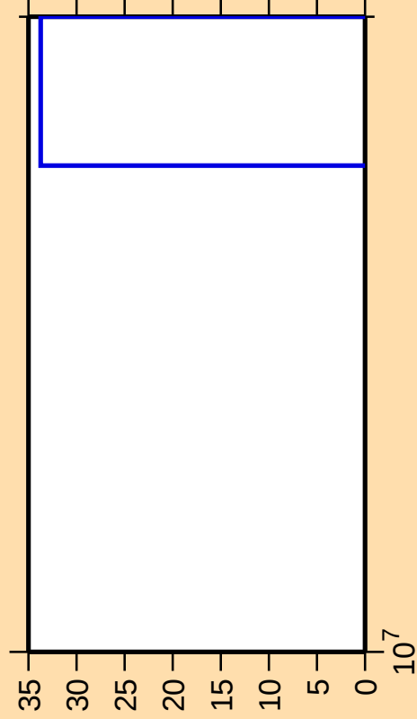
\Delta\sigma/\sigma vs. E for ^{191}\text{Hg} (mt 34)
