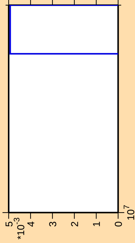
\Delta\sigma/\sigma vs. E for ^{191}\text{Hg}(n,3n\alpha)
