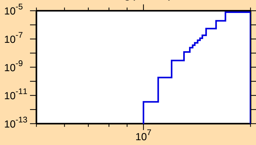
\sigma vs. E for ^{191}\text{Hg}(n,2n\alpha)
