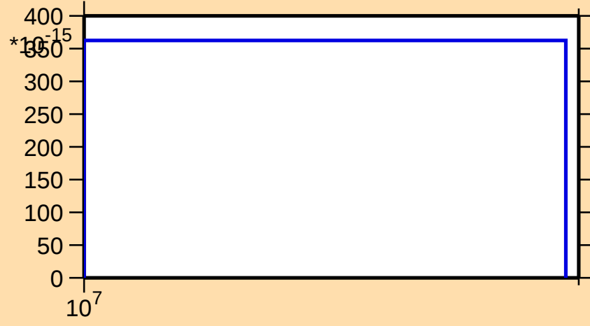
\sigma vs. E for ^{191}\text{Hg}(n,\text{nt})
