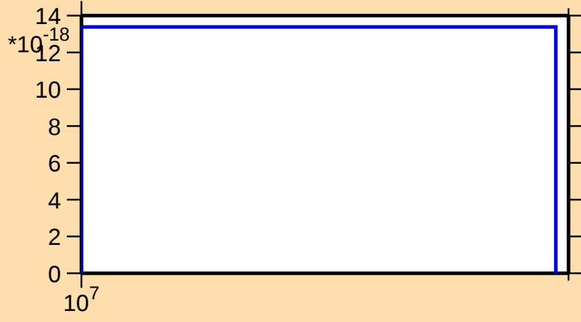
\sigma vs. E for ^{191}\text{Hg}(n,3n\alpha)
