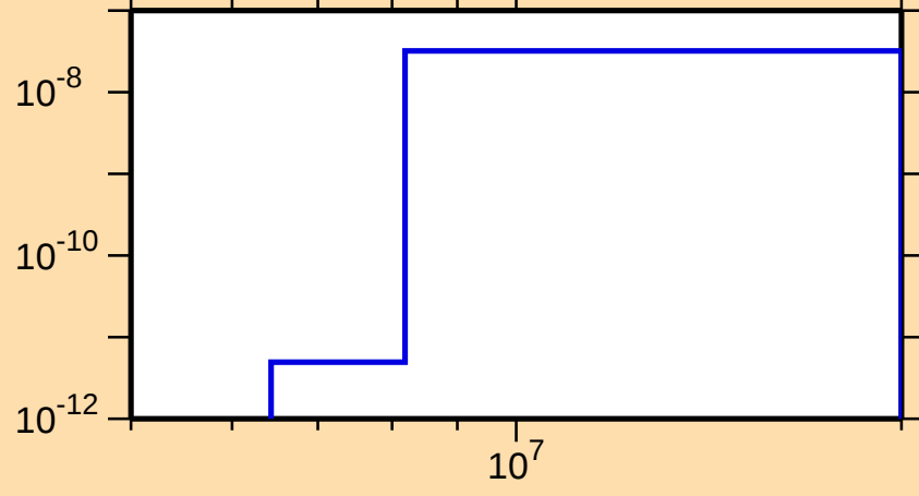
\sigma vs. E for ^{191}\text{Hg}(n,p\alpha)
