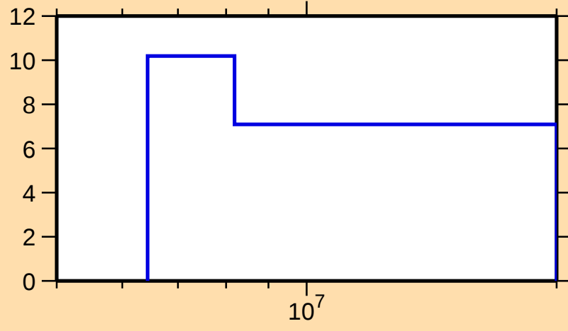
\Delta\sigma/\sigma vs. E for ^{191}\text{Hg}(n,\text{nonel.})
