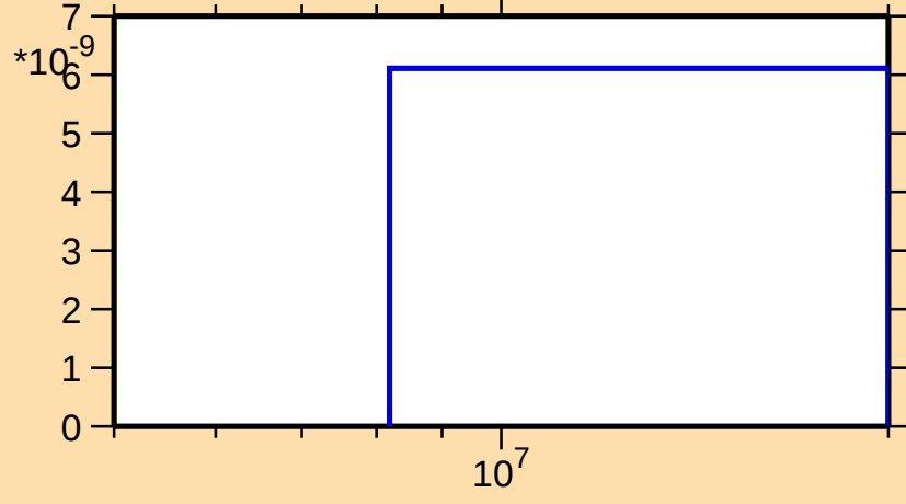
\sigma vs. E for ^{191}\text{Hg}(n,\text{nd})
