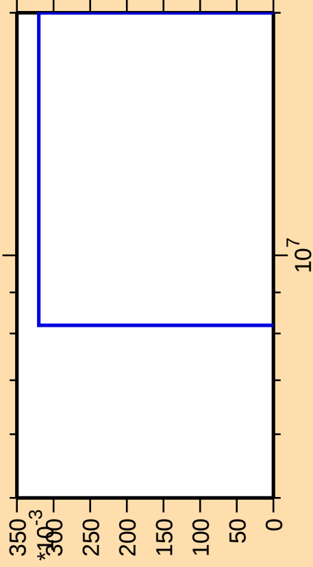
\Delta\sigma/\sigma vs. E for ^{191}\text{Hg}(\text{mt117})
