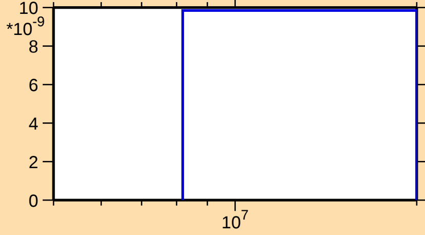
\sigma vs. E for ^{191}\text{Hg}(n,\text{He}3)
