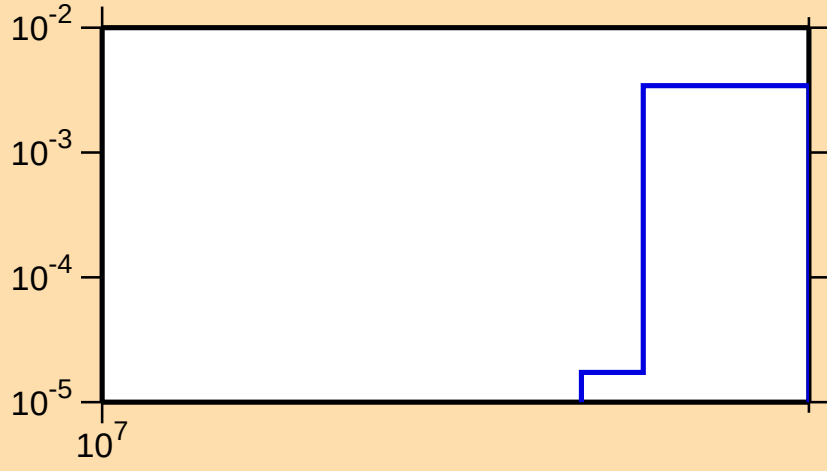
\sigma vs. E for ^{193}\text{Hg}(n,3n)
