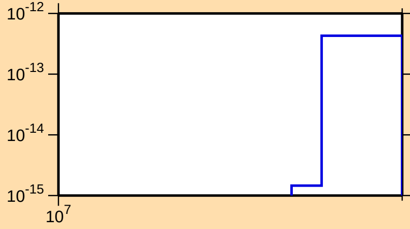
\sigma vs. E for ^{193}\text{Hg} (mt 34)
