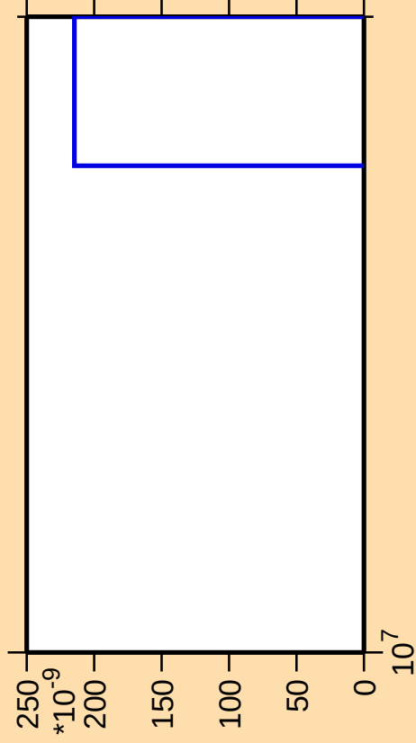
\Delta\sigma/\sigma vs. E for ^{193}\text{Hg} (mt 11)
