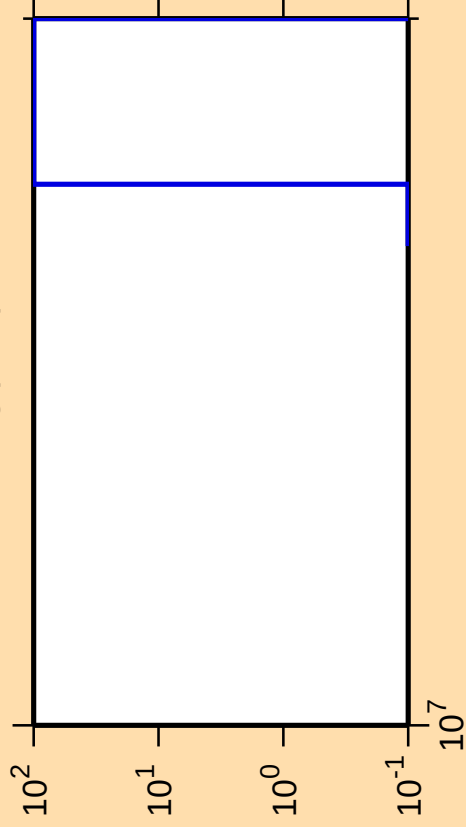
\Delta\sigma/\sigma vs. E for ^{193}\text{Hg}(n,\text{nt})
