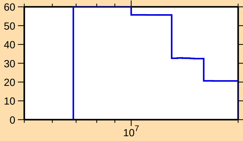
\Delta\sigma/\sigma vs. E for ^{193}\text{Hg}(n,2n)
