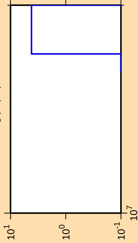
\Delta\sigma/\sigma vs. E for ^{193}\text{Hg}(n,\text{pd})
