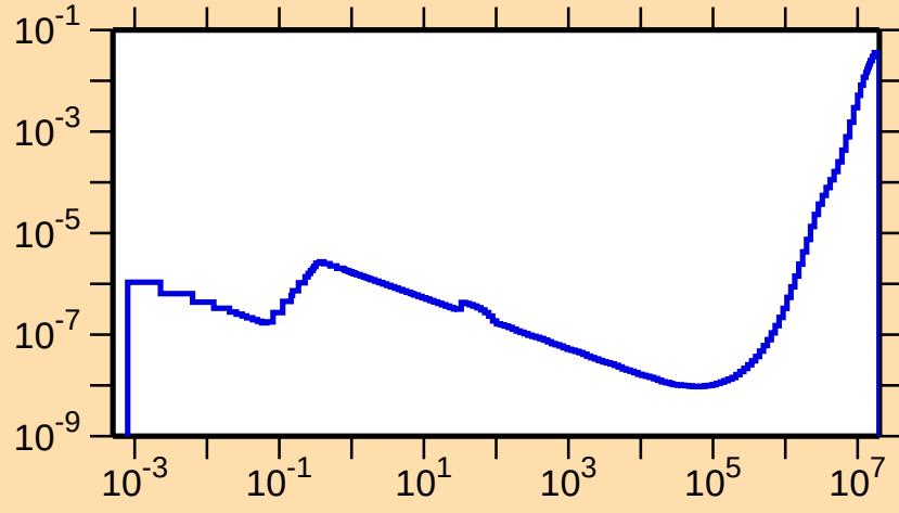
\sigma vs. E for ^{193}\text{Hg}(n,p)
