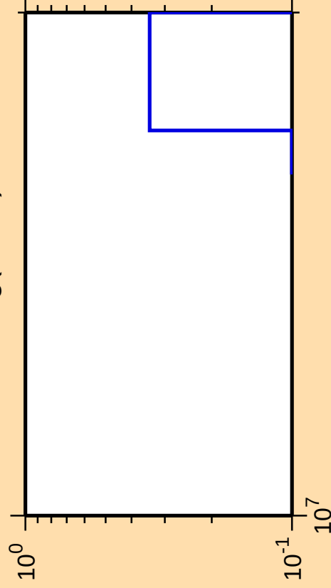
\Delta\sigma/\sigma vs. E for ^{193}\text{Hg} (mt 45)
