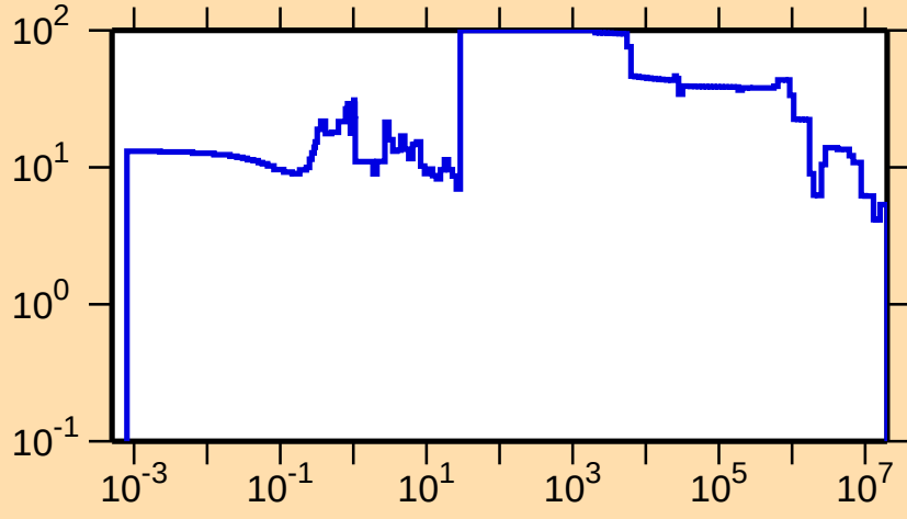
\Delta\sigma/\sigma vs. E for ^{193}\text{Hg}(n,\text{tot.})
