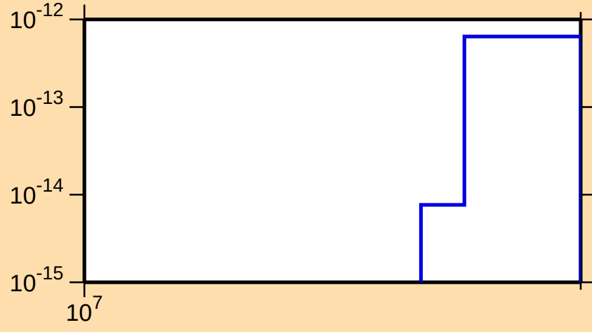
\sigma vs. E for ^{193}\text{Hg}(n,\text{pd})
