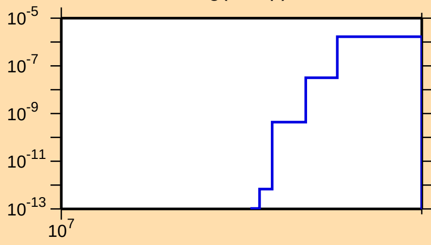
\sigma vs. E for ^{193}\text{Hg}(n,2np)
