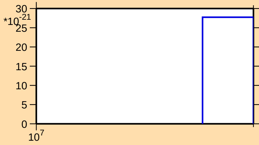
\sigma vs. E for ^{193}\text{Hg} (mt 11)
