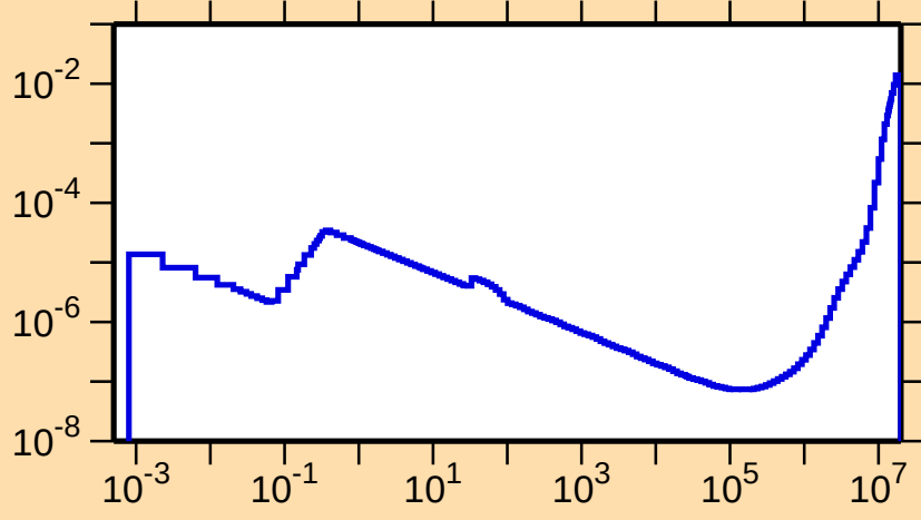
\sigma vs. E for ^{193}\text{Hg}(n,\alpha)
