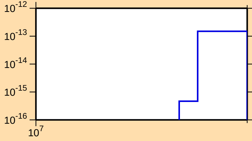
\sigma vs. E for ^{193}\text{Hg}(n,\text{pt})
