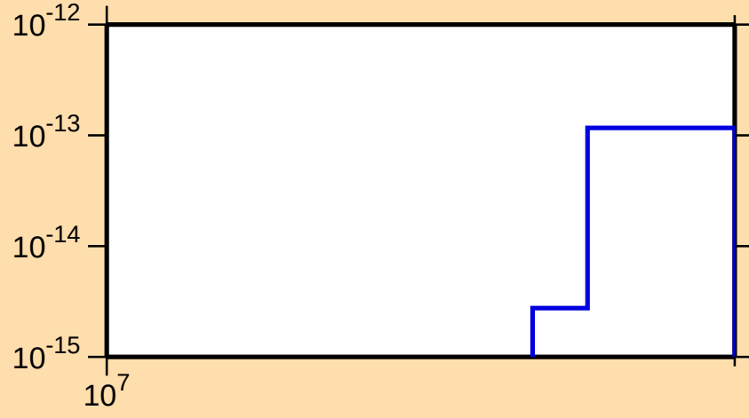
\sigma vs. E for ^{193}\text{Hg} (mt 45)
