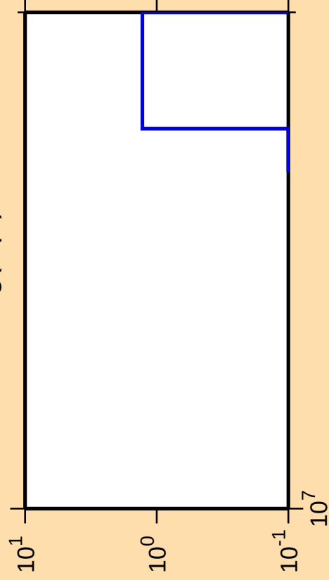
\Delta\sigma/\sigma vs. E for ^{193}\text{Hg}(n,\text{pt})
