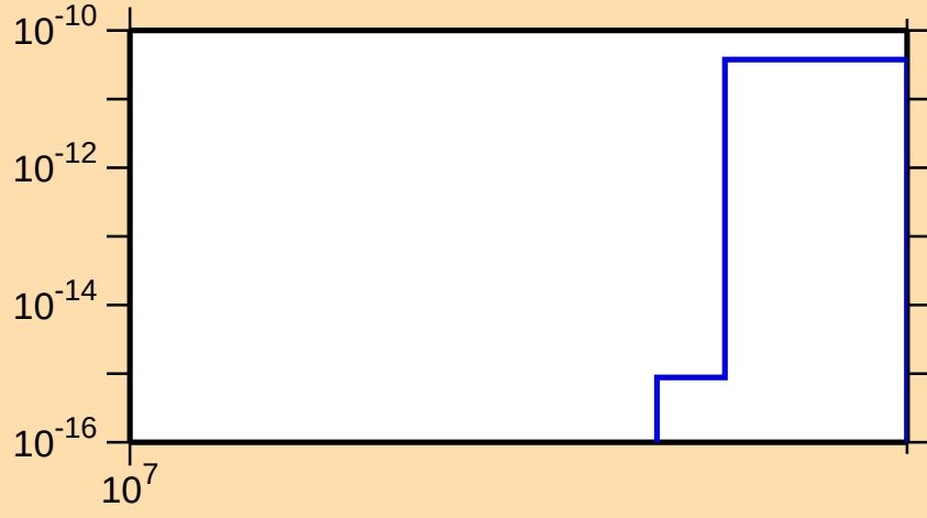
\sigma vs. E for ^{193}\text{Hg}(n,\text{nt})
