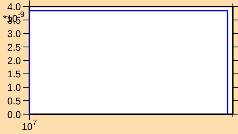
\sigma vs. E for ^{193}\text{Hg}(n,\text{nd})
