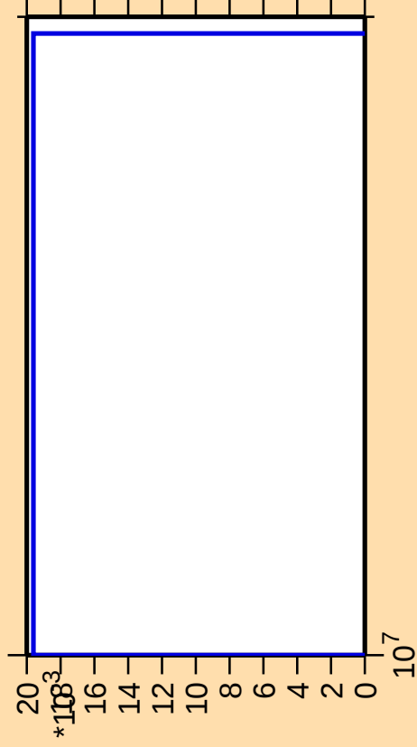
\Delta\sigma/\sigma vs. E for ^{193}\text{Hg} (mt 34)
