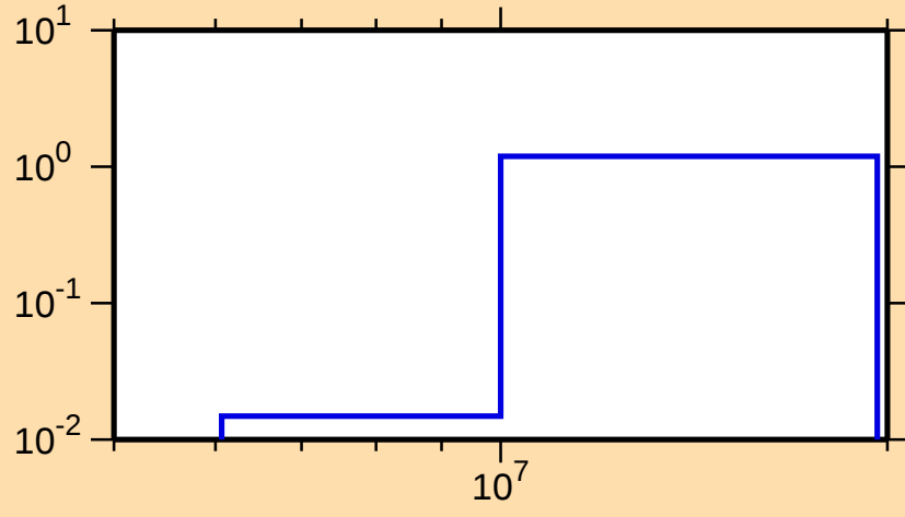
\sigma vs. E for ^{193}\text{Hg}(n,2n)
