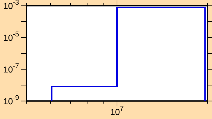
\sigma vs. E for ^{193}\text{Hg}(n,d)
