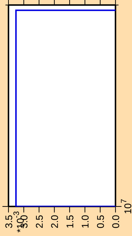
\Delta\sigma/\sigma vs. E for ^{193}\text{Hg} (mt 45)
