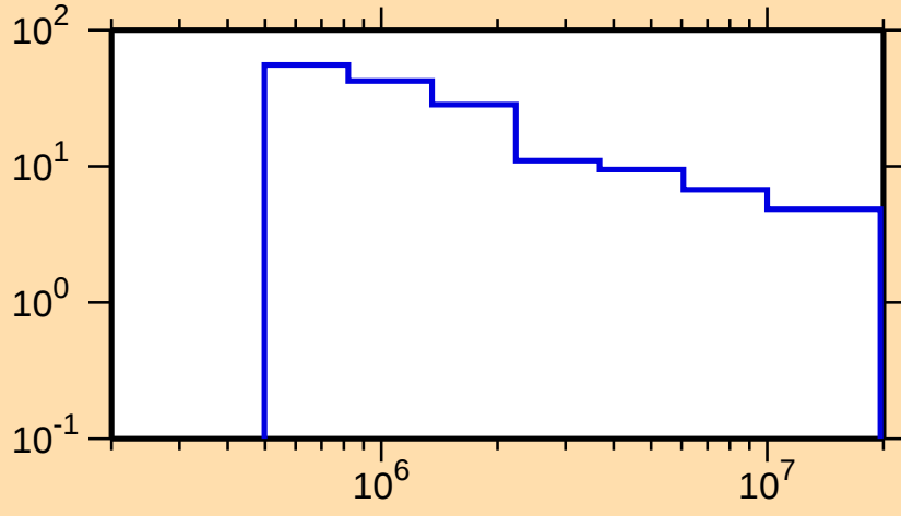
\Delta\sigma/\sigma vs. E for ^{193}\text{Hg}(n,n\text{onel.})
