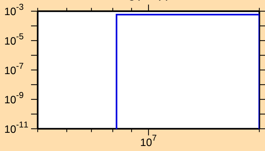
\sigma vs. E for ^{193}\text{Hg}(n,np)
