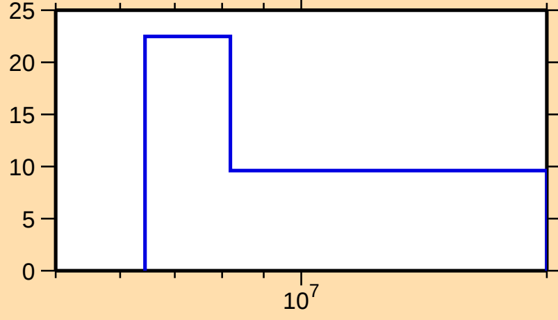
\Delta\sigma/\sigma vs. E for ^{193}\text{Hg}(n,\text{el.})
