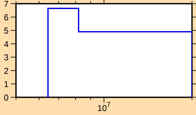
\Delta\sigma/\sigma vs. E for ^{193}\text{Hg}(n,\text{nonel.})
