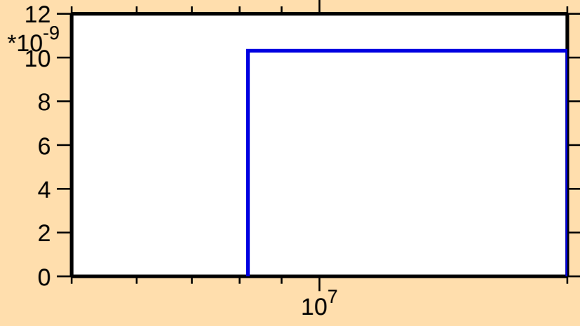
\sigma vs. E for ^{193}\text{Hg}(n,2n\alpha)
