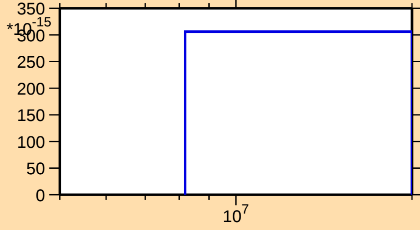
\sigma vs. E for ^{193}\text{Hg}(n,nt)
