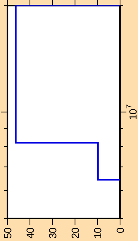
\Delta\sigma/\sigma vs. E for ^{193}\text{Hg}(n,n\text{cont.})
