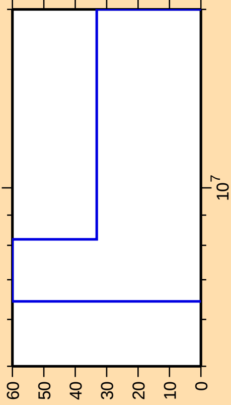
\Delta\sigma/\sigma vs. E for ^{193}\text{Hg}(n,2n)
