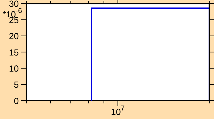
\sigma vs. E for ^{193}\text{Hg}(n,3n)
