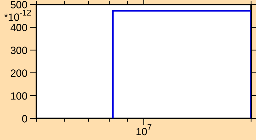
\sigma vs. E for ^{193}\text{Hg}(n,p\alpha)
