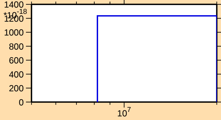
\sigma vs. E for ^{193}\text{Hg}(n,\text{pt})
