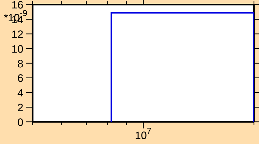
\sigma vs. E for ^{193}\text{Hg}(n,2np)
