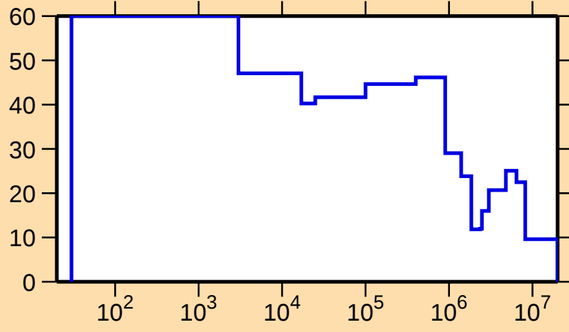
\Delta\sigma/\sigma vs. E for ^{193}\text{Hg}(n,\text{el.})
