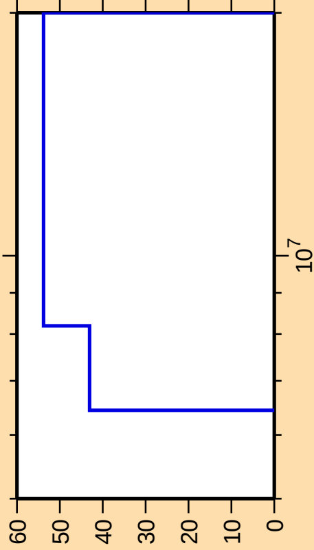
\Delta\sigma/\sigma vs. E for ^{193}\text{Hg}(n,n_1)
