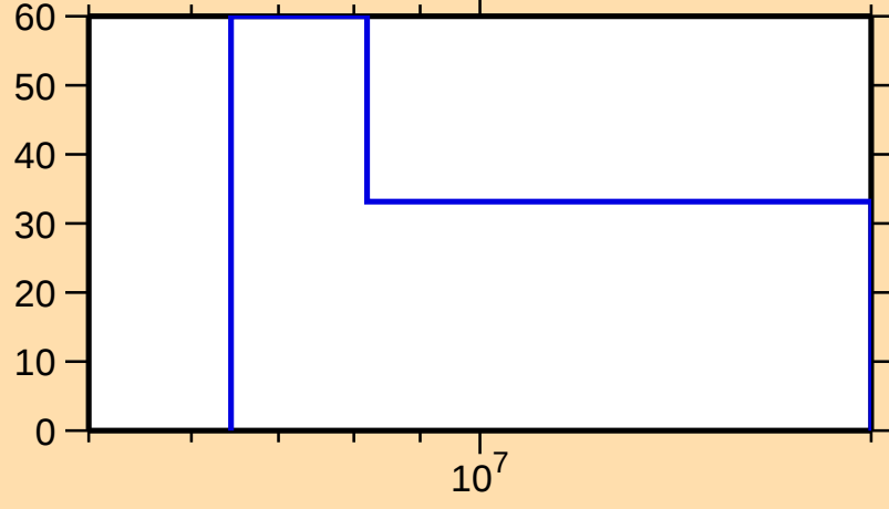
\Delta\sigma/\sigma vs. E for ^{193}\text{Hg}(n,2n)
