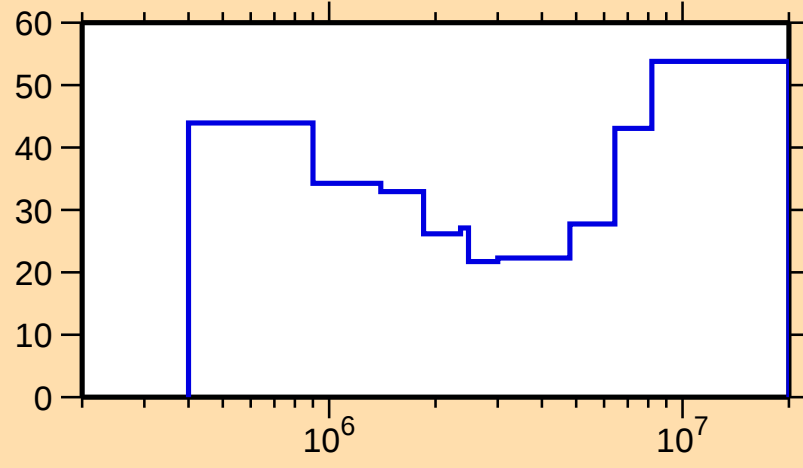
\Delta\sigma/\sigma vs. E for ^{193}\text{Hg}(n,n_1)
