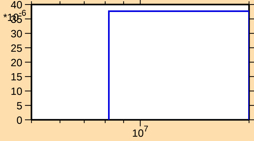
\sigma vs. E for ^{193}\text{Hg}(n,t)
