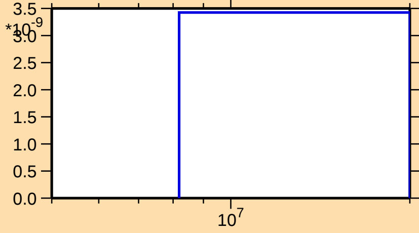
\sigma vs. E for ^{193}\text{Hg}(n,\text{nd})
