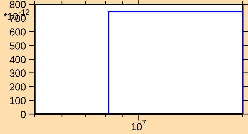
\sigma vs. E for ^{193}\text{Hg}(n,\text{He}3)
