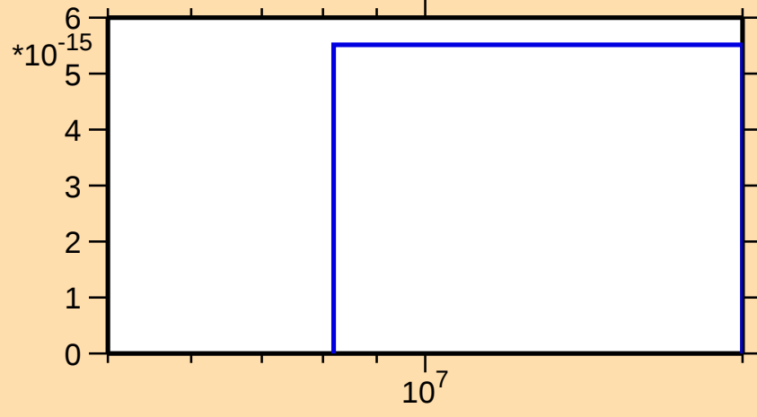
\sigma vs. E for ^{193}\text{Hg}(n,\text{pd})
