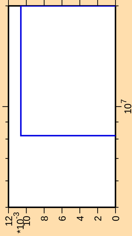
\Delta\sigma/\sigma vs. E for ^{193}\text{Hg}(n,\text{pt})
