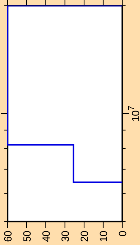
\Delta\sigma/\sigma vs. E for ^{193}\text{Hg}(n,np)
