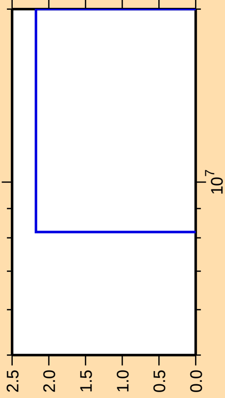
\Delta\sigma/\sigma vs. E for ^{193}\text{Hg}(n,nt)
