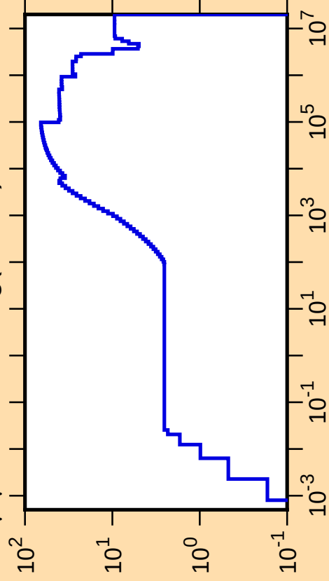
\Delta\mu/\mu vs. E for ^{194}\text{Hg}(\text{mt251})
