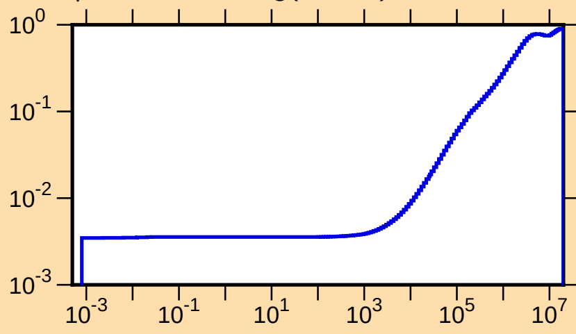
\mu vs. E for ^{194}\text{Hg}(\text{mt251})
