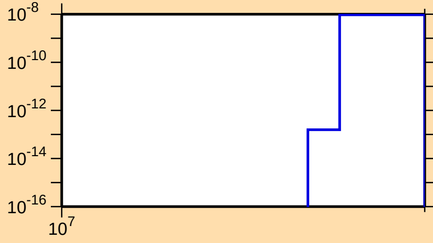
\sigma vs. E for ^{194}\text{Hg}(n,2np)
