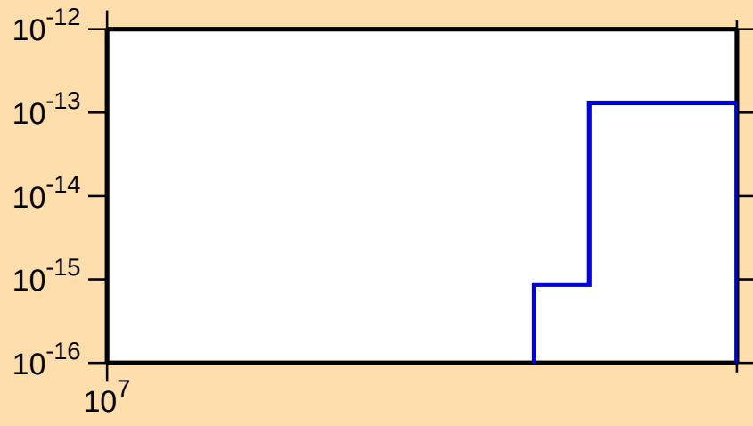
\sigma vs. E for ^{194}\text{Hg}(n,\text{pd})
