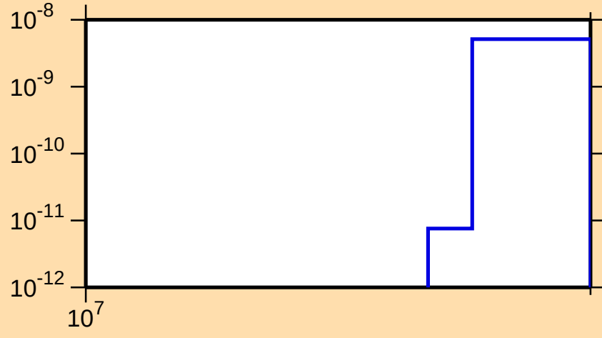
\sigma vs. E for ^{194}\text{Hg}(n,\text{nd})
