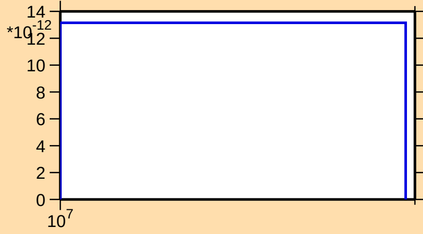
\sigma vs. E for ^{194}\text{Hg}(n,p\alpha)
