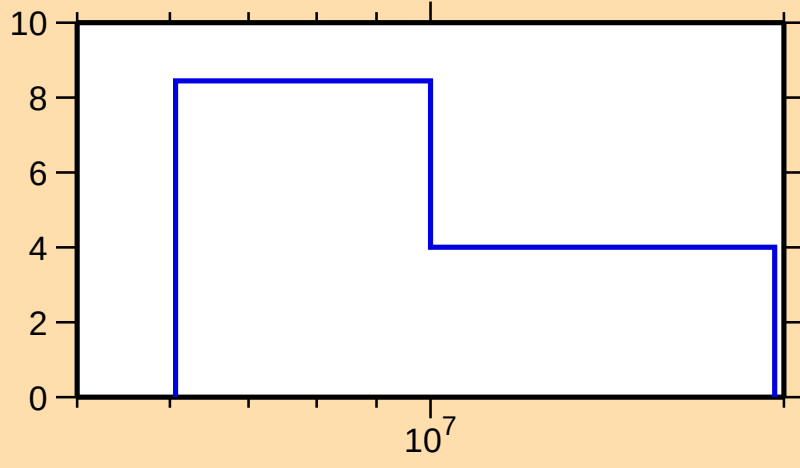
\Delta\sigma/\sigma vs. E for ^{194}\text{Hg}(n,\text{tot.})
