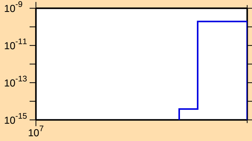
\sigma vs. E for ^{195}\text{Hg}(n,\text{nt})
