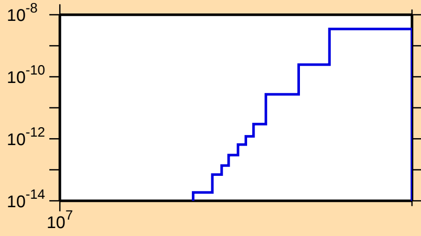
\sigma vs. E for ^{195}\text{Hg}(n,\text{He3})
