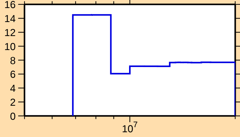
\Delta\sigma/\sigma vs. E for ^{195}\text{Hg}(n,\text{el.})
