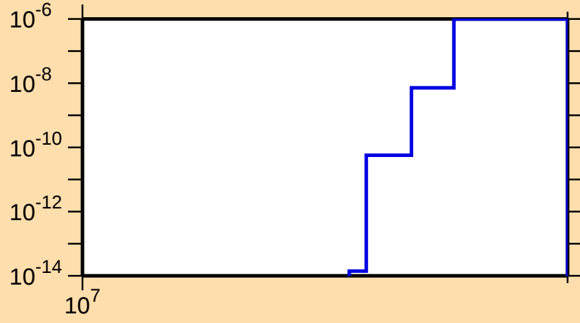
\sigma vs. E for ^{195}\text{Hg}(n,2np)
