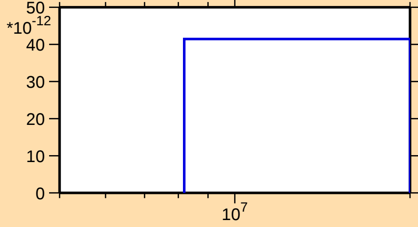
\sigma vs. E for ^{195}\text{Hg}(n,\text{He}3)
