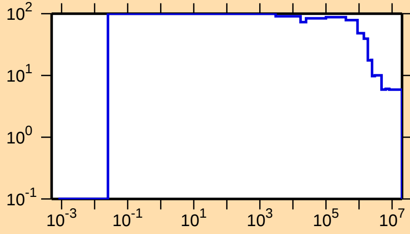
\Delta\sigma/\sigma vs. E for ^{195}\text{Hg}(n,\text{nonel.})
