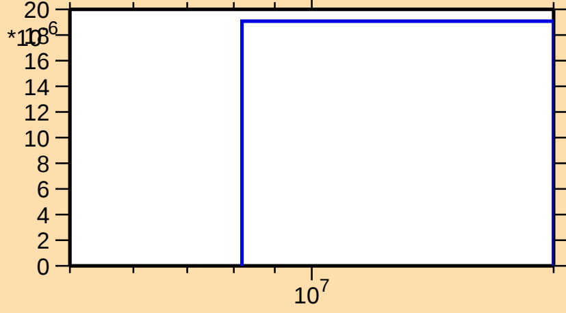
\sigma vs. E for ^{195}\text{Hg}(n,t)
