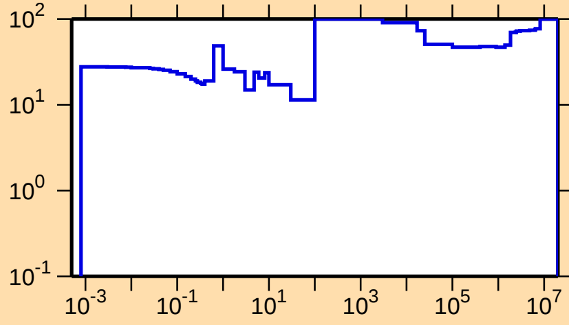
\Delta\sigma/\sigma vs. E for ^{195}\text{Hg}(n,\gamma)
