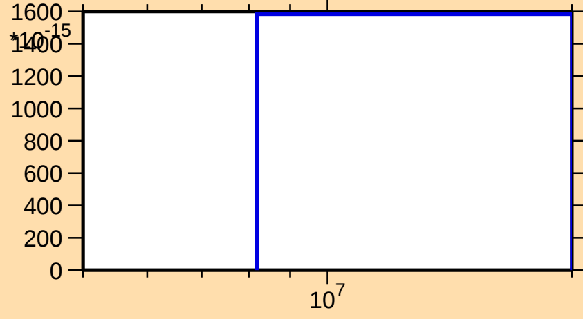
\sigma vs. E for ^{195}\text{Hg}(n,nt)
