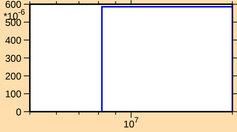
\sigma vs. E for ^{195}\text{Hg}(n,3n)
