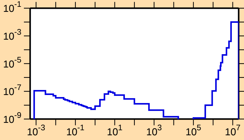
\sigma vs. E for ^{195}\text{Hg}(n,p)
