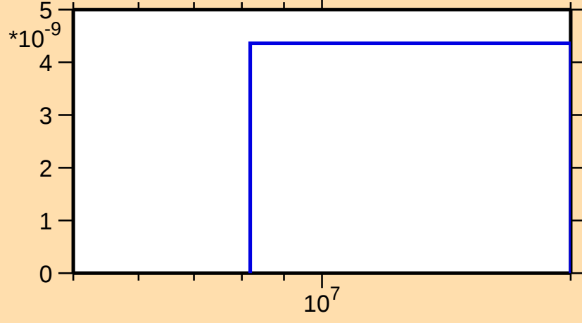
\sigma vs. E for ^{195}\text{Hg}(n,\text{nd})
