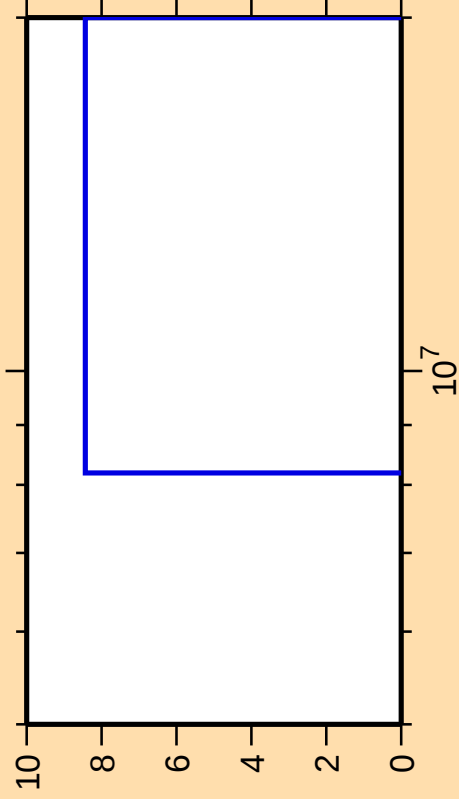
\Delta\sigma/\sigma vs. E for ^{195}\text{Hg}(n,nt)
