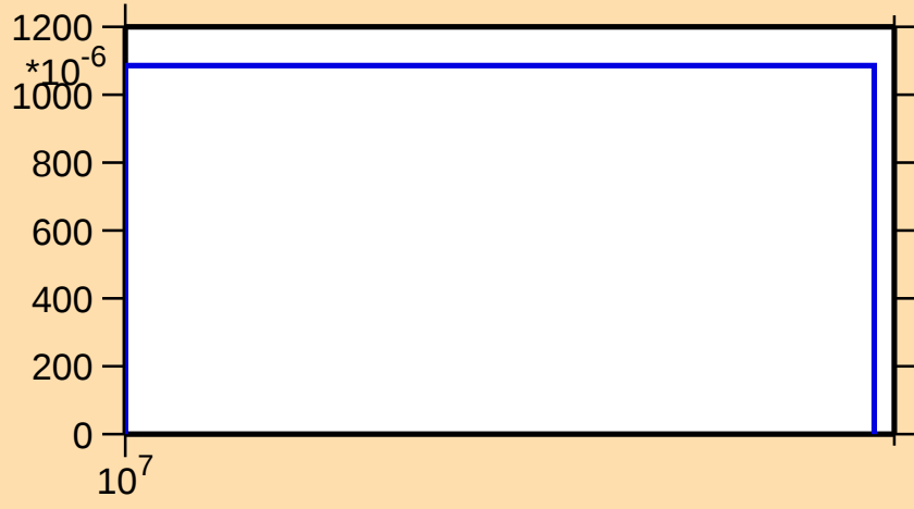
\sigma vs. E for ^{197}\text{Hg}(n,3n)
