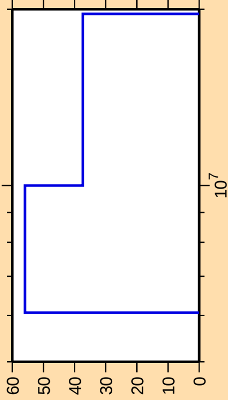
\Delta\sigma/\sigma vs. E for ^{197}\text{Hg}(n,\gamma)
