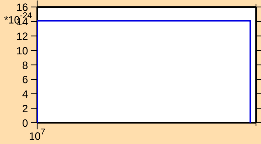
\sigma vs. E for ^{197}\text{Hg} (mt 11)
