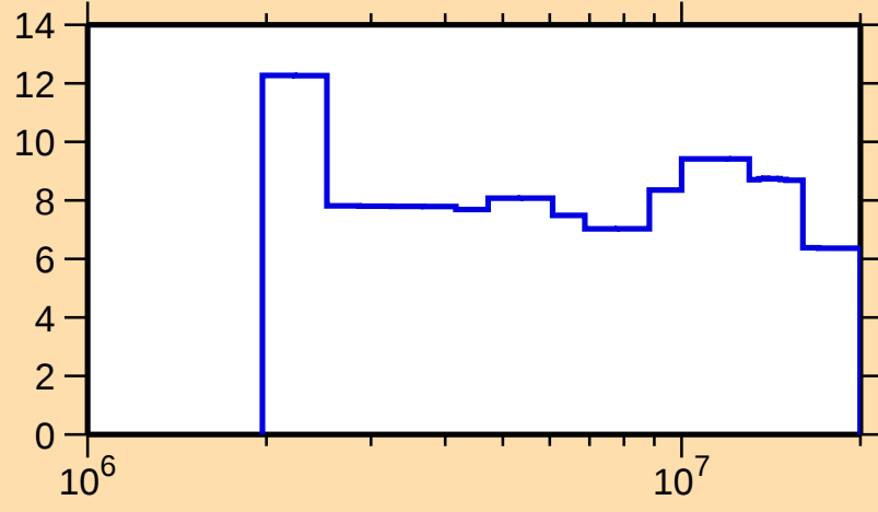
\Delta\sigma/\sigma vs. E for ^{202}\text{Hg}(n,\text{el.})
