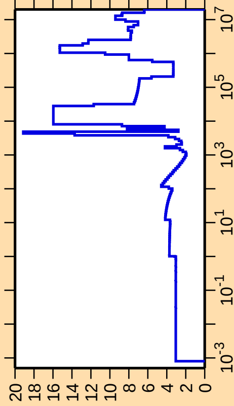
\Delta\sigma/\sigma vs. E for ^{202}\text{Hg}(n,\text{el.})
