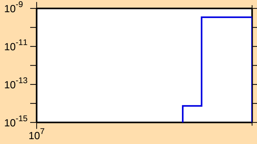
\sigma vs. E for ^{202}\text{Hg}(n,\text{nt})
