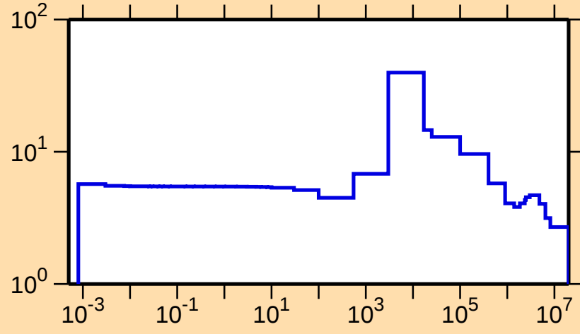
\sigma vs. E for ^{202}\text{Hg}(n,\text{el.})
