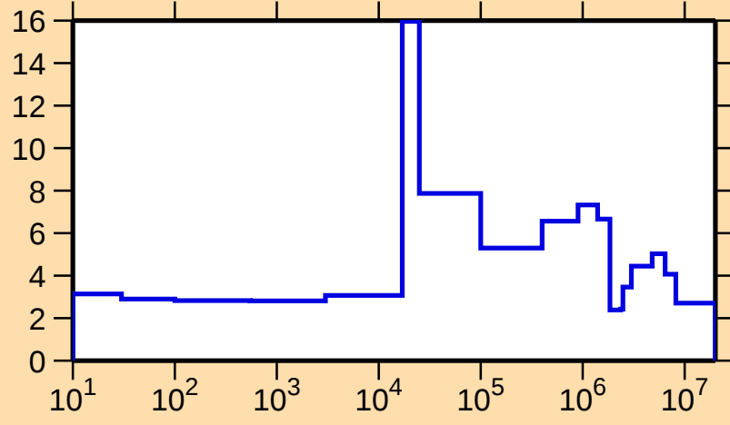
\Delta\sigma/\sigma vs. E for ^{202}\text{Hg}(n,\text{tot.})
