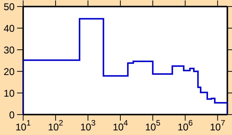
\Delta\sigma/\sigma vs. E for ^{202}\text{Hg}(n,\text{nonel.})
