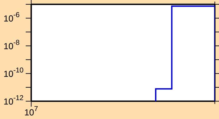
\sigma vs. E for ^{203}\text{Hg}(n,2n\alpha)
