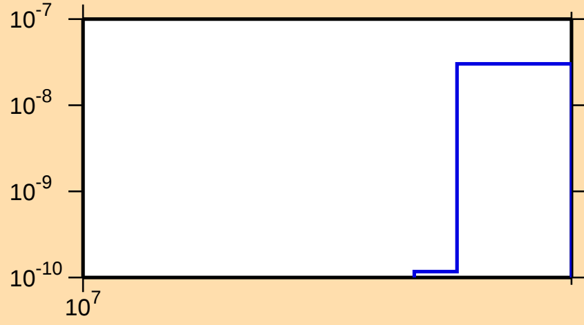
\sigma vs. E for ^{203}\text{Hg}(n,\text{nd})
