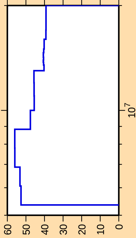
\Delta\sigma/\sigma vs. E for ^{203}\text{Hg}(n,n_1)
