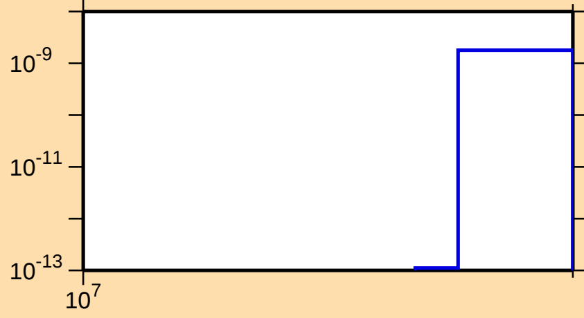
\sigma vs. E for ^{203}\text{Hg}(n,2np)
