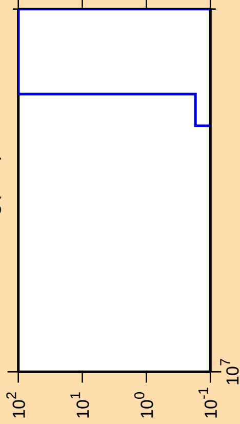
\Delta\sigma/\sigma vs. E for ^{203}\text{Hg}(n,\text{nt})
