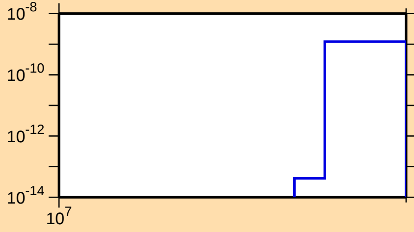
\sigma vs. E for ^{203}\text{Hg}(n,\text{nt})
