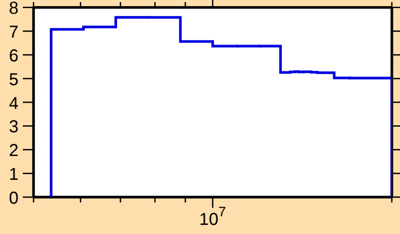
\Delta\sigma/\sigma vs. E for ^{203}\text{Hg}(n,\text{nonel.})
