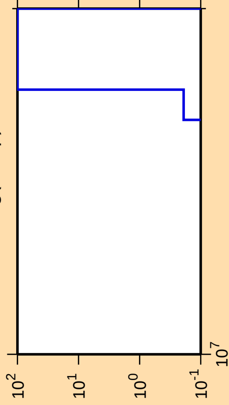
\Delta\sigma/\sigma vs. E for ^{203}\text{Hg}(n,2np)
