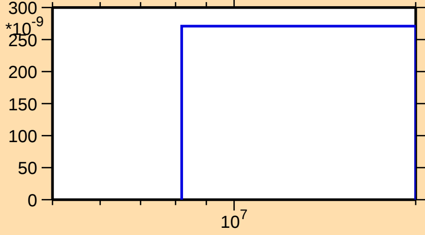
\sigma vs. E for ^{203}\text{Hg}(n,n\alpha)
