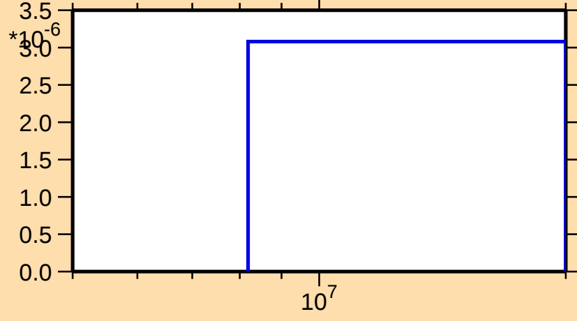
\sigma vs. E for ^{203}\text{Hg}(n,t)
