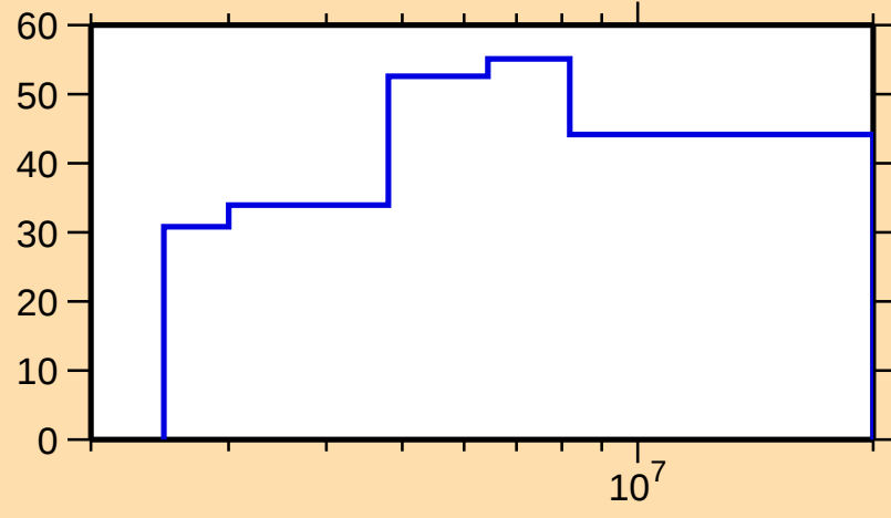
\Delta\sigma/\sigma vs. E for ^{203}\text{Hg}(n,n_1)
