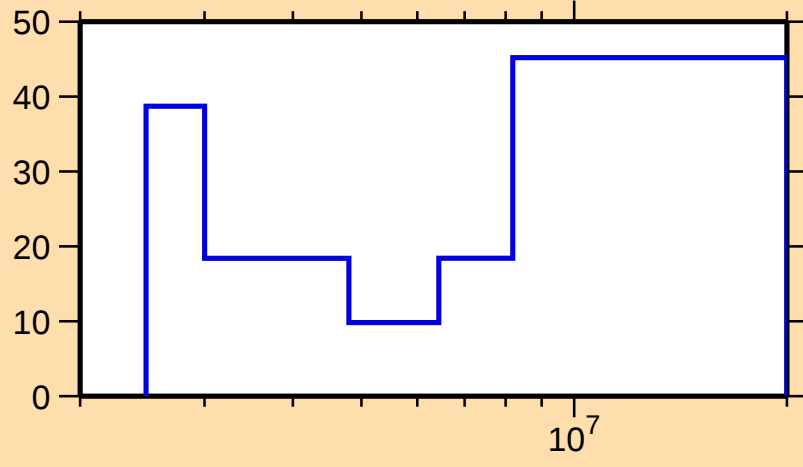
\Delta\sigma/\sigma vs. E for ^{203}\text{Hg}(n,n\text{cont.})
